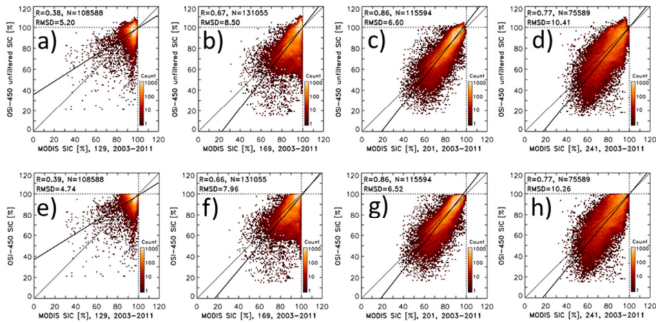
Figure 14. Illustration of the impact using the non-truncated (top row, panel a) to d) instead of the truncated (bottom row, panel e) to h) SIC data, for example OSI-450 (representative of group I products), when comparing PMW SIC with MODIS SIC. Shown are the two-dimensional histograms for all four 8-day periods starting at DOY 129, 169, 201, and 241 of the years 2003 through 2011 (see Fig. S1). The quantities given in the top left corner are R: linear correlation coefficient, N: number of valid data pairs, and RMSD: root mean squared difference. The thin black line is the identity line; the thick black line denotes the linear regression through the data pairs.
