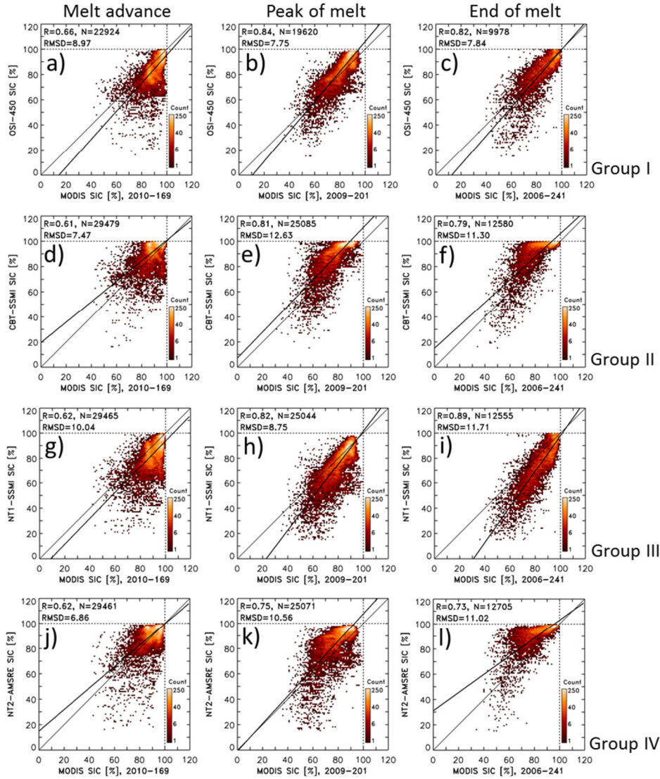
Figure 56. Two-dimensional histograms of the distribution of PMW (y-axis) versus MODIS (x-axis) SIC data pairs using a bin size of 1 % for the same 8-day periods as shown in Fig. 54e-p, i.e. melt advance, peak melt, and end of melt. The topmost row shows OSI-450 (for group I), the second row CBT-SSMI (for group II), the third row NT1-SSMI (for group III), and the bottommost row NT2-AMSRE (group IV). The thin black line is the identity line. The thick black line denotes the linear regression through the data pairs. At the top left of every image we display the linear correlation coefficient R , the number of data pairs N and the root mean squared difference RMSD; the latter is given in percent. The leftmost, middle and rightmost columns are representing melt advance, peak of melt, and end of the melt, respectively. Respective scatterplots for pre-melt are shown in Figure S06 in the supplementary material 2 .
