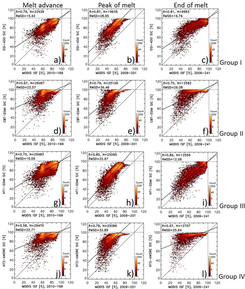
Figure 89. Two-dimensional histograms of the distribution of PMW SIC (y-axis) versus MODIS ISF (x-axis) data pairs using a bin size of 1 % for the same 8-day periods as shown in Fig. 78e-p, i.e. melt advance, peak melt, and end of melt. The topmost row shows OSI-450 (for group I), the second row CBT-SSMI (for group II), the third row NT1-SSMI (for group III), and the bottommost row NT2-AMSRE (group IV). The thin black line is the identity line. The thick black line denotes the linear regression through the data pairs. At the top left of every image we display the linear correlation coefficient R, the number of data pairs N and the root mean squared difference RMSD; the latter is given in percent. The leftmost, middle and rightmost columns are representing melt advance, peak of melt, and end of the melt, respectively. Respective scatterplots for pre-melt are shown in Figure S09 in the supplementary material4.
