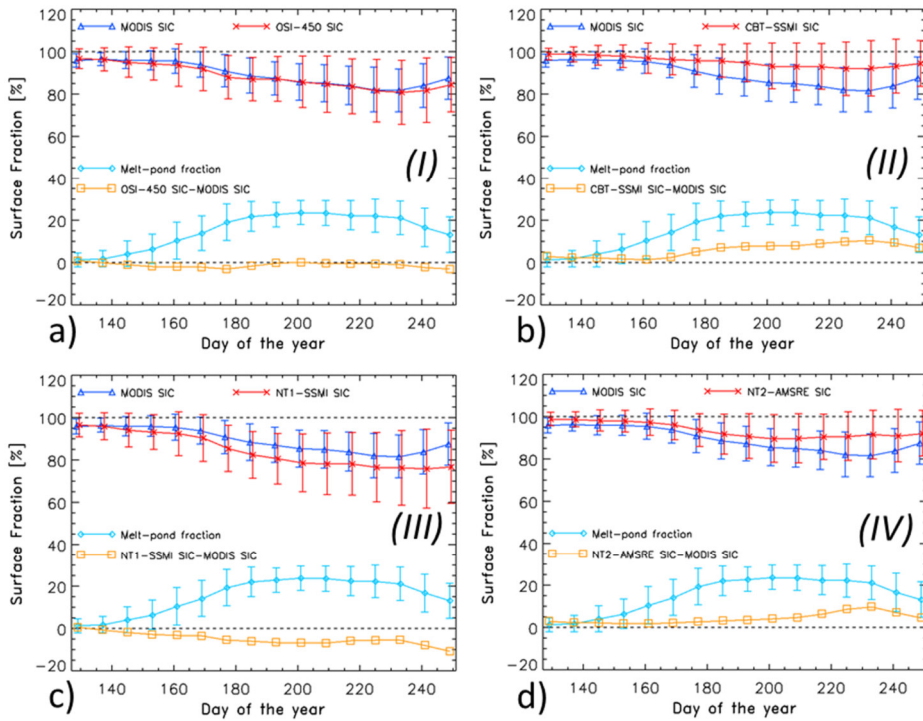
Figure 67. Average seasonal cycle of the mean (limited to Arctic Ocean and Canadian Arctic Archipelago) MODIS SIC (in blue), PMW SIC (in red), their difference PMW minus MODIS SIC (in orange), and the MODIS melt-pond fraction (in cyan), averaged for each 8-day period for the years 2003-2011 of the PMW products representing groups I to IV (see also Fig. S07, supplementary material). Error bars denote one standard deviation of the mean. Roman numerals in bold font denote the group (see Table 1) to which the algorithm is assigned.
