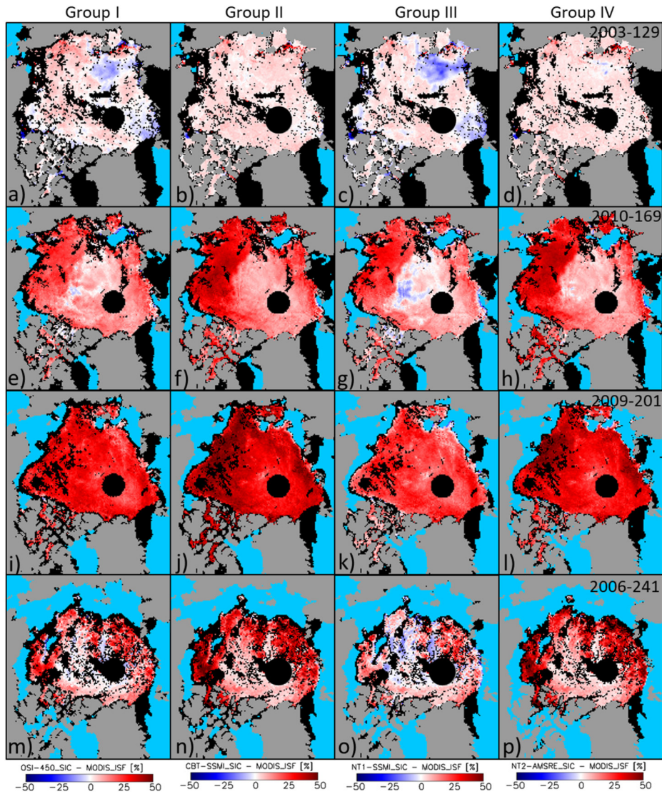
150 Figure 78. Maps of the difference PMW sea-ice concentration minus MODIS ice surface fraction (ISF) for the same 8-day periods as shown in Fig. 54. The leftmost column shows OSI-450, representing group I, the second column CBT-SSMI, representing group II, the third column NT1-SSMI, representing group III, and the rightmost column NT2-AMSRE, representing group IV. Black areas denote invalid or missing data, clouds, or grid cells being ice-covered but not considered further in the analysis, e.g. in the Greenland Sea or Hudson Bay. Row starting with (a) are representative of pre-melt, row starting with (e) is melt advance, row starting with (i) is at the peak of melt, and row starting 1155 with (m) is at the end of the melt.
