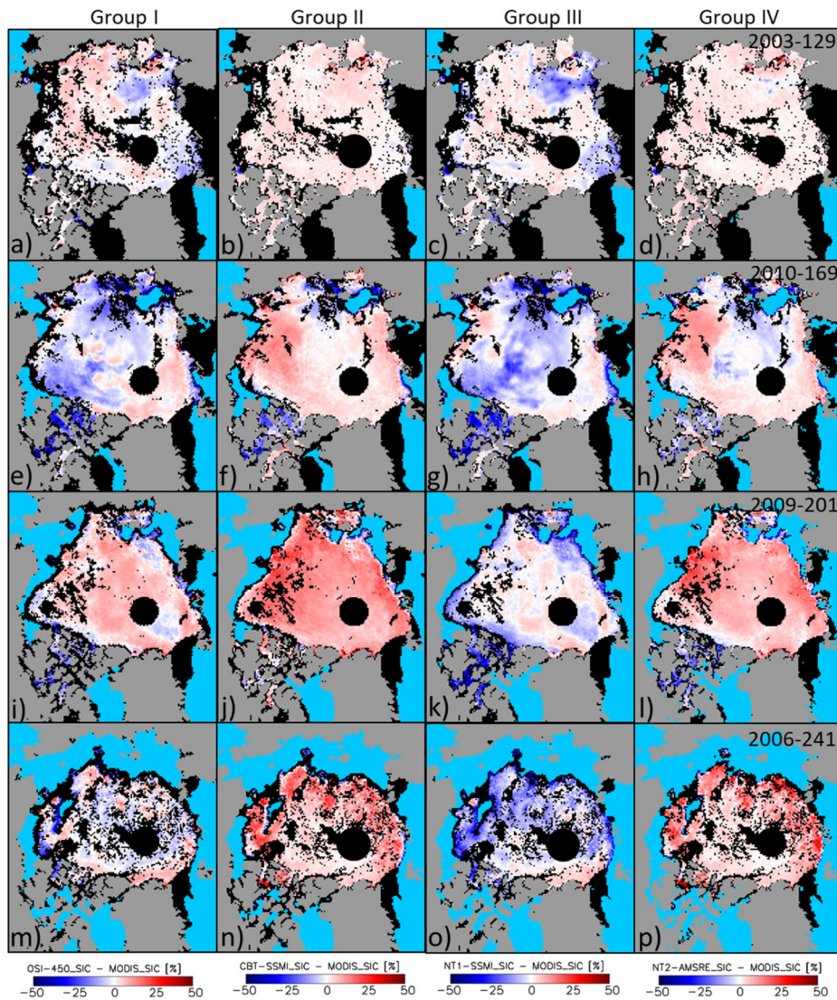
Figure 45. Maps of the difference PMW minus MODIS sea-ice concentration for a) to d): day-of-year (DOY) 129 (May 9-16) 2003, e) to h): DOY 169 (June 18-25) 2010, i) to l): DOY 201 (July 20-27) 2009, and m) to p): DOY 241 (Aug. 29-Sep. 5) 2006; these are the same periods as used in Fig. 2. The leftmost column shows OSI-450, representing group I, the second column CBT-SSMI, representing group II, the third column NT1-SSMI, representing group III, and the rightmost column NT2-AMSRE, representing group IV. Black areas denote invalid or missing data, clouds, or grid cells being ice-covered but not considered further in the analysis, e.g. in the Greenland Sea or Hudson Bay. Row starting with (a) are representative of pre-melt, row starting with (e) is melt advance, row starting with (i) is at the peak of melt, and row starting with (m) is at the end-of-melt.
