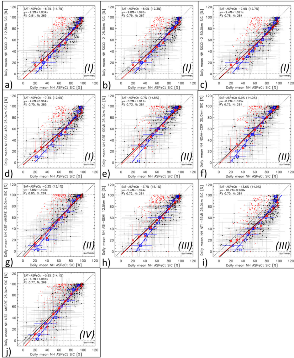
Figure 11. Scatterplots of co-located daily average SIC (black dots) and average ice-surface fraction (red dots) from visual ship-based observations (ASPeCt, x-axis) and the ten satellite SIC algorithm products (SAT, y-axis) for the Arctic for May through September for years 2002-2011 (see Fig. 3 for locations). Error bars denote one standard deviation of the average. Dotted lines denote the identity line. Solid lines denote the linear regression of the SIC data pairs. The mean difference (standard deviation), the linear regression equation, the squared linear correlation coefficient ( R^2 ) and the number of valid data pairs N is given in the top left of every image for the daily SIC value data pairs. Red triangles (blue squares) denote the average SAT SIC at 10% wide ship-based SIC bins (average ship-based SIC at 10% wide SAT SIC bins). Roman numerals in bold font denote the group (see Table 1) to which the algorithm is assigned.
