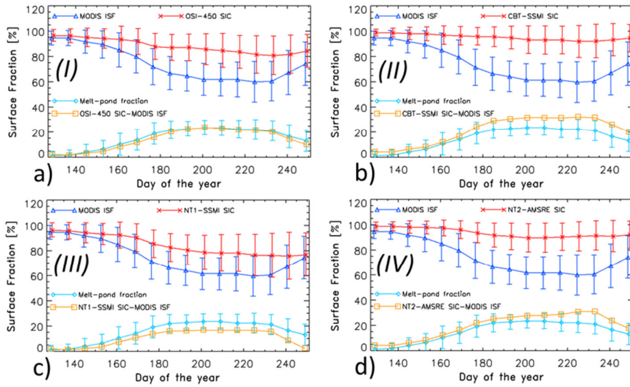
Figure 9 . Average seasonal cycle of the mean (limited to Arctic Ocean and Canadian Arctic Archipelago) MODIS ISF (in blue), PMW SIC (in red), their difference PMW SIC minus MODIS ISF (in orange), and the MODIS melt-pond fraction (in cyan), averaged for each 8-day period over the years 2003-2011 of the PMW products representing groups I to IV (see also Fig. S10 in the supplementary material). Error bars denote one standard deviation of the mean. Roman numbers in bold font denote the group (see Table 1) to which the algorithm is assigned.
