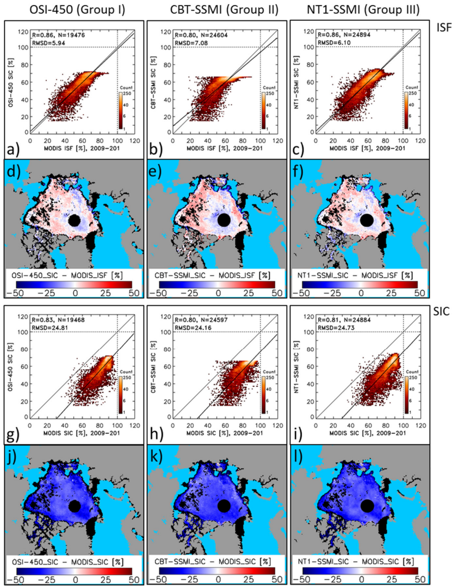
Figure 102. Illustration of the effect of a simple linear bias correction of PMW SIC towards MODIS ISF for an 8-day period during peak-melt (DOY 201, July 20-27, 2009). Topmost row, panels a) to c): Two-dimensional histograms of the distribution of bias-corrected PMW SIC (y-axis) versus MODIS ISF (x-axis) data pairs. Second row, panels d) to f): Respective maps of the difference of bias-corrected PMW SIC minus MODIS ISF. Third row, panels g) to i) Two-dimensional histograms of the distribution of bias-corrected PMW SIC (y-axis) versus MODIS SIC (x-axis) data pairs. Bottommost row, panels j) to l): Respective maps of the difference bias-corrected PMW SIC minus MODIS SIC. Leftmost, middle and rightmost columns show OSI-450 (for group I), CBT-SSMI (for group II), and NT1-SSMI (for group III). Bin size in the histograms is 1%. The quantities given in the top left corner are R: linear correlation coefficient, N: number of valid data
