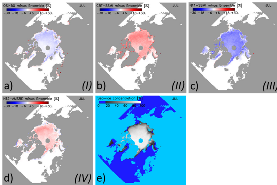
Figure 43. (a) to (d) Maps of the difference between the multi-annual average monthly SIC of the individual algorithms representing groups I to IV and the 10-algorithm ensemble median multi-annual average monthly SIC (e) for the Arctic for July 2003-2011 (see also Fig. S04, supplementary material). Differences are only computed for sea-ice concentration of both data sets larger than 15%. Roman numbers in bold font denote the group (see Table 1) to which the algorithm is assigned.
