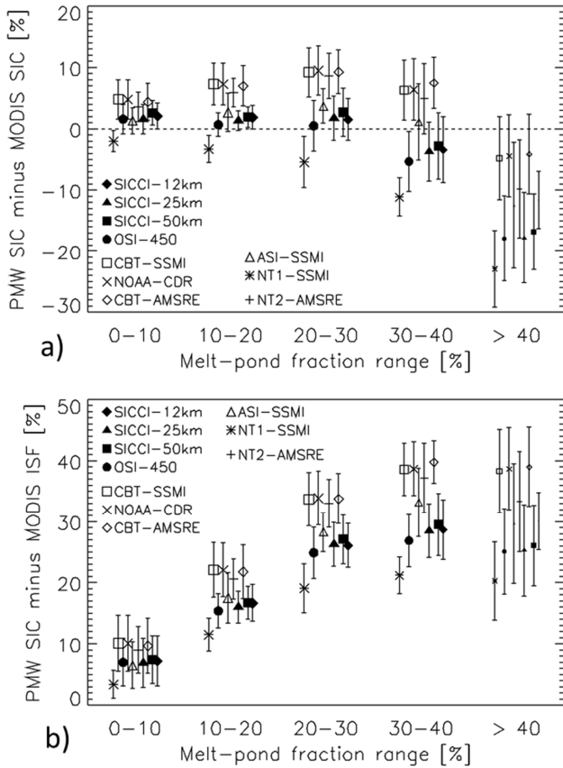
Figure 113. Mean difference PMW SIC minus MODIS SIC (image a) and PMW SIC minus MODIS ISF (image b) derived for all 8-day periods of the years 2003-2011 for all ten products separately for melt-pond fraction ranges 0-10 % to > 40 %. Error bars denote one standard deviation of the mean. Symbol size scales with the number of valid data pairs. The topmost four and bottommost three entries in left column of annotations denote group I (filled symbols) and group II, respectively. The topmost two entries and the last entry in right column of annotations denote group III and group IV, respectively.
