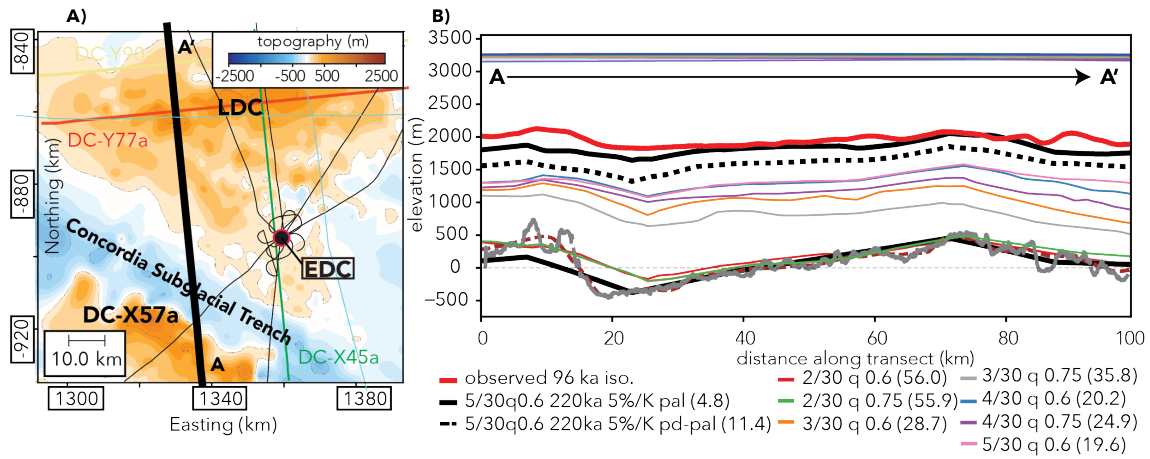
Figure 7. Comparison of the observed and modelled 96 ka isochrone along radar profile DC-X57a (red line in right panel) in the Dome C region: A) depicts the study area and the location of the radar transect corresponding to the simulated and observed isochrone. B) 96 ka observed isochrone elevation in red, paleoclimate simulation with 5\%K^{-1} precipitation scaling black line, present-day output of the paleoclimate simulation (black dashed line) and present-day equilibrium simulations as well as corresponding surface elevations (colored lines). The observed surface elevation is plotted in dark blue. Root mean square difference (%) between observed and modelled isochrone elevation is given by the numbers in the legend of B). Bedrock elevation in the pal model run is plotted in black and bedrock elevation derived from the radar transect in grey. The gridded 1km BedMachine bedrock elevation (Morlighem et al., 2020) is plotted for comparison as well (smooth dashed red line).
