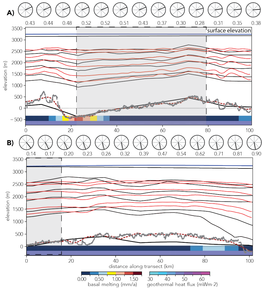
Figure 9. Modelled (black lines) and observed isochrones (red lines 38, 48, 74, 96, 130, 160 ka from top to bottom) for transect DC-X57a (A) and DC-Y77a (B) (orientation from left to right as depicted in Figure 7 A). The grey vertical bars highlight areas with low elevation differences in the low resolution model bedrock input (black line) compared to the high resolution radar observations (grey line) which generally correspond to a good match of modelled and observed isochrones. Bedrock and surface elevation in the model runs is plotted in black. Observed surface elevation is plotted in dark blue. The 1 km BedMachine data (Morlighem et al., 2020) is depicted by the red dashed line. The labeled circles denote the surface flow and magnitude in m/a relative to the direction of the transect. The coloured bars on the bottom depict the geothermal heat flux (Shapiro and Ritzwoller, 2004) and the computed basal melt rate along the transect.
