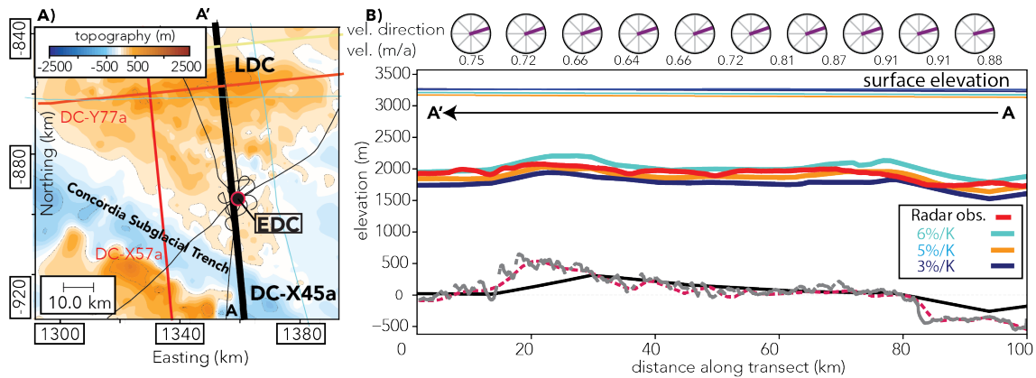
Figure 5. Transect DC-DC-X45a with the 96 ka isochrone. Panel A) illustrates the bedrock elevation and radar transects analysed in this study crossing Dome C. In B) the computed isochrone elevations for simulations with 3%, 5% and 6% precipitation change per Kelvin surface temperature change are plotted against the observed isochrone (red line). The modelled surface elevation is plotted in the corresponding color of the modelled isochrones and the observed surface elevation (Fretwell et al., 2013) is depicted in dark blue. Bedrock elevation in the model is plotted in black and bedrock elevation derived from the radar transect in grey. The gridded 1km BedMachine bedrock elevation (Morlighem et al., 2020) is plotted for comparison as well (smooth dashed red line). The circles on the top of B) denote the relative flow direction and speed with respect to the radar transect.
