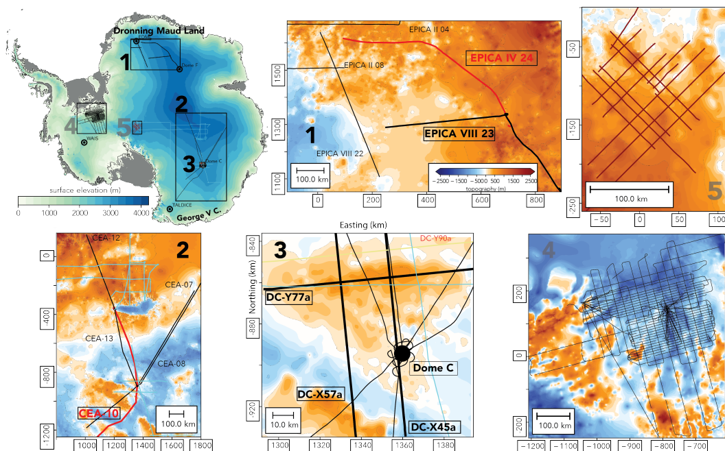
Figure 1. Antarctic surface (top left) and bedrock elevation from BedMachine Antarctica (Morlighem et al., 2020) overlain by radar transects with individual dated isochrones analysed in this study. The enlarged sections highlight regional clusters and their respective topographic settings. Clusters 1-3 are discussed in this study. The isochrone data are from: cluster 1) Winter et al. (2019), cluster 2) and 3) Leysinger Vieli et al. (2011); Cavitte et al. (2016, 2020); Winter et al. (2019), cluster 4) Beem et al. (2020), cluster 5) Ashmore et al. (2020). Northing/Easting is attained via cartographic transformation based on the WGS84 reference coordinate system.
