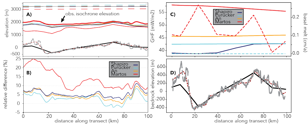
Figure 8. Illustration of model data along DC-X57a transect with a temperature precipitation scaling of 3\%K^{-1} . Panel A) shows the modelled surface (dashed lines, observed ice surface is depicted by the thin black line) and isochrone elevation under geothermal heat flux boundary conditions from Shapiro and Ritzwoller (2004); Purucker (2013); An et al. (2015); Martos et al. (2017). Panel B) depicts the isochrone mismatch (normalised by local ice thickness) between modelled and observed isochrone elevations. Panel C) shows the geothermal heat flux along the transect and the associated modelled basal melt (dashed lines). Panel D) highlights the bedrock elevation from the model simulation based on the Bedmap2 (Fretwell et al., 2013) at 16 km resolution (black line), bedrock radar reflection (Cavitt et al., 2016) (gray line) and Bedmachine Antarctica (Morlighem et al., 2020) data at 1 km resolution (red dashed line).
