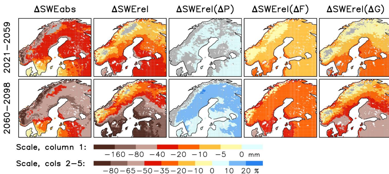
Figure 9. Multi-RCM mean changes in March mean SWE from years 1982-2020 to 2021-2059 (top) and 2060-2098 (bottom). Columns 1-2: change in SWE in absolute (mm) units and in per cent of the 1982-2020 multi-RCM mean. Columns 3-5: contributions of total precipitation change ( \Delta P ), snowfall fraction ( \Delta F ) change and snow-on-ground fraction ( \Delta G ) change to the per cent change in SWE. Grey shading is used in areas where less than 14 of the 17 RCM simulations agree on the sign of the change.
