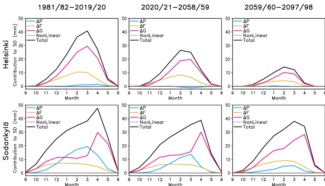
Figure 11. Multi-RCM mean interannual standard deviation of SWE (black line) in Helsinki (top) and Sodankylä (bottom) in the periods 1981/82-2019/20 (left), 2020/21-2058/59 (middle) and 2059/60-2097/98 (right) and the contributions of the four rhs terms in Eq. (2) to it (coloured lines).
