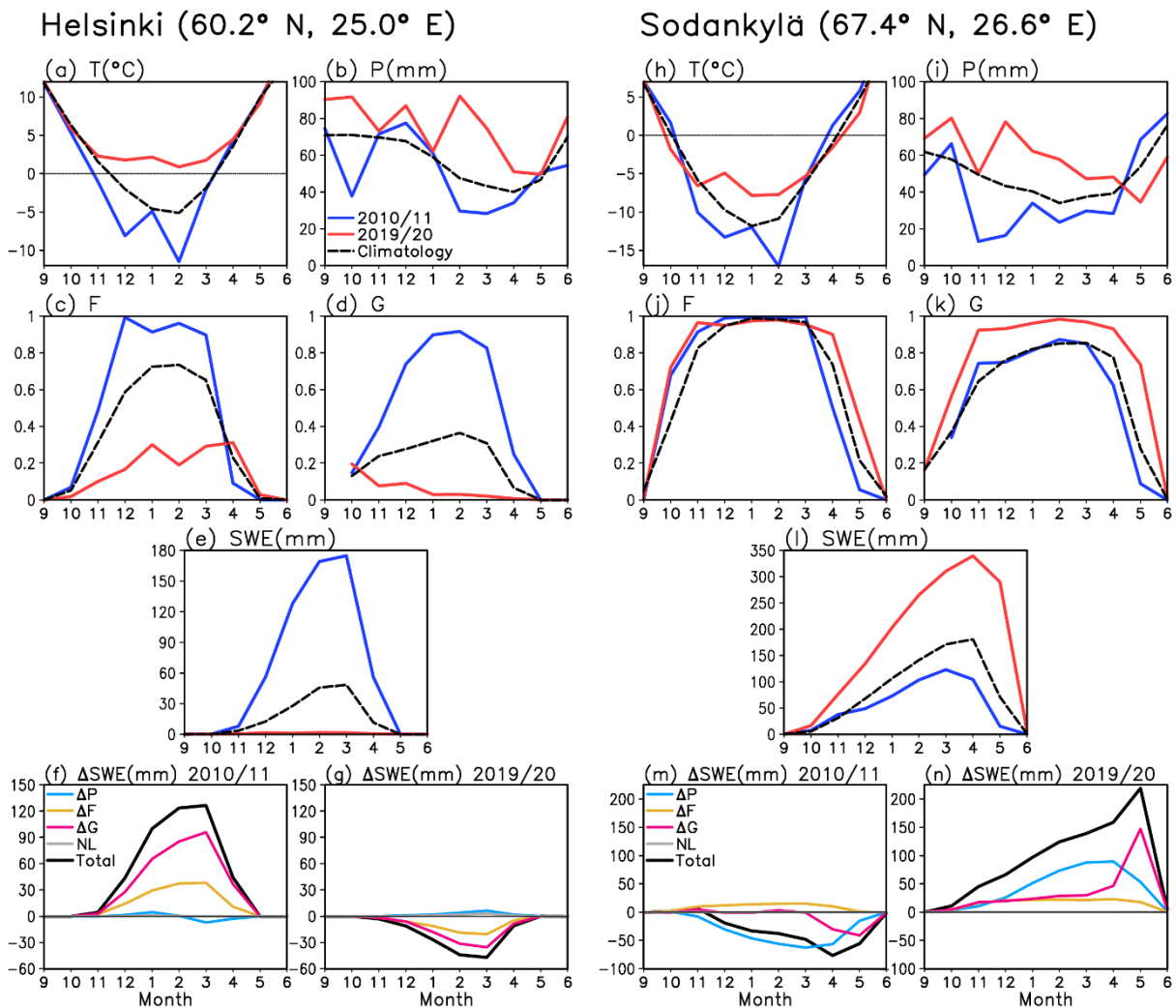
175 Figure 4. (a)-(g) Weather and SWE diagnostics for winters 2010/11 and 2019/20 for the ERA5-land grid box closest to Helsinki. (a)-(e): temperature T , precipitation P , snowfall fraction F , snow-on-ground fraction G and SWE in 2010/11 (blue), 2019/20 (red) and the corresponding 39-winter mean values (black). (f)-(g): decomposition of the winter 2010/11 and 2019/20 SWE anomalies to contributions from the four rhs terms in (2) (see the legend in (f) for line colors). (h)-(n) The same for Sodankylä.
