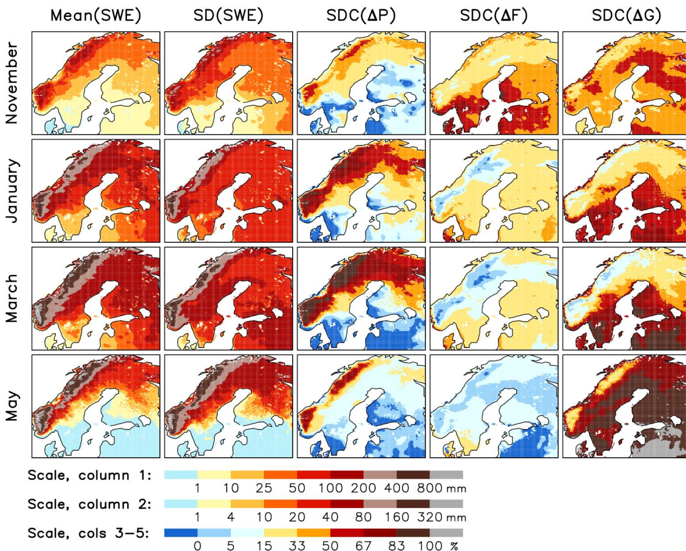
240 Figure 7. Statistics of SWE in ERA5-Land, winters 1981/82 to 2019/20. Columns 1-2: mean and interannual standard deviation of SWE (in mm). Columns 3-5. Relative contributions of total precipitation ( \Delta P ), snowfall fraction ( \Delta F ) and snow-on-ground fraction ( \Delta G ) to the standard deviation of SWE (in %). The colour scales are given at the bottom of the figure.
