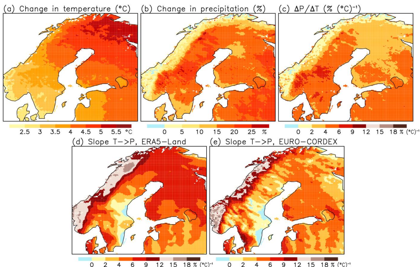
Figure 10. Top: multi-RCM mean changes in NDJFM mean (a) temperature T and (b) precipitation P from 1981/82-2019/20 to 2059/60-2097/98, and (c) the ratio of the precipitation change to the temperature change. Bottom: slope b in least-square linear regression P(\text{NDJFM}) = a + bT(\text{NDJFM}) for interannual variability in 1981/82-2019/20, in (d) ERA5-Land and (e) as averaged over the EURO-CORDEX RCMs. 330
