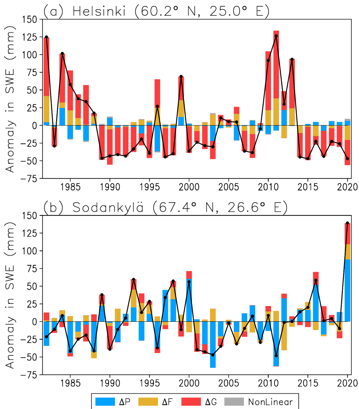
210 Figure 5. Anomalies of March mean SWE in (a) Helsinki and (b) Sodankylä in years 1982-2020 based on ERA5-Land. The solid line shows the total SWE anomaly and the bars the contributions of the four rhs terms in Eq. (2).
