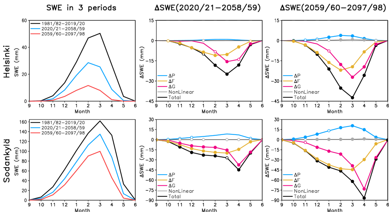
Figure 8. Left: multi-RCM mean SWE in Helsinki and Sodankylä in the winters 1981/82-2019/20 (black), 2020/21-2058/59 (blue) and 2059/60-2097/98 (red). Middle: the changes from 1981/82-2019/20 decomposed to the contributions of the four rhs terms in Eq. (2) (see the legend for line colours). Months in which all 17 (14-16 of the 17) simulations agree on the sign of the change are indicated with a closed (open) circle. Right: as middle, but for the period 2059/60-2097/98.
