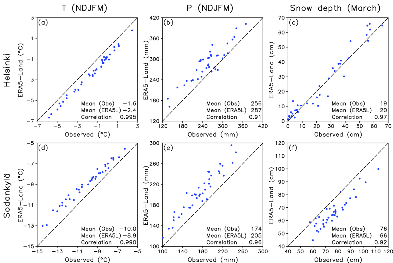
Figure 3. Comparison between station observations and ERA5-Land reanalysis of (left) NDJFM mean temperature, (middle) NDJFM precipitation and (right) March mean snow depth in winters 1981/82-2019/20. Top: station Helsinki Kaisaniemi vs. ERA5-Land at (60.2° N, 25.0° E); bottom: station Sodankylä Tähtelä vs. ERA5-Land at (67.4° N, 26.6° E). Station observations from the Finnish Meteorological Institute ( https://www.ilmatieteenlaitos.fi/havaintojen-lataus )
