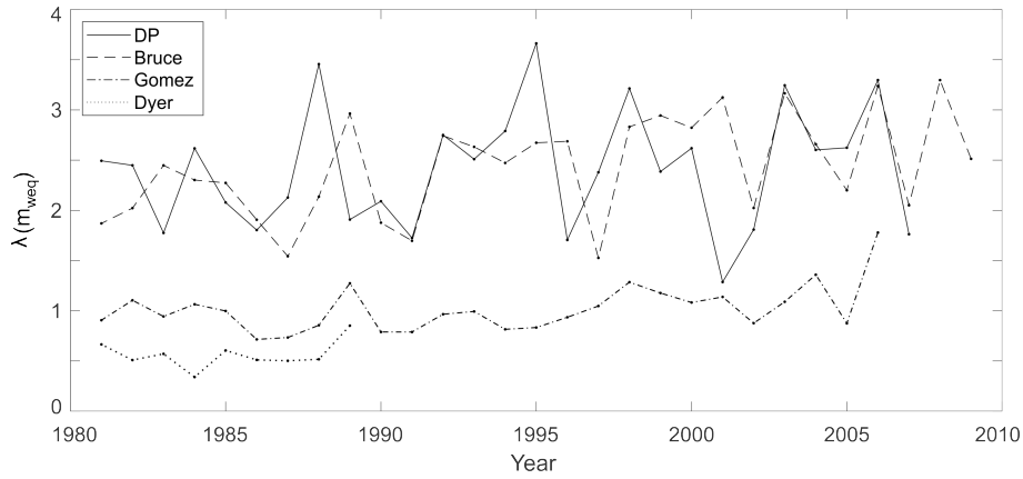
Figure 6. Annual snow accumulation in ice cores from the Antarctic Peninsula region between 1980 and 2010. DP refers to (solid line), Bruce plateau (dash line), Gomez (dot-dash line) and Dyer (dot line) for the results of this paper period 1980-2010.
