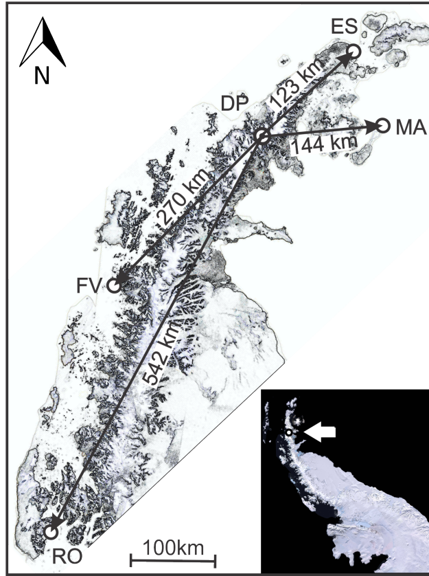
Figure 1. The four Antarctic Stations, Esperanza (ES), Marambio (MA), Faraday-Vernadsky (FV) and Rothera (RO), and the borehole at PD DP , on the Northern Antarctica Peninsula. The white arrow in the right lower corner inset shows the location of PD DP on the Peninsula. Both maps were modified from a pan-sharpened scene (RGBREF_x - 2550000y + 1350000) of the Landsat Image Mosaic of Antarctica (LIMA) by USGS https://lima.usgs.gov/
