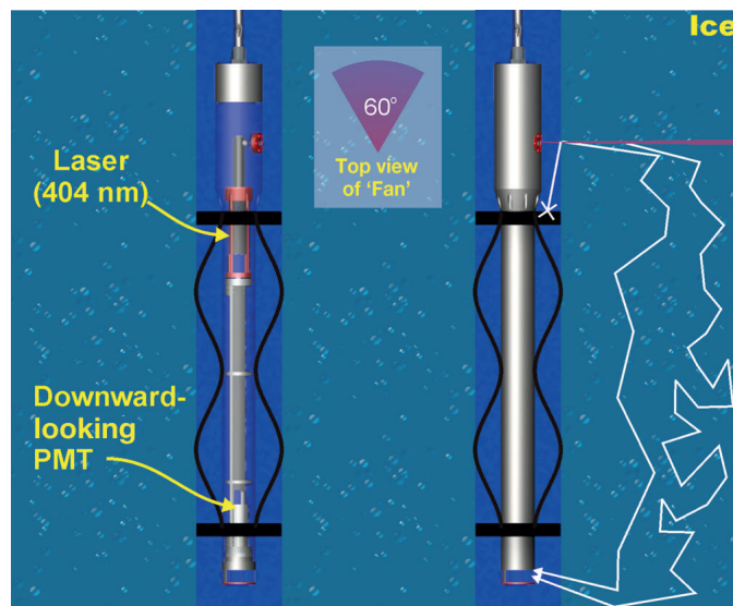
Figure 1. Sketch of the laser dust logger. Light emitted by a 404 nm diode laser in a 60° horizontal fan can only reach the photon counter below through scattering on nearby impurities.
