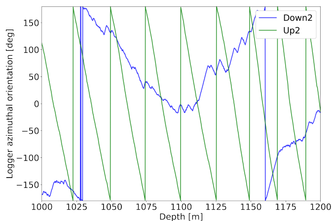
Figure 3. Rotation of the tool descending and ascending the bore hole. A smooth and continuous rotation of slightly varying angular velocity is observed when ascending. During descent the rotational movement is erratic.
