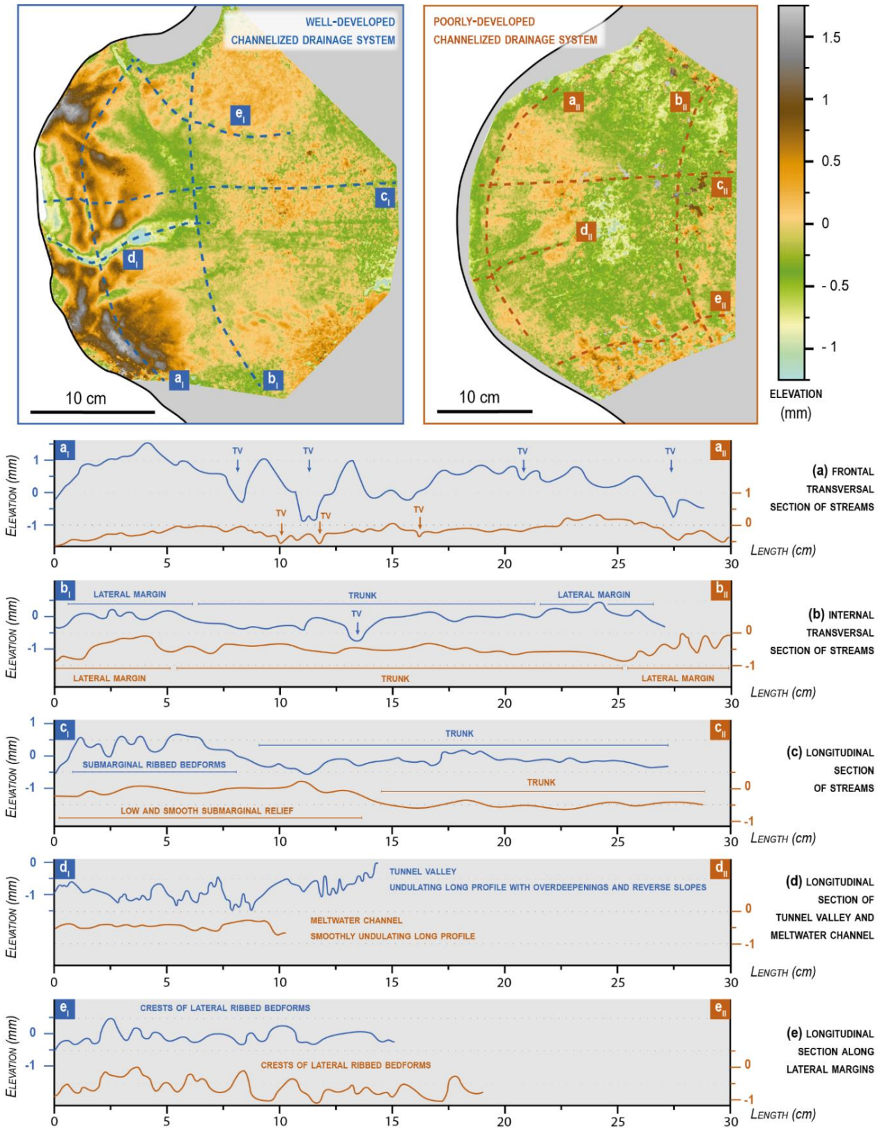
415 Figure 10. DEMs of the bed surface beneath the lobes of the silicone streams at the final stage of experiment 10 (blue) and 14 (brown). Ten elevation profiles (a to e) within the lobes are drawn to compare the morphological imprint beneath the two types of streams.
