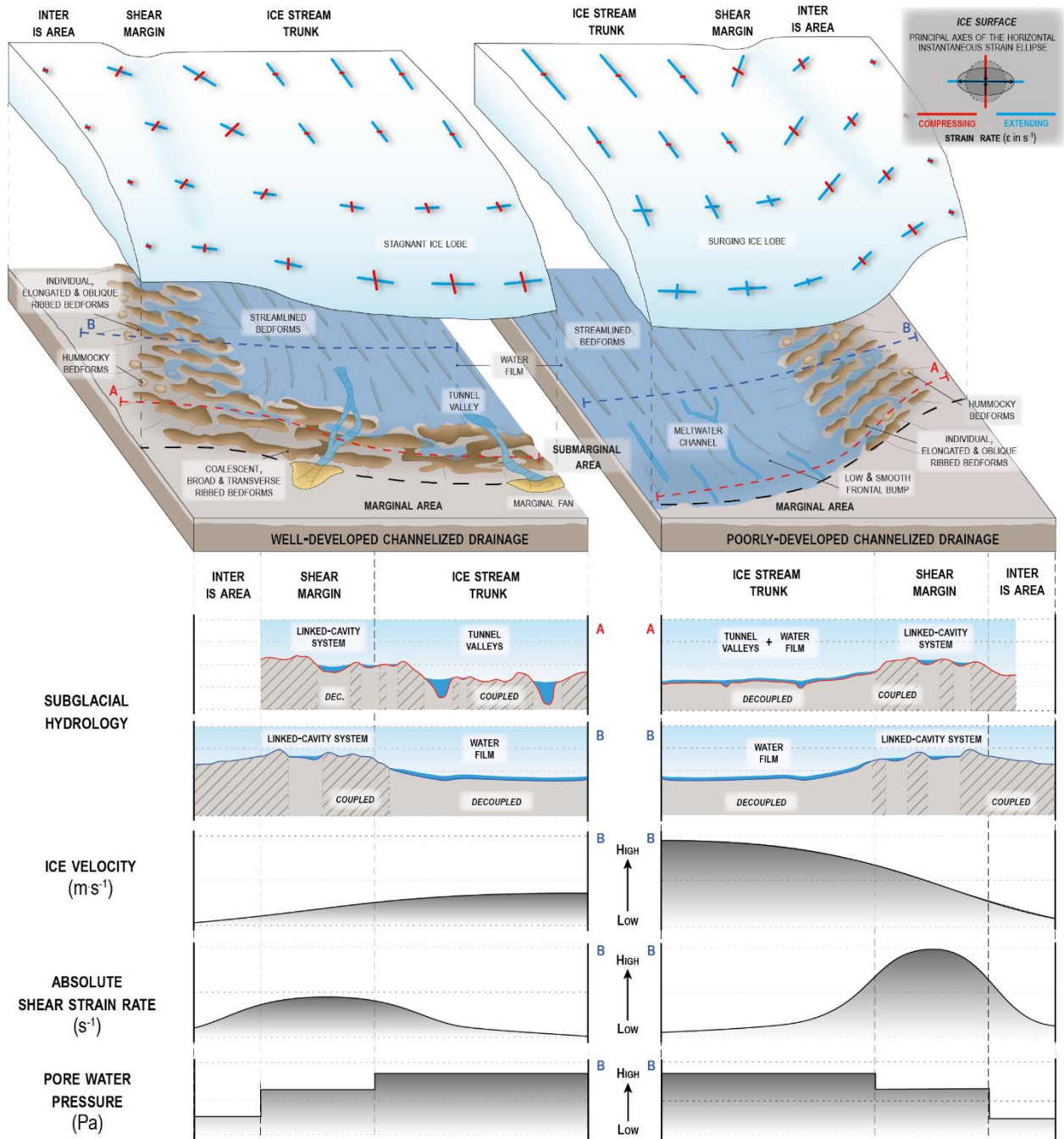
Figure 15. Conceptual model summarising our observations and interpretations and the proposed role of hydrology, ice velocity and superficial ice strain in generating the observed landforms and their spatial distribution. This is for a terrestrial ice-stream context either characterized by well-developed or poorly-developed channelized drainage below the lobe frontal margin.
