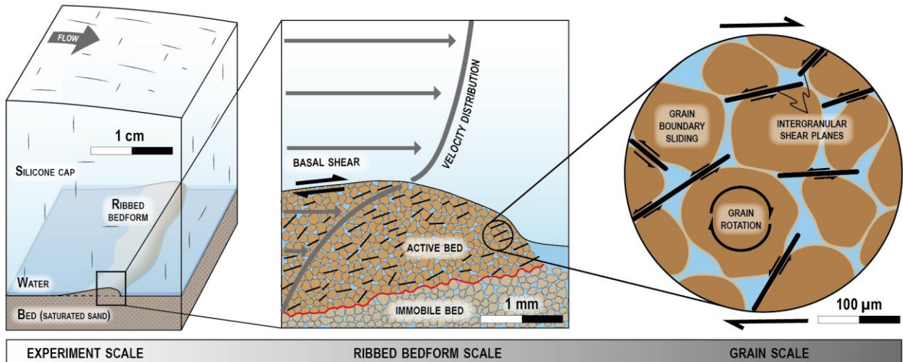
Figure 14: Model of experimental ribbed bedforms formation. Deformation of a water-saturated and granular bed during silicone-bed coupling. The active bed (i.e. superficial portion of the bed accommodating the basal shear generated by the flow of silicone putty) is able to produce millimetre-thick bedforms through boundary sliding of individual grains along intergranular shear planes and individual grain rotations.
