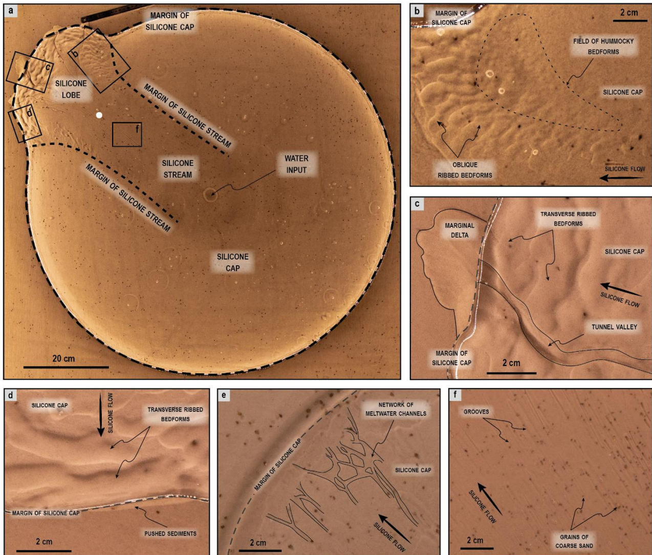
290 Figure 5. Illustration of bedform assemblages produced during the experiments. (a) Overall surface view of the silicone cap at the end of an experimental run, showing the distribution of bedforms beneath a stream/lobe system characterized by a well-developed channelized drainage (Experiment 10). The white dot indicates the position of the pressure sensor where pore water pressure presented in Fig. 4 is measured. (b) Close-up on oblique ribbed and hummocky bedforms observed at the right lateral shear margin. (c) Transverse ribbed bedforms parallel to the lobe frontal margin and formed submarginally. Tunnel valley and associated marginal delta. (d) Transverse ribbed bedforms parallel to the lobe frontal margin and pushed marginal sediments bulldozed by the lobe margin. (e) Network of meltwater channels extending parallel and perpendicular to the silicone flow (not located on (a), because it was observed in Experiment 14, characterized by a poorly-developed channelized drainage). (f) Field of grooves inscribed in the bed and oriented parallel to silicone flow with embedded sand grains at their down-stream extremities.
