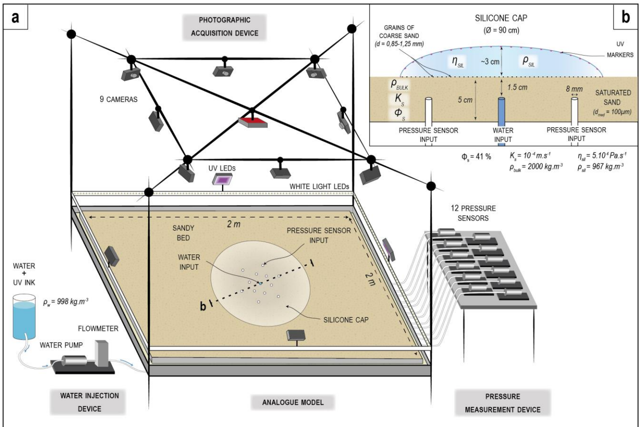
180 Figure 2. (a) Experimental model and monitoring apparatus. A cap, of transparent and viscous silicone putty, flows under its own weight above a bed composed of water-saturated sand. We inject coloured water in the bed, through an injector located below the centre of the silicone cap. We use a photographic acquisition device and pressure sensors to monitor the development of bedforms at the silicone/bed interface, the silicone flow velocity, the water flow and the water pressure. (b) Transverse section of the model with the experimental parameters.
