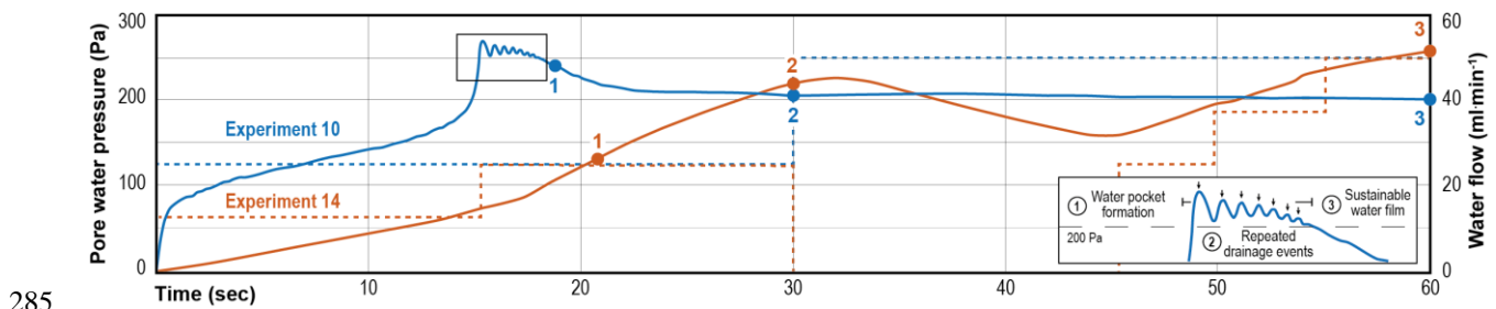
Figure 4. Evolution of pore water pressure (solid lines) measured in the trunk axis (see Fig. 5a for position) and water flow injected in the bed through the water injector (dotted lines), for Experiments 10 and 14. Points numbered 1 to 3 correspond to stages described in sections 4.1, 4.2 and 4.3.
