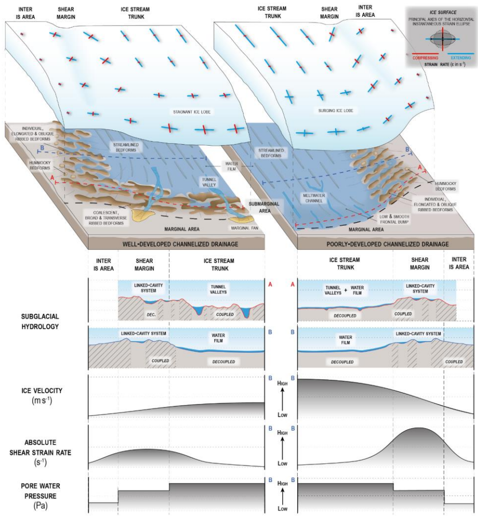
Figure 154. Conceptual model summarising our observations and interpretations and the proposed role of hydrology, ice velocity and superficial ice strains subglacial shear in generating the observed landforms and their spatial distribution. This is for a terrestrial ice-stream context either characterized by well-developed or poorly-developed channelized drainage below the lobe frontal margin.
