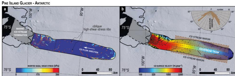
685 Figure 13: Maps of inverted (a) basal shear stress (kPa) beneath Pine Island Glacier and (b) ice-surface velocity (modified from Sergienko and Hindmarsh, 2013). Small and isolated areas of very high basal shear stress (red on (a) and black on (b)) referred to as “high-shear-stress ribs” are obliquely set to the main ice flow direction. The orientations of oblique ribs relative to mean ice-flow direction, located in the brown rectangular areas (along ice stream margins), are compiled in a rose diagram in (b) (© Landsat / Copernicus - © Google Earth).
