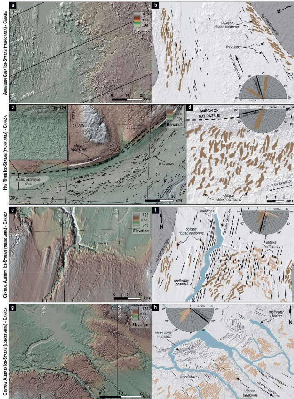
605 Figure 12. Manual mapping of ribbed bedforms, lineations and ice stream margins along different palaeo-ice stream tracks in Canada. Left panels show digital elevation models and hillshades using Arctic DEM database (Porter et al., 2018) and Lidar data (Alberta Geological Survey). Right panels show our morphological interpretations and the rose diagrams compiling bedform orientations.
