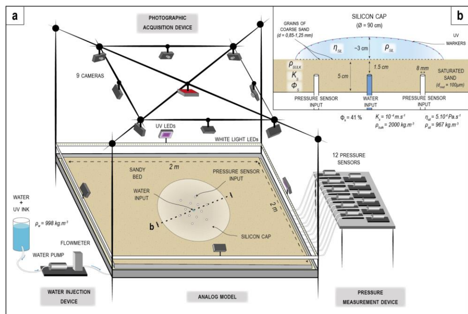
Figure 2. (a) Scheme of the experimental model and monitoring apparatus. A cap, of transparent and viscous silicon putty, flows under its own weight above a bed composed of water-saturated sand. We inject coloured water in the bed, through an injector located below the centre of the silicon cap. We used a photographic acquisition device and pressure sensors to monitor the development of bedforms at the silicon/bed interface, the silicon flow velocity, the water flow and the water pressure. (b) Transverse section of the model with the experimental parameters.
