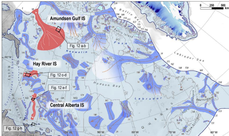
355 Figure 3. Extent of the North American Laurentide Ice Sheet during the Last Glacial Maximum with positions of known ice stream tracks (modified from Margold et al., 2018). The areas mapped in this study are identified by black rectangles in three ice streams (Amundsen Gulf, Hay River and Central Alberta IS) are identified by black rectangles .
