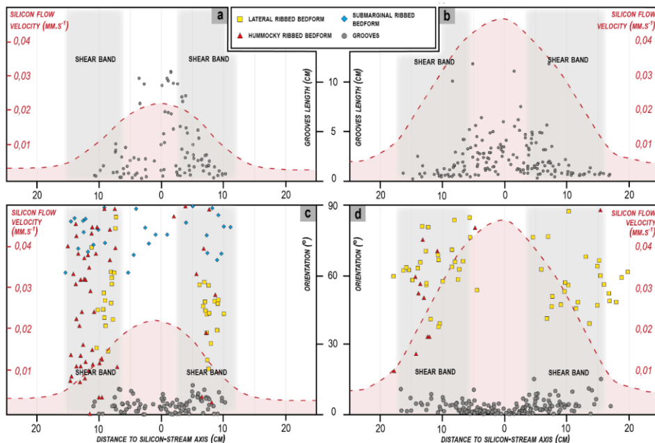
555 Figure 11. Morphometric properties of bedforms produced beneath each type of stream at the final stage of Experiments 10 (right panel) and 14 (left panel) plotted according to the distance from the silicon stream central axis. (a) and (b) relationship between groove length and silicon flow velocity ( \text{mm}\cdot\text{s}^{-1} ). (c) and (d) variation in orientation of each population of bedforms (lateral ribs, submarginal ribs, hummocky) compared to the silicon flow velocity and the shear band position (grey columns; defined as v_{\text{shear}} > 0.5 \times 10^{-4} \text{ s}^{-1} ).
