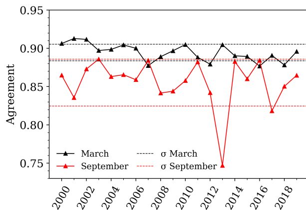
Figure 9. Agreement between NSIDC's Sea Ice Index and the obtained monthly sea ice extent maps for all analysed years.
