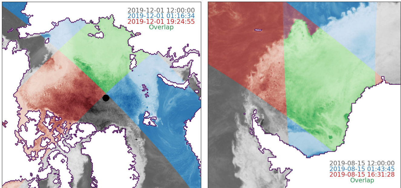
160 Figure 2: Left: daily average map of AMSR2 36.5 GHz V-pol T_B on 1 December 2019 (greys) for the Arctic, and two individual gridded swaths on the same day (blues: 01:16:34 UTC, reds: 19:24:55 UTC). The sea-ice region of overlap between the two swaths is highlighted in greens, and is where S2S drift vectors can be computed. Right: similar but for the Antarctic on 15 August 2019 (blues: 01:43:45 UTC, reds: 16:31:28 UTC)
