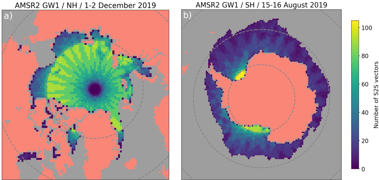
Figure 3: a) number of S2S vectors per grid cell in the Northern Hemisphere for the period 1-2 December 2019 and GCOM-W1 AMSR2 mission. b) same quantity but for the Southern Hemisphere and for the period 15-16 August 2019. Parallels at \pm 75^\circ and \pm 60^\circ are drawn.
