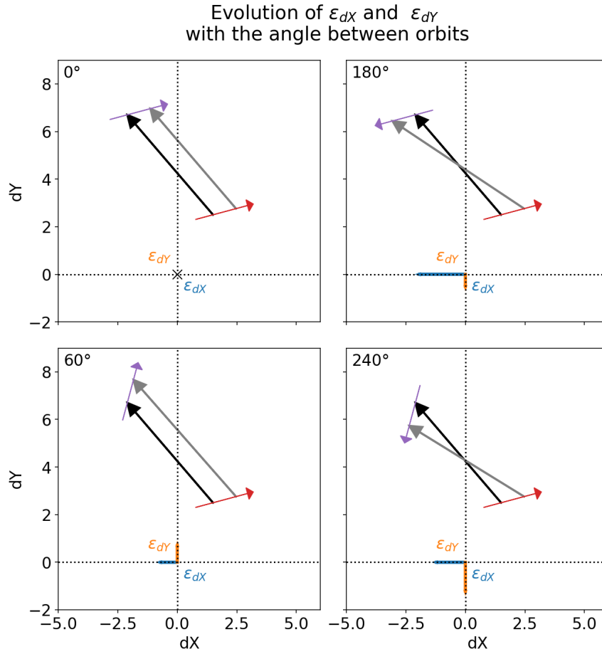
380 Figure 8: Impact of a constant geo-location error in the flight direction on S2S retrievals. Each panel corresponds to a different relative angle \theta_r between the two orbits from which sea-ice drift vectors are estimated. The true drift vector is in black, the geo-location offsets in the first and second orbits are of the same length, and create an erroneous drift vector (gray). The errors in the dX and dY components are \varepsilon_{dX} and \varepsilon_{dY} .
