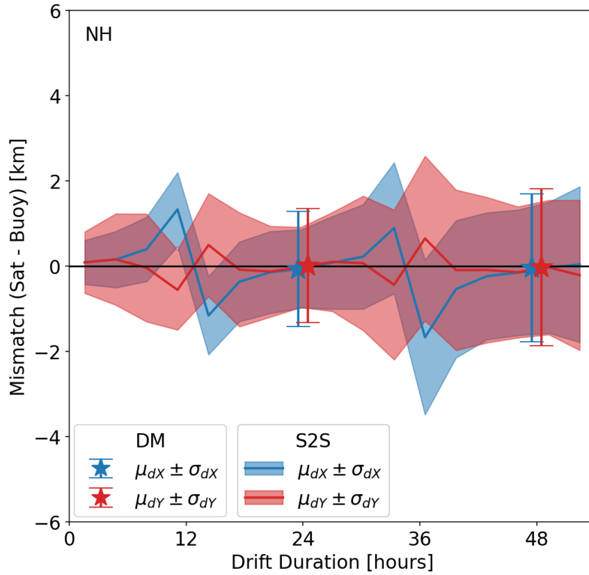
Figure 7: Same as Fig. 5 a), but for the case where the 36.5 GHz imagery is purposely mis-registered to the location of the 18.7 GHz imagery.
