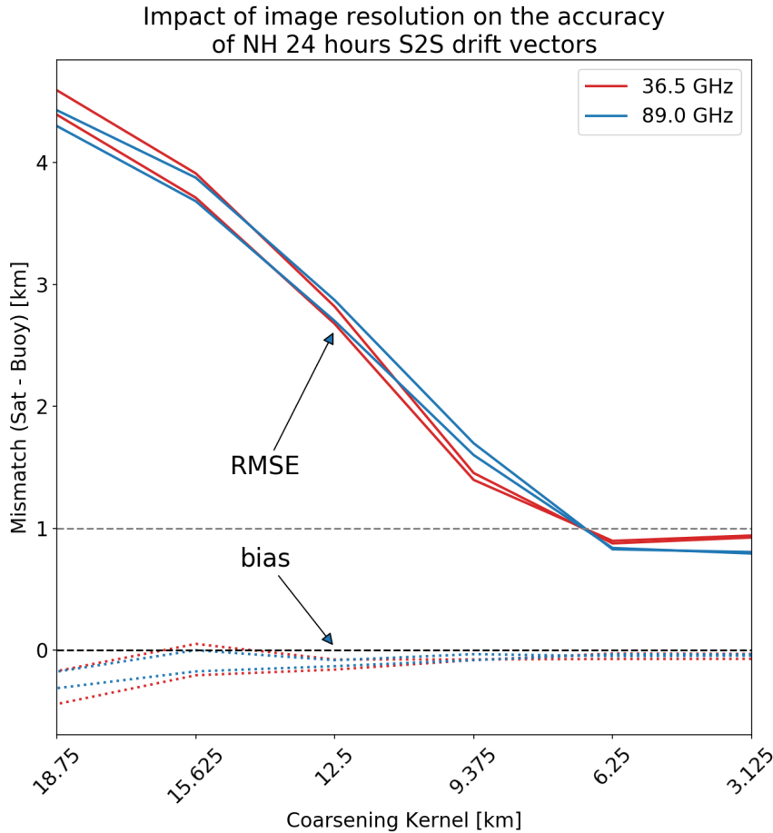
Figure 9: Bias (dashed lines) and RMSE (solid lines) of NH ~24 hours S2S drift vectors processed from GCOM-W1 AMSR2 36.5 GHz (red) and 89.0 GHz (blue) as a function of the width of an image coarsening kernel applied on 3.125 km images. The best image resolution is to the right of the x-axis. The lines do not distinguish between the dX and dY components of the drift vectors as they evolve in a similar manner.
