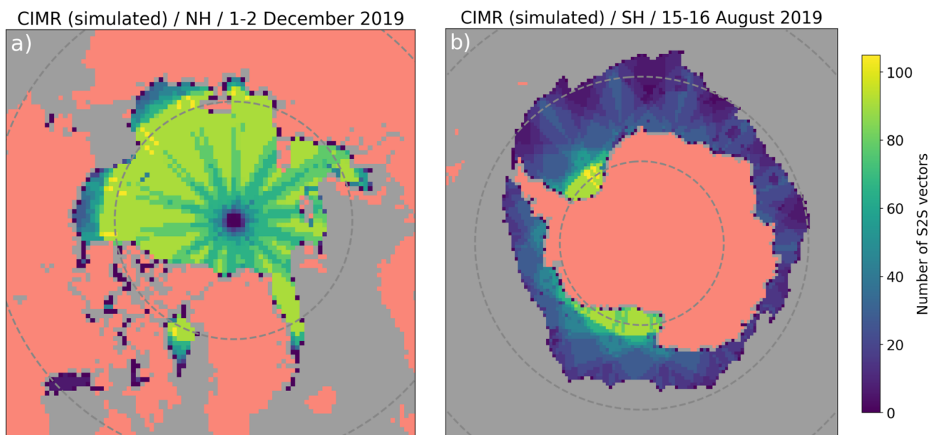
Figure 10: Same as Fig. 3 but for simulated CIMR coverage. a) number of S2S vectors per grid cell in the Northern Hemisphere with the same sea-ice cover as 1-2 December 2019. b) number of S2S vectors per grid cell in the Southern Hemisphere and with the same sea-ice cover as 15-16 August 2019. Parallels at \pm 75^\circ and \pm 60^\circ are drawn.
