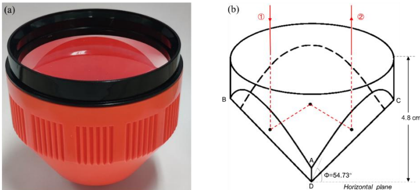
625 Figure A1. (a) CCR head used for calibration of ICESat-2 ATL03 data, and (b) parameters of the lens system and optical path of a total-reflecting photon.
