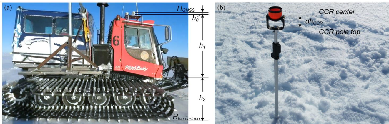
Figure 4. (a) GNSS roving receivers mounted on the roof of a Pisten Bully snowcat and boresight parameters for ice surface elevation estimation from the GNSS observations, and (b) CCR installed in the field with the pole top elevation ( h_{Pole\ top} ) surveyed by GNSS and the CCR center height ( dh_{CCR} ) measured using a steel tape.
