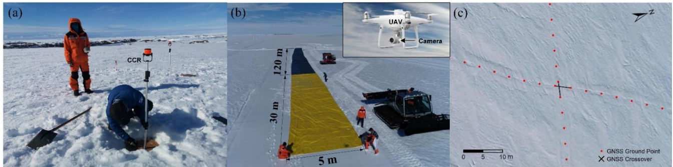
125 Figure 2. (a) Ten CCRs were installed along a line across an ICESat-2 ground track at each site; (b) a two-coating RTS (5 m × 150 130 m with yellow and dark green coatings) was deployed near Zhongshan Station and surveyed by a UAV; and (c) example of a GNSS crossover point and snowcat tracks on a UAV image.
