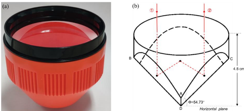
605 Figure A1. (a) CCR head used for calibration of ICESat-2 ATL03 data, and (b) parameters of the lens system and optical path of a total-reflecting photon.
