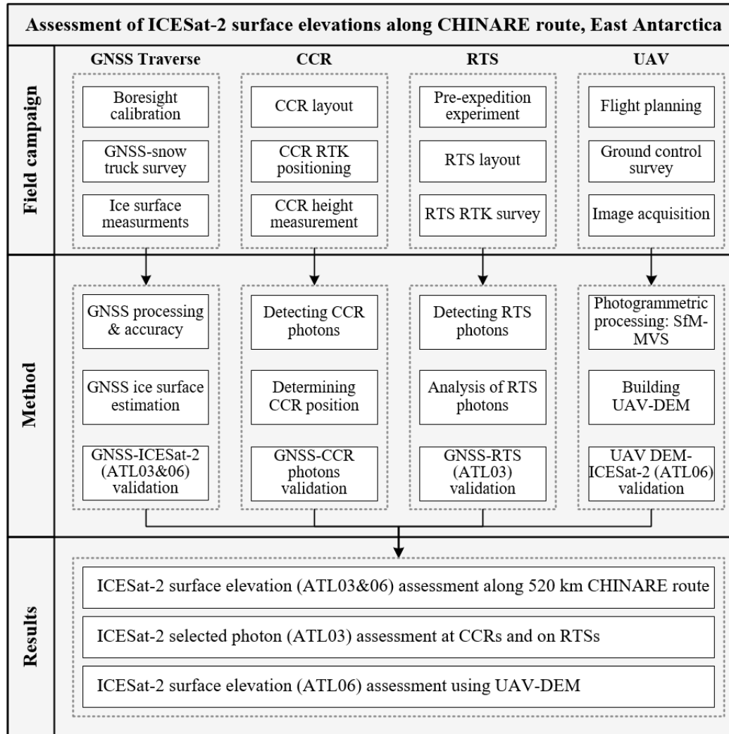
Figure 3. Flow chart for assessment of ICESat-2 ice sheet surface elevations along the CHINARE route as well as two validation sites, East Antarctica, based on coordinated multi-sensor observations.
