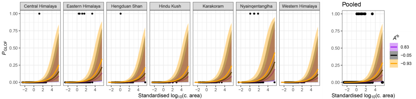
Figure 7: Glacier-mass balance model: posterior probabilities P_{\text{GLOF}} as a function of standardised catchment area C and standardised lake-area change A^{*b} between 2005 and 2018, grouped by regions of average glacier-mass balance (see Fig. 1). Black dots are lake data with (no) reported GLOF records for the interval 2005 to 2018. Thick coloured lines are mean fits, and colour shades encompass the associated 95% HDIs.
