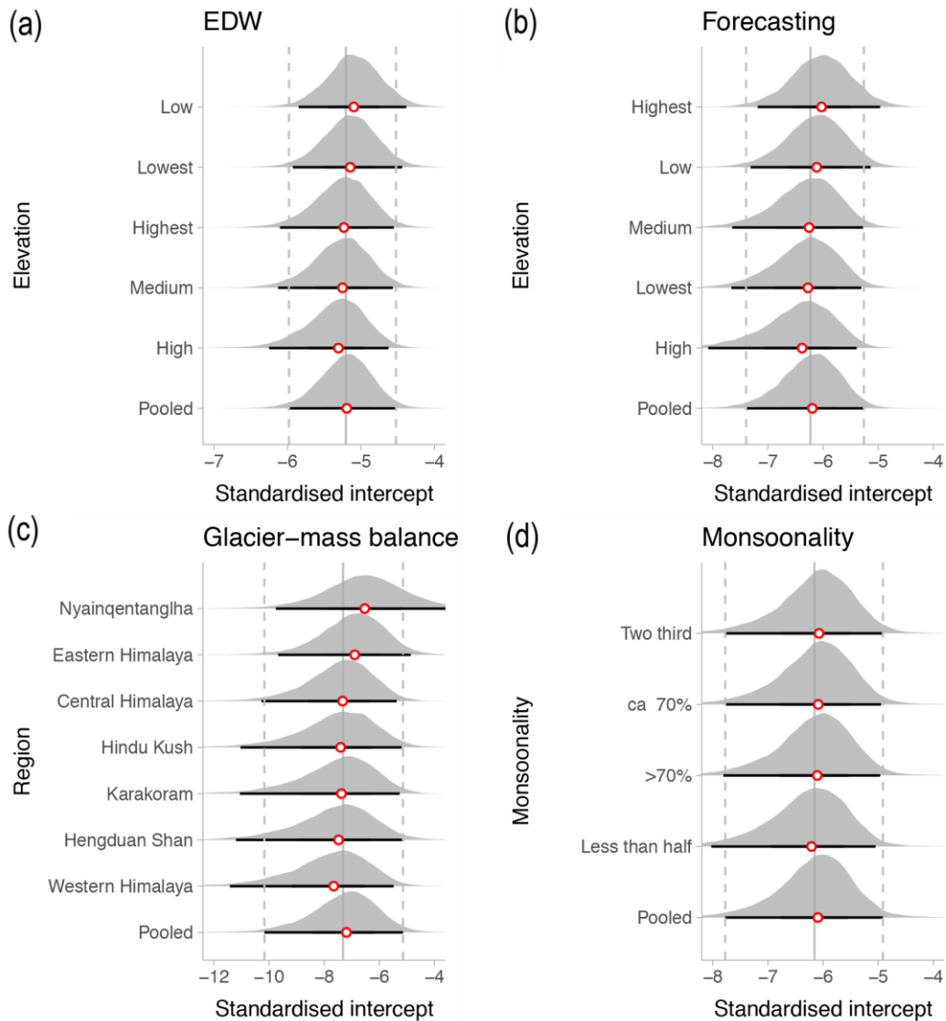
280 Figure 4: Posterior pooled and group-level intercepts for the four models considered; EDW = elevation-dependent warming; see Fig. 1 for a summary of the quantiles of elevation and monsoonality. Black horizontal lines delimit 95% HDI, red circles indicate posterior medians. Vertical continuous (dashed) grey lines are posterior means (95% HDI) of the pooled intercept of each model. Intercepts are standardised and thus refer to lakes with average predictor values.
