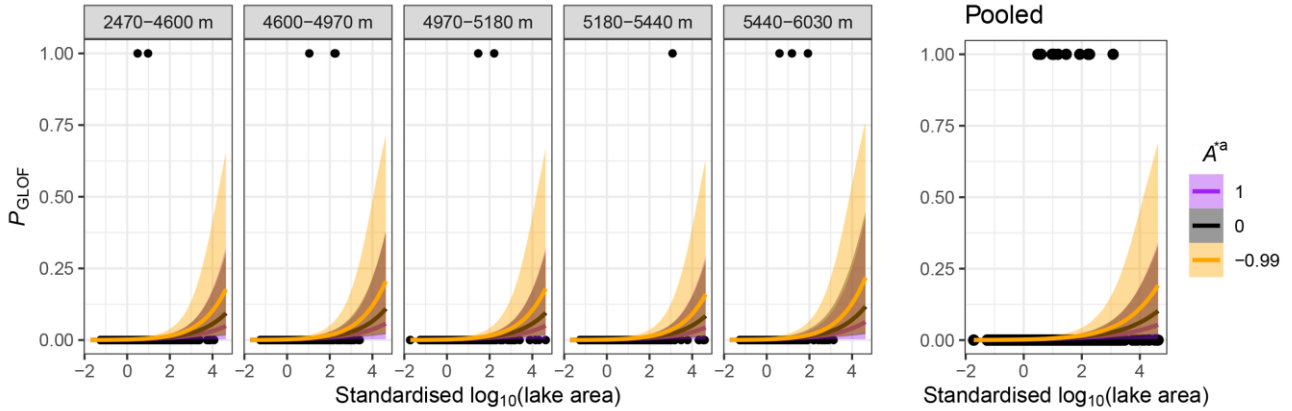
310 Figure 6: Forecasting model: posterior probabilities P_{\text{GLOF}} as a function of standardised lake area A (in 2005) and standardised lake-area change A^{*a} between 1990 and 2005, grouped by quantiles of elevation (defined in Fig. 1; lowest: 2470-4600 m a.s.l., low: 4600-4970 m a.s.l., medium: 4970-5180 m a.s.l., high: 5180-5440 m a.s.l., highest: 5440-6030 m a.s.l.). Black dots are lake data with (no) reported GLOF records for the interval 2005 to 2018. Thick coloured lines are mean fits, and colour shades encompass the associated 95% HDIs.
