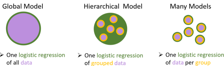
220 Figure 3: Schematic comparison of global vs. multi-level logistic regression models.
