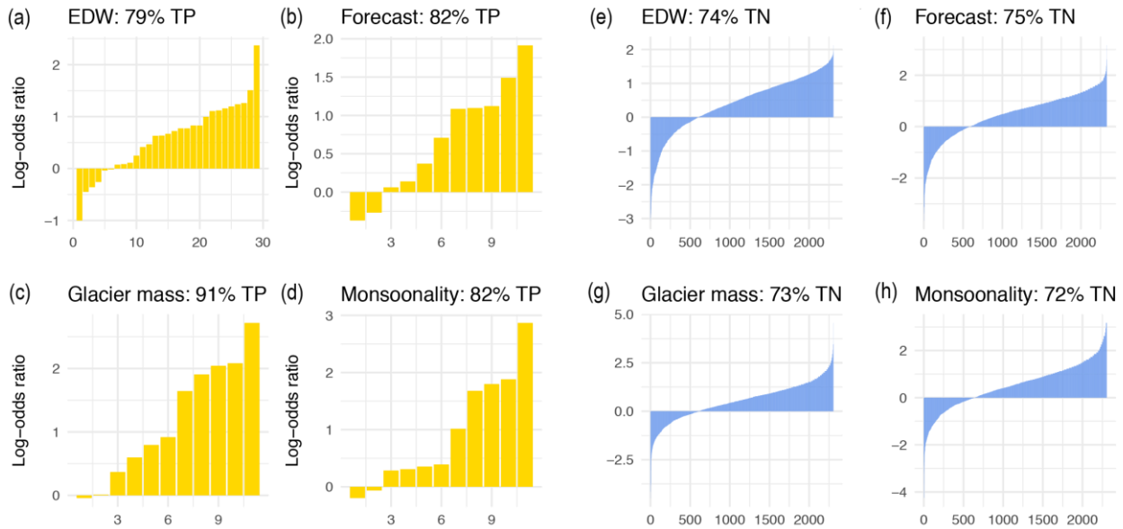
Figure 9: Average posterior log-odds ratios for true positives TP (negatives, TN), i.e. lakes with (without) a GLOF in the period 1981 – 2018 (a and e) and 2005 – 2018 (b-d and f-h) in the past four decades (on the x axis) for the four different models. The log-odds ratios describe here the ratio of the mean posterior over the mean prior probability of classifying a given lake as having had a GLOF. We estimate the mean prior probability from the relative frequency of GLOFs in the datasets; EDW = elevation-dependent warming model.
