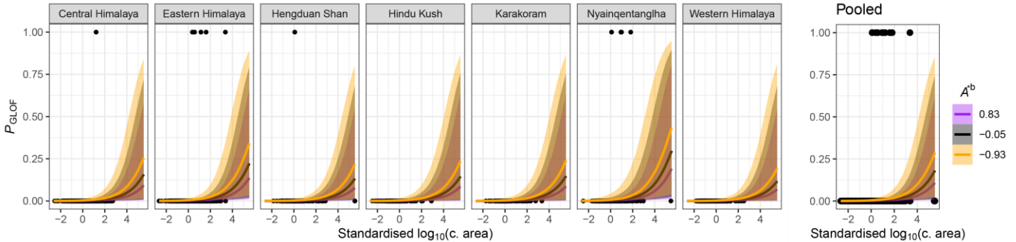
Figure 7: Glacier-mass balance model: posterior probabilities P_{\text{GLOF}} as a function of standardised catchment area C and standardised lake-area change A^b between 2005 and 2018, grouped by regions of average glacier-mass balance (see Fig. 1). Black dots are lake data with (no) reported GLOF records for the interval 2005 to 2018. Thick coloured lines are mean fits, and colour shades encompass the associated 95% HDIs.
