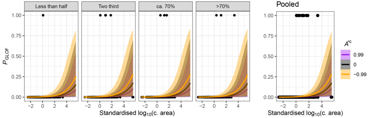
Figure 8: Monsoonality model: posterior probabilities P_{\text{GLOF}} as a function of standardised catchment area C and standardised lake-area change A^c between 1990 and 2018, grouped by quantiles of the annual proportion of precipitation falling during summer (defined in Fig. 1). Black dots are lake data with (no) reported GLOF records for the interval 1990 to 2018. Thick coloured lines are mean fits, and colour shades encompass the associated 95% HDIs.
