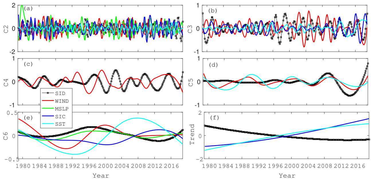
Figure 10. The IMF modes (a-e) and trend components (f) after EEMD of the third sea ice EOF temporal coefficient and each environmental parameter. (For each environmental parameter, only the EOF component marked with an asterisk is drawn.)
