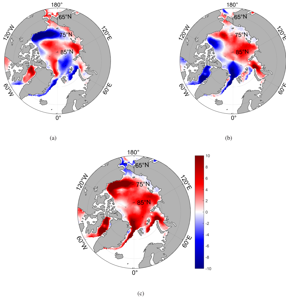
Figure 4. Annual spatial distribution of monotonic variation trends in sea ice motion from 1979 to 2018. (a) The zonal component of drift speed (red shading values indicate enhanced eastward drift, while blue shading values indicate enhanced westward drift, where east is counterclockwise), (b) the meridional component of drift speed (red shading values indicate enhanced northward drift, while blue shading values indicate enhanced southward drift, where north is toward the center of the grid) and (c) total drift velocity (red shading values indicate drift velocity increases, while blue shading values indicate drift velocity decreases). The significance test was carried out by the Mann-Kendall nonparametric test ( p < 0.05 ).
