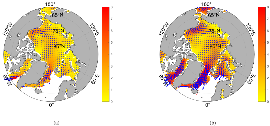
Figure 3. Climatological distribution of the sea ice drift speed field in summer (a) and winter (b) from 1979 to 2018 (the different shading represent the velocity, and the arrows represent the direction and magnitude of ice drift).
