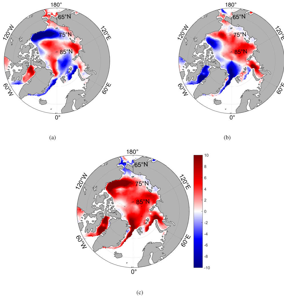
Figure 4. Annual spatial distribution of monotonic variation trends in sea ice drift-velocity-motion from 1979 to 2018. (a) The zonal component of drift speed (red shading values indicate enhanced eastward drift, while blue shading values indicate enhanced westward drift, where east is counterclockwise), (b) the meridional component of drift speed (red shading values indicate enhanced northward drift, while blue shading values indicate enhanced southward drift, where north is toward the center of the grid) and (c) total drift velocity (red shading values indicate drift velocity increases, while blue shading values indicate drift velocity decreases). The significance test was carried out by the Mann-Kendall nonparametric test ( p < 0.05 ).
