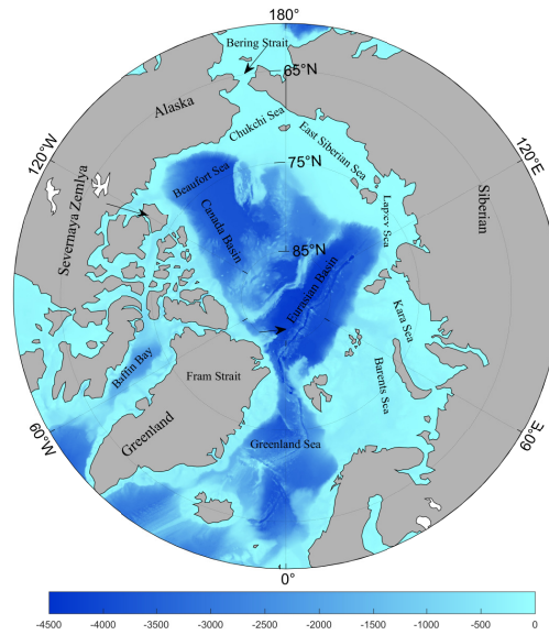
Figure 1. Geographic map of the Arctic and its adjacent seas (the colors shading represent the water depth in m).
