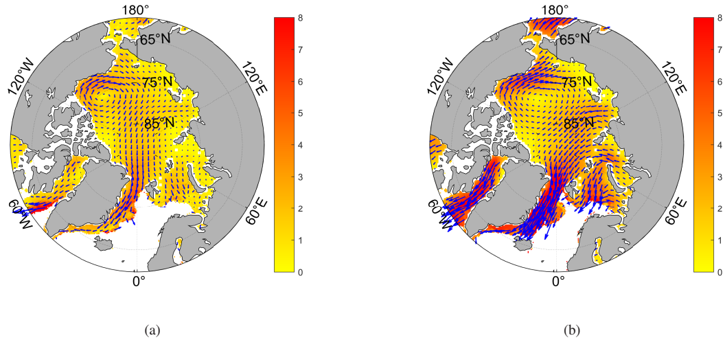
Figure 3. Climatological distribution of the sea ice drift speed field in summer (a) and winter (b) from 1979 to 2018 (the different colors shading represent the velocity, and the arrows represent the drift direction and magnitude of ice drift).
