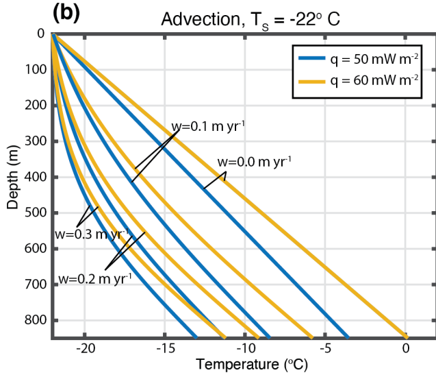
550 Figure 6. Modeled ice sheet thermal structure. Panel (a) shows thermal profiles neglecting advection for surface temperatures T_s = -22^\circ\text{C} and T_s = -20^\circ\text{C} . Panel (b) shows thermal profiles including advection for surface temperatures of T_s = -22^\circ\text{C} and T_s = -20^\circ\text{C} , respectively. The basal heat flux q is varied between 50 - 60\text{ mW m}^{-2} and the accumulation rate w is varied between 0\text{ m yr}^{-1} and 0.3\text{ m yr}^{-1} .
