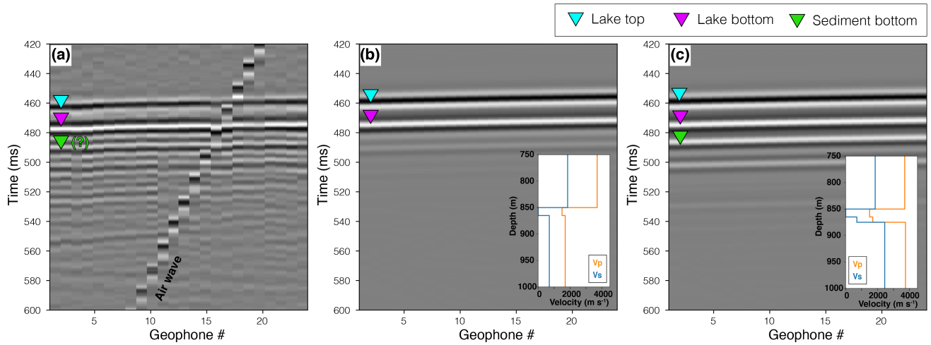
545 Figure 5. Observed (a) and synthetic (b and c) seismic data for shot gather 12 bandpass filtered between 50 – 200 Hz. The offset from the source to geophone 1 is 230 m. The colored triangles indicate reflections from the lake top (blue), lake bottom (purple), and sediment bottom (green). The insets in panels (b) and (c) show the V_P and V_S models that were used to compute the synthetics. Both models include a 12 m thick lake below 850 m of ice. The model used in (c) includes an additional discontinuity 10 m below the lake, which represents the boundary between the lake bottom sediments and underlying bedrock.
