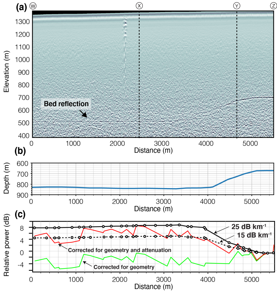
515 Figure 3. GPR profile. (a) shows the 5 MHz radar data, unmigrated. The primary bed reflection is marked with an arrow. Vertical dashed lines mark the approximate endpoints of the seismic survey. The depth from the surface to the base of the ice is shown in (b). In panel (c), the relative power of the basal reflections is shown after being corrected for geometric spreading (green line) and both geometric spreading and depth-average attenuation of -15 \text{ dB km}^{-1} (red line). The black solid and dashed lines show the magnitude of attenuation corrections assuming an englacial attenuation of -25 \text{ dB km}^{-1} and -15 \text{ dB km}^{-1} , respectively.
