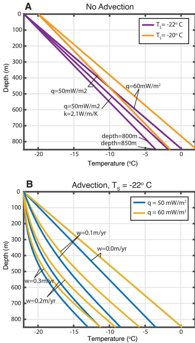
535 Figure 6. Modeled ice sheet thermal structure. Panel A shows thermal profiles neglecting advection for surface temperatures T_s = -22^\circ\text{C} and T_s = -20^\circ\text{C} , respectively. The basal heat flux q is varied between 50 – 60 \text{mW m}^{-2} and the accumulation rate w is varied between 0 \text{m yr}^{-1} and 0.3 \text{m yr}^{-1} .
