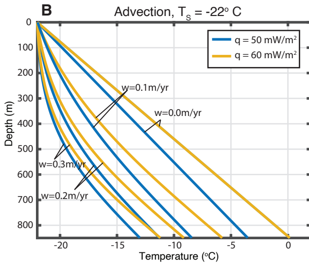
535 Figure 6. Modeled ice sheet thermal structure. Panel A shows thermal profiles neglecting advection for surface temperatures T_s = -22^{\circ}\text{C} and T_s = -20^{\circ}\text{C} . Panel B shows thermal profiles including advection for surface temperatures of T_s = -22^{\circ}\text{C} and T_s = -20^{\circ}\text{C} , respectively. The basal heat flux q is varied between 50 - 60\text{mW m}^{-2} and the accumulation rate w is varied between 0\text{m yr}^{-1} and 0.3\text{m yr}^{-1} .
