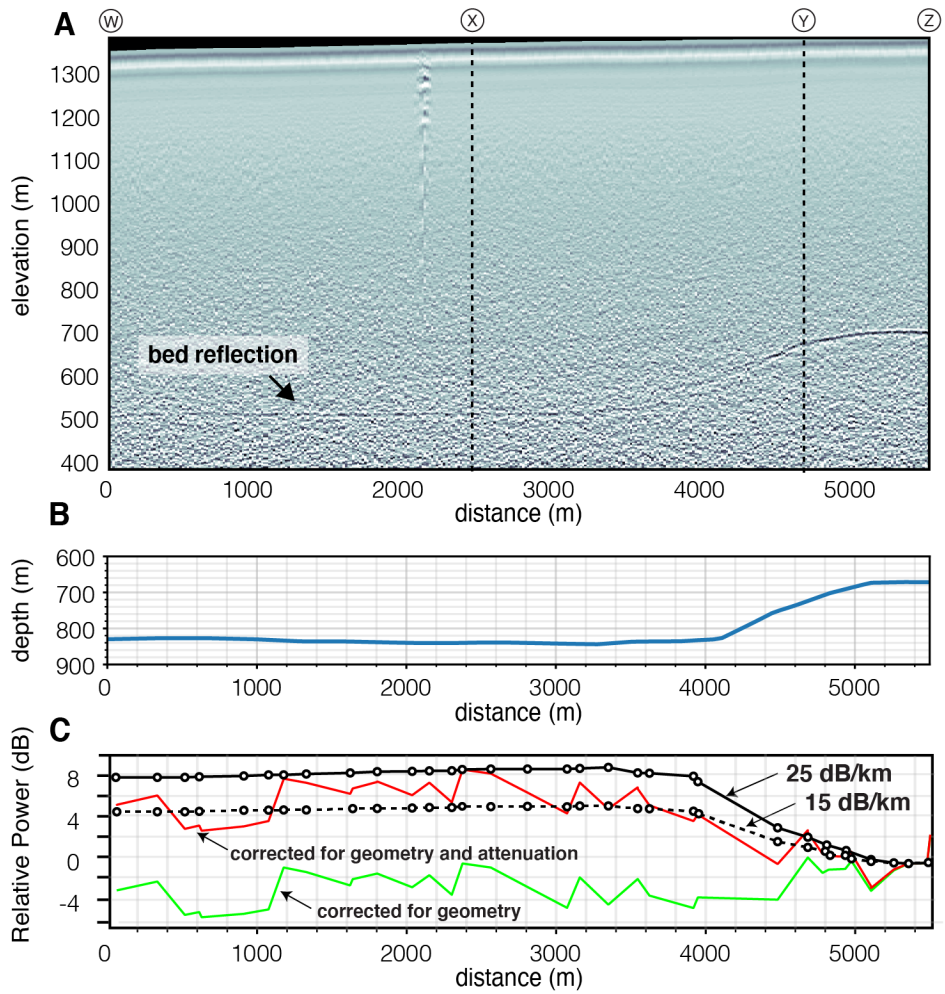
500 Figure 3. GPR profile. (A) shows the 5 MHz radar data, unmigrated. The primary bed reflection is marked with an arrow. Vertical dashed lines mark the approximate endpoints of the seismic survey. The depth from the surface to the base of the ice is shown in (B). In panel (C), the relative power of the basal reflections is shown after being corrected for geometric spreading (green line) and both geometric spreading and depth-average attenuation of -15dB/km (red line). The black solid and dashed lines show the magnitude of attenuation corrections assuming an englacial attenuation of -25 dB/km and -15 dB/km, respectively.
