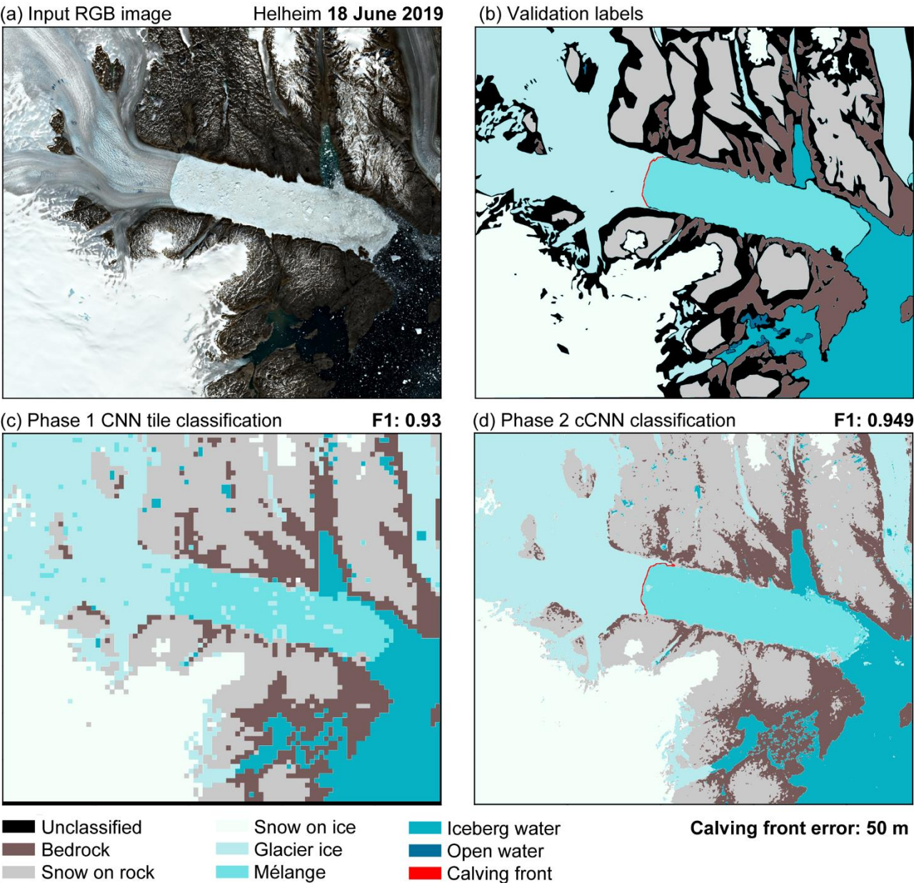
570 Figure 16: Example of CSC using Joint training for (a) an unseen image of Helheim acquired on 18 June 2019. (b) Shows the manually collected validation labels. (c) Shows the tiled output of the phase 1 CNN and (d) shows the final pixel-level classification with an associated calving front detection. The optimum classification parameters with a tile size of 50, patch size of 15 and RGB + NIR bands were used in this example.
