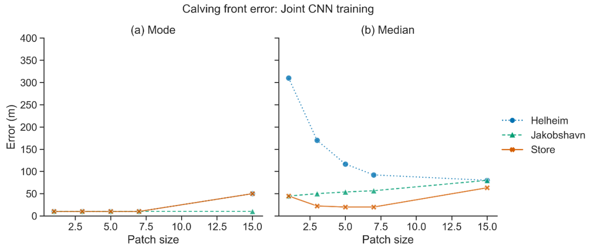
Figure 20: (a) modal and (b) median calving front error as a function of patch size for each glacier using Joint training.
