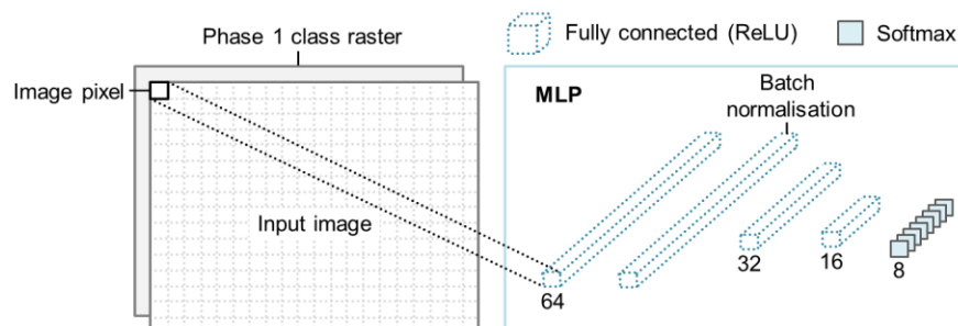
Figure 6: Architecture of phase two multilayer perceptron used for pixel-based classification.
