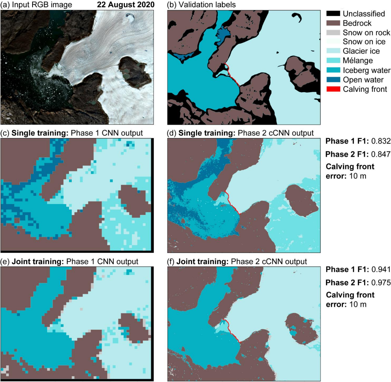
Figure 15: Comparison of Single and Joint training methods for (a) an image of Store glacier acquired on 22 August 2020. (b) shows the manually collected validation labels. (c) Shows the phase 1 tiled output using Single training and (d) shows the resulting CSC output. Note the area of glacier ice which has been misclassified using Single training. (e) Shows the phase 1 output using Joint training with the associated pixel-level phase 2 output shown in (f). A tile size of 50, patch size of 5 and RGB+NIR bands were used in the examples shown here. The Joint training method rectifies the misclassified area of glacier ice.
