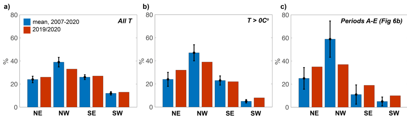
Figure 8. Percentage (%) of wind each season (1 November to 31 March) at Fossil Bluff AWS that is northeasterly (NE), northwesterly (NW), southeasterly (SE), southwesterly (SW), with the interannual (2007/2008 to 2019/2020) mean shown in blue and the 2019/2020 values shown in red. (a) Wind direction proportions using all recorded air temperatures. (b) Wind
