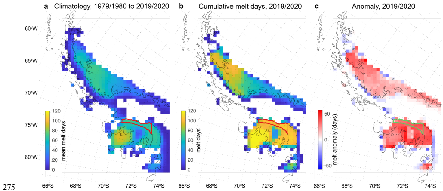
Figure 2. Microwave radiometer-derived maps of surface/near-surface melt days over the AP. (a) the climatology (i.e. mean cumulative melt days per season) from 1979/1980 to 2019/2020 (excluding 1987/1988 due to missing data); (b) cumulative melt days in 2019/2020; (c) the 2019/2020 melt season anomaly (i.e. (b) minus (a)). Melt days are counted within the period 1 November to 31 March (inclusive) each austral summer. The location of the study AOI is shown by a red outline in panels a) and b), and as a green outline in panel c). The black outline of the AP is from the MODIS Mosaic of Antarctica (Haran et al., 2014).
