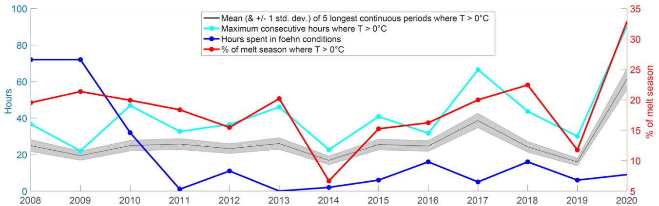
Figure 6. Analysis of sustained warm ( \geq 0^{\circ}\text{C} ) air temperature (T) periods and foehn wind occurrence for the 2007/2008 to 2019/2020 melt seasons. The cyan line shows the maximum number of consecutive hours in each melt season when T \geq 0^{\circ}\text{C} . The black line shows the mean length (hours) of the five longest periods when T \geq 0^{\circ}\text{C} for each season, with the grey shading indicating \pm 1 standard deviation from that mean. The red line shows the proportion of each season (1 November to 31 March) when T \geq 0^{\circ}\text{C} . The blue line shows the total number of hours spent in a foehn condition (see Section 3.4 for definition) each season. The x-axis dates indicate the second year of each austral summer, e.g., 2020 corresponds to the 2019/2020 season.
