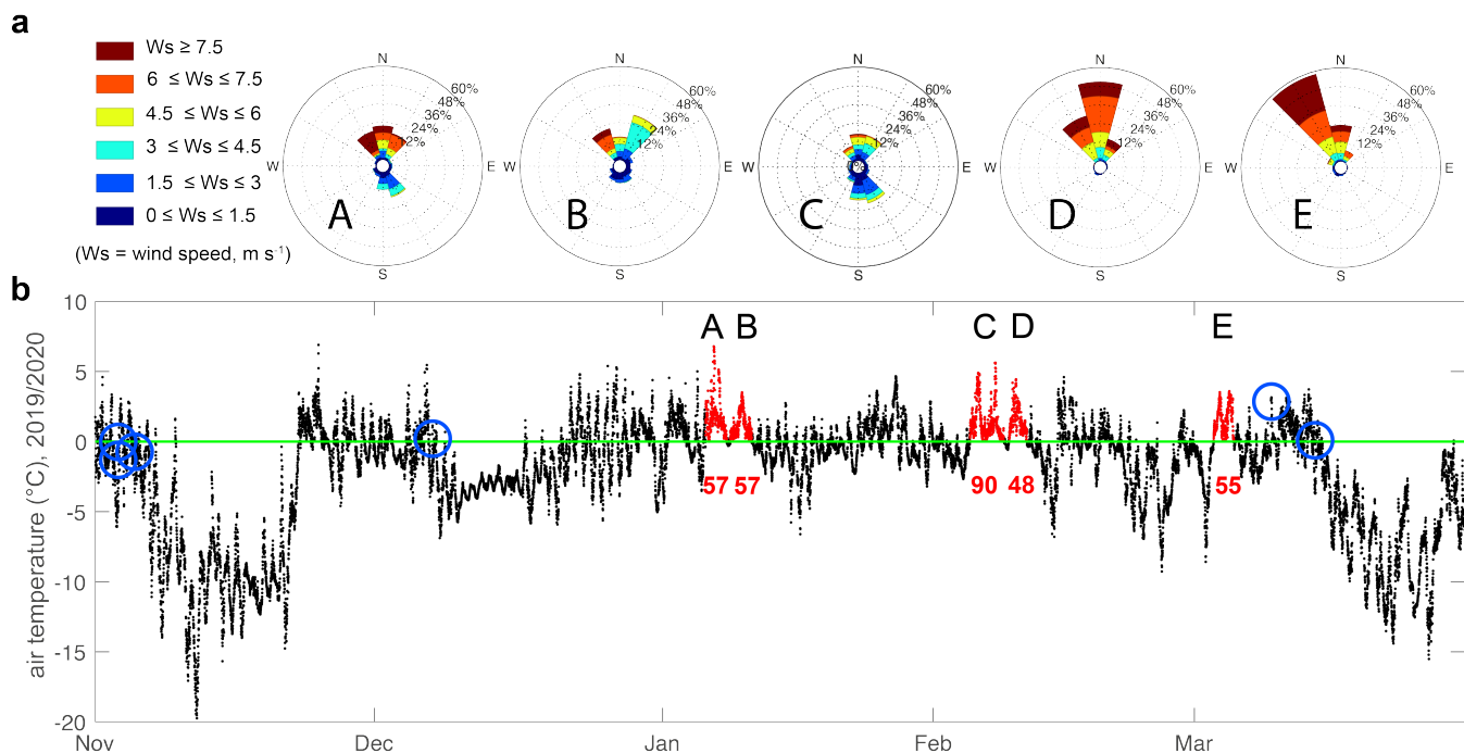
Figure 7. 2019/2020 wind and air temperature and data (10 minute) from the Fossil Bluff AWS. (a) Wind roses for corresponding periods of sustained air temperatures (A-E) indicated in b. (b) Air temperature record for 2019/2020 with the five longest periods of temperatures \geq 0^\circ\text{C} shown in red. The red numbers below these time periods indicate the total number of hours when the temperature is continuously \geq 0^\circ\text{C} . It is notable that only 9 hours separate periods A and B, and only 14 hours separate C and D. The six blue circles indicate periods when we calculate foehn conditions to be present (see Section 3.4 for methods).
