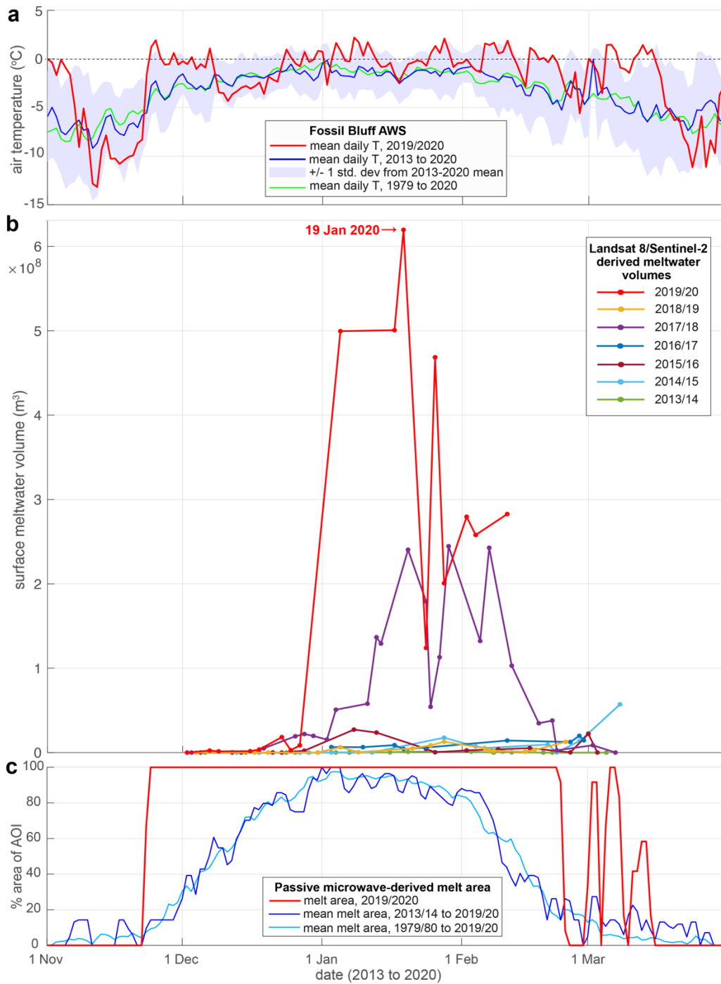
360 Figure 5 (a) Surface (2 m) air temperature data from the Fossil Bluff AWS (location in Fig. 1b, yellow star). The daily mean air temperature for the 2019/2020 melt season is shown by the red line, the daily mean temperature for the seven melt seasons from 2013/2014 to 2019/2020 are shown by the blue line, +/- one standard deviation from that blue line is shown by the areas
