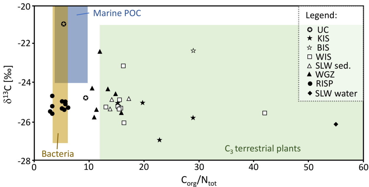
Figure 3: \delta^{13}C plotted against C_{org}:N_{tot} (atom:atom). Shaded areas taken from Lamb et al. (2006). Although the RISP and WGZ samples are from a sub-ice shelf cavity, RISP is located mid-ice shelf whereas WGZ is located within the grounding zone. The UC samples are sediments melted out from basal ice, as opposed to collected below ice or an ocean cavity.
