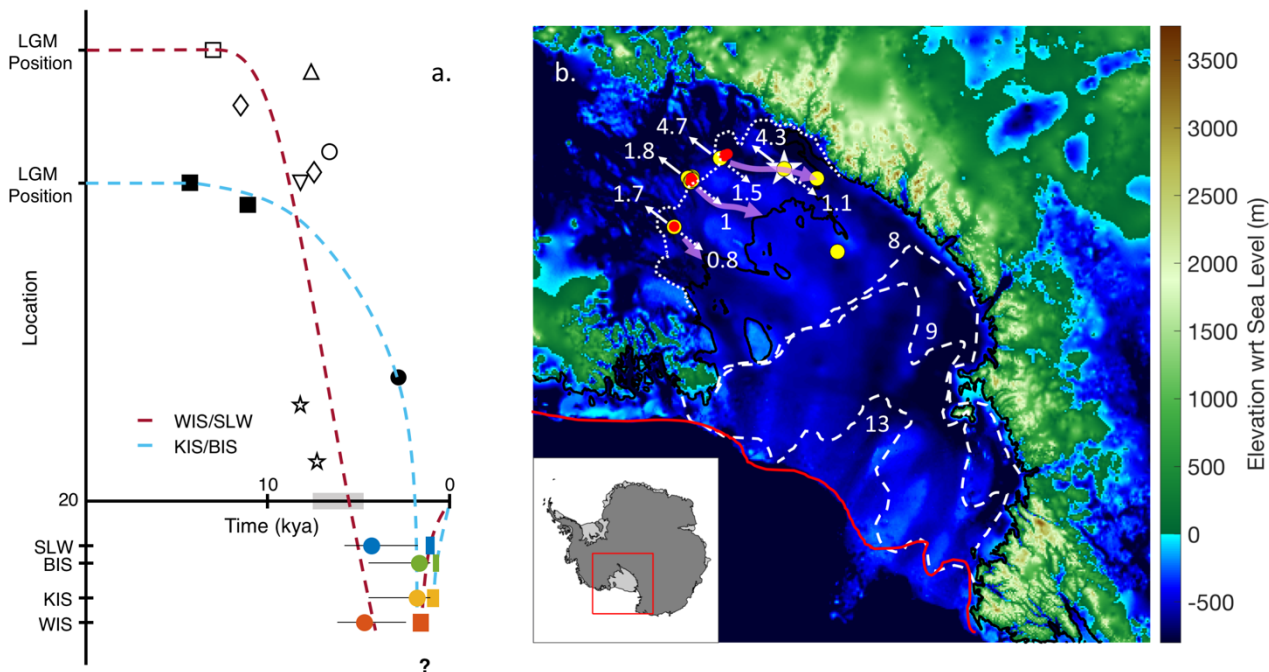
930 Figure 9: The evolution of grounding line positions in the Ross Embayment for the past 20,000 years. (a) Schematic for grounding 935 line position along the flow lines of the Whillans Ice Stream (maroon dashed line) as well as the Bindschadler Ice Stream and 940 Kamb Ice Stream (blue dashed line). The colored dots represent the optimal grounding line retreat timing (error indicated by thin 945 black lines) seen in Fig. 8. The colored bars represent the optimal timing of grounding line readvance (between the 32 nd and 68 th Baroni and Hall (2004) (right side up empty triangle), Bart et al. (2018) (solid square), Conway et al. (1999) (solid circle), Cunningham et al. (1999) (empty square), Jones et al. (2015) (empty circle), Licht et al. (1996) (empty diamond), McKay et al. (2016) (upside down empty triangle), Spector et al. (2017) (empty star). Open symbols represent ages along/near the flowline of the Whillans Ice Stream, and solid symbols represent ages along the flowline of the Bindschadler Ice Stream. Gray bar along the grounding line represents grounding line retreat at WGZ calculated in Venturelli et al. (2020). (b) Map-view of Holocene grounding line positions in the Ross Embayment. Background image is bed elevation (Fretwell et al., 2013). Yellow dots denote the location of sediment cores taken for radiocarbon and TOC analysis. Red dots denote the location of deep temperature profiles examined in this study. Cyan diamond indicates the location where sediment porewater was collected and analyzed. Red line indicates LGM grounding line position (Bentley et al., 2014). Dashed white lines indicate grounding line retreat from Lee et al. (2017). The corresponding numbers indicate timing in kya (thousands of years). Dotted white line shows most retreated grounding line position modelled in Kingslake et al. (2018). Solid white arrows indicate timing of grounding line retreat in kya, and dotted white arrows indicate timing of grounding line readvance over those sites. Thick purple arrows indicate flowlines along the Whillans, Kamb, and Bindschadler Ice Streams.
