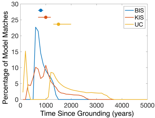
890 Figure 5: Results of temperature diffusion modelling. The y-axis represents the frequency at which the modelled basal temperature gradients fit within 10% of the observed basal temperature gradients (Engelhardt, 2004). The number of observed basal temperature gradients varied between the sites: one observation for BIS, four observations for KIS, and three observations for UC. The dots and lines in the upper portion of the figure correspond to the median and the 32 nd to 68 th percentiles of the distributions shown in the lower portion of the figure. The total number of model runs performed was 808,000, corresponding to a time window of 8000 years ago to present.
