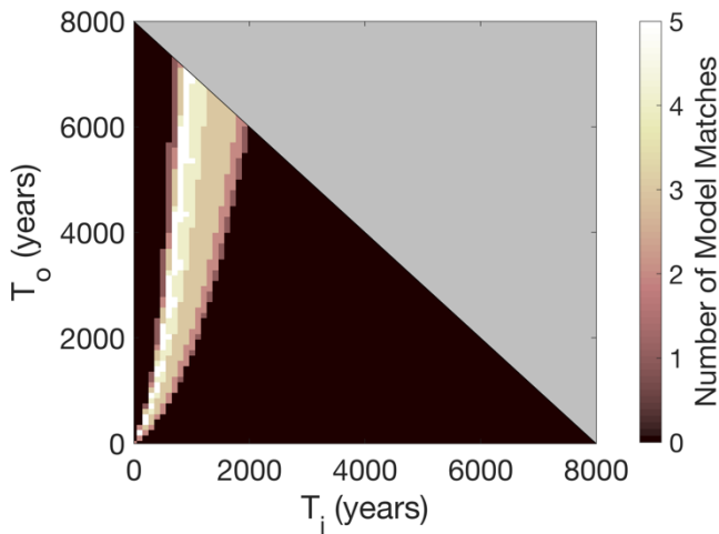
895 Figure 6: Stacked results from ionic diffusion modelling of all six chemical parameters. T_o represents the length of time over which the topmost sediment was exposed to ocean water after initial grounding line retreat and before grounding line readvance. T_i represents the length of time over which the topmost sediment was exposed to subglacial conditions between the grounding line readvance over SLW and now. The number of model runs included in this figure is 19,926.
