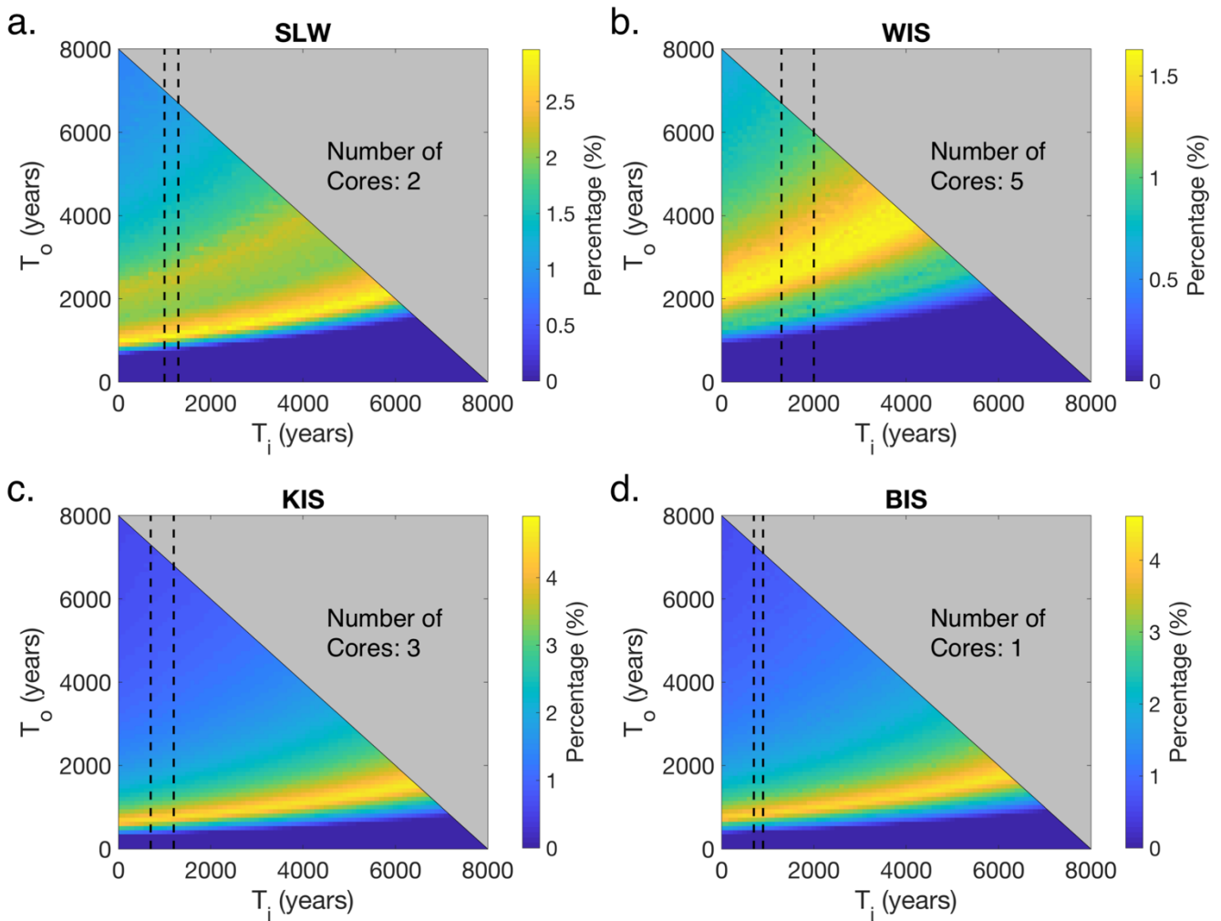
900 Figure 7: Results of radiocarbon modelling for all eleven subglacial cores. The axes correspond to the length of time the grounding line position had either retreated behind the sites ( T_o ) or advanced over them ( T_i ). The colorbar indicates the percentage of model runs which produced F_m and TOC that fell within the observed ranges for each core. A total of 103,495,644 model runs were performed for each core. Results from cores at the same field site are stacked on top of each other. Thus, the total number of model runs for each site is 206,991,288 for SLW, 517,478,220 for WIS, 310,486,932 for KIS, and 103,495,644 for 905 BIS. The large number of model runs (which serve as the denominator in calculations of percentage of model matches) are responsible for the relatively small percentages shown in a-d. (a) SLW (b) WIS (c) KIS (d) BIS. a-d indicate that the model provides better constraint to T_o than T_i . For example, (c) shows that at KIS, the model prefers ocean exposure durations ( T_o ) of 600-1800 years but does not constrain the duration of grounding line readvance ( T_i ). The dashed lines indicate the 32 nd and 68 th percentiles from the results of the duration of T_i as determined by ionic and temperature diffusion modelling.
