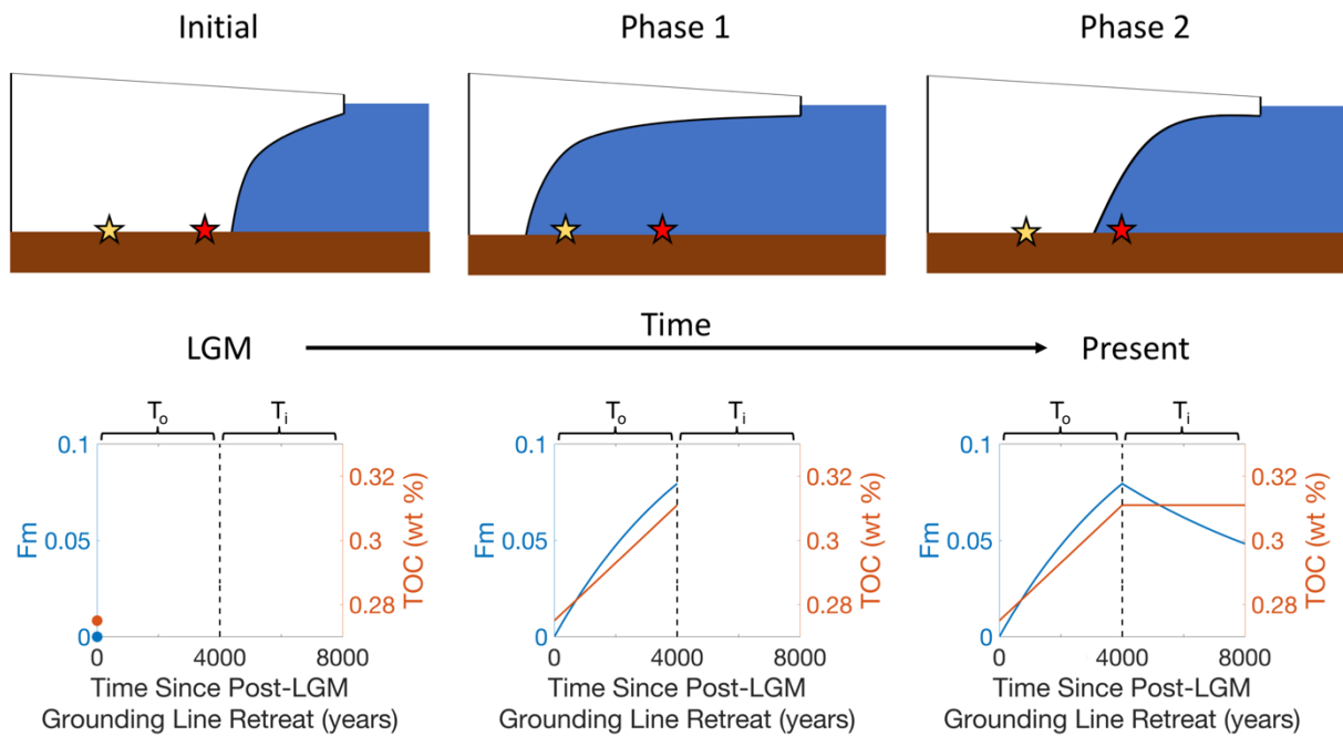
880 Figure 4: Schematic of the two-phase model of radiocarbon evolution since onset of LGM grounding line retreat over the field sites. The yellow star represents subglacial field sites, whereas the red star represents sub-ice shelf sites. The evolutions of Fm and TOC are shown for subglacial field sites. For this run, both T_o and T_i equal 4000 years; the horizontal axis represents time since post-LGM grounding line retreat past a subglacial site (yellow star). Ocean exposure (when the grounding line had retreated beyond a site) begins at t = 0 and is assumed here to last until t = 4000 years. Subsequent grounding line readvance occurs at t = 885 t = 4000 years and lasts until the end of the model run ( t = 8000 years). Accumulation rates for ^{14}C and ^{12}C were assumed to be 9.23 \times 10^{-18} g/yr and 9.0 \times 10^{-6} g/yr per 100 grams of dry sediments, respectively. Note that the right-hand side axis (TOC) does not start at zero.
