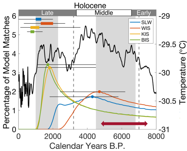
915 Figure 8: The estimated timing of grounding line retreat and readvance compared to selected climate data for the study region. 920 The colored lines (which correspond to the left y-axis) represent the probability distribution of the timing of grounding line retreat ( T_o + T_i ) for each subglacial field site. The lines are calculated by summing T_o and T_i from the model matches in between the dashed lines of the radiocarbon model results shown in Fig. 7. The dots on the peaks of the distributions indicate the optimal timing of grounding line retreat, and the thin black lines indicate the estimate on error. The box and whisker plots in the upper left corner indicate the timing of grounding line readvance over our field sites ( T_i ) estimated from temperature and ionic diffusion modelling. The thick black line (which corresponds to the right y-axis) represents the Holocene history of surface temperature at WAIS Divide (Cuffey et al., 2016; Cuffey, 2017). The gray vertical shaded regions indicate the warm periods of less extensive sea ice in the Western Ross Sea proposed by Hall et al. (2006), and the gray dashed lines bracket the period of Ross Sea warming identified by Cunningham et al. (1999). The maroon arrow indicates the estimated range of grounding line retreat over WGZ based on the ramped-pyrolysis method (Venturelli et al., 2020).
