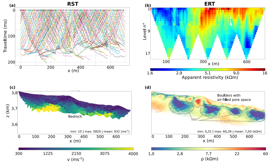
Figure 6. Geophysical observations and inversion model results for El Jote rock glacier. (a) RST first arrival traveltimes. (b) ERT apparent resistivity. (c) Velocity and (d) resistivity tomograms. The velocity model is cut below the lowermost ray-path while the resistivity model transparency is proportional to the ERT data coverage. The velocity colorbar is linear, while the resistivity one is expressed in logarithmic scale.
