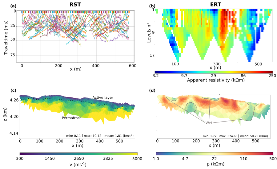
Figure 8. Geophysical observations and inversion model results for El Ternero rock glacier. (a) RST first arrival traveltimes. (b) ERT apparent resistivity. (c) Velocity and (d) resistivity tomograms. The velocity model is cut below the lowermost ray-path while the resistivity model transparency is proportional to the ERT data coverage. The velocity colorbar is linear, while the resistivity one is expressed in logarithmic scale.
