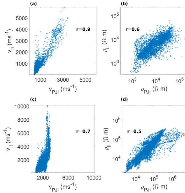
Figure 10. Correlation of P-waves velocity and resistivity model results between individual dataset inversion (II) and petrophysical joint inversion (PJI). (a) El Jote P-waves velocity and (b) resistivity model values; (c) El Ternero P-waves velocity and (d) resistivity model values. In each figure is indicated the correlation coefficient r .
