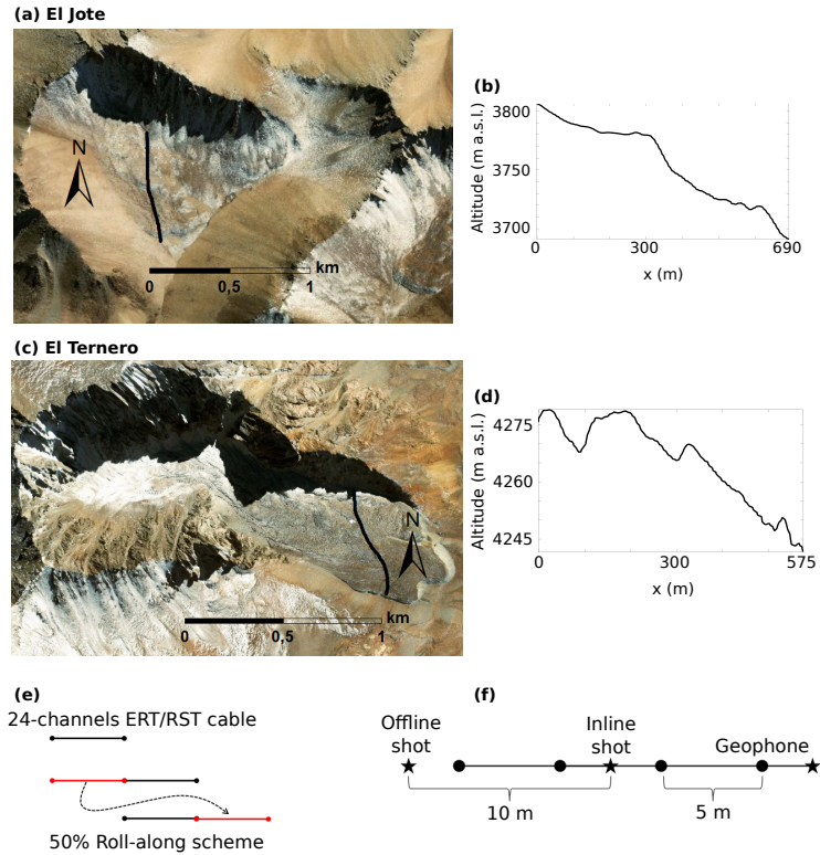
Figure 4. (a) Aerial image of El Jote, showing the location of the geophysical survey line and (b) its topography from field differential GPS measurements. (c) Aerial image of El Ternero, showing the location of the geophysical survey line and (d) its topography from field differential GPS measurements. Base maps in (a) and (c) from Esri World Imagery 2018. (e) Scheme of the 50% roll-along scheme used for ERT surveys on both rock glaciers and RST survey on El Jote. (f) Scheme of geophones and Inline/Offline shot positions for RST surveys.
