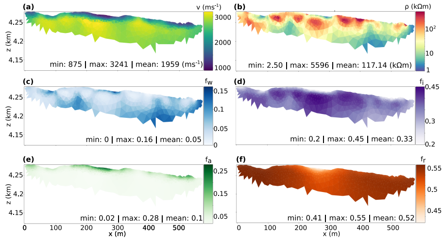
Figure 9. Petrophysical joint inversion results of El Ternero field data sets. The tomograms represents (a) velocity and (b) resistivity transformed models. The directly inverted parameters are (c) water, (d) ice, (e) air and (f) rock volumetric content. All models are cut off below the lowermost ray path, with only resistivity colorbar expressed in logarithmic scale.
