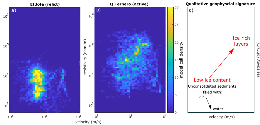
Figure 11. Density plots of resistivity versus P-waves velocity values for (a) El Jote and (b) El Ternerro datasets. (c) Schematic plot of the qualitative ERT and RST signature for intact and relict rock glaciers. The model cells involved in this analysis are inside the modeled grid, where there are raypaths and resistivity sensitivity
