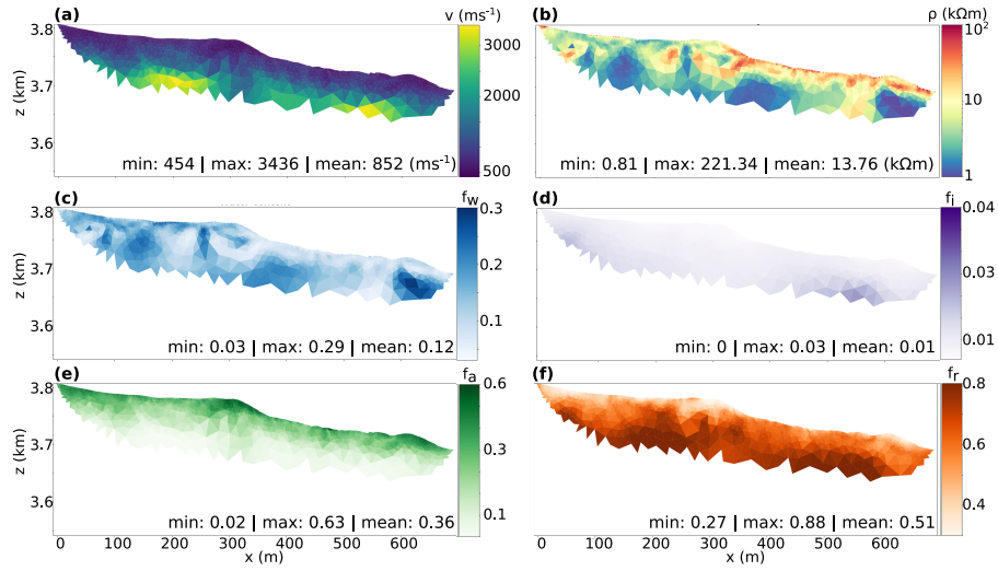
Figure 7. Petrophysical joint inversion results of El Jote field data sets. The tomograms represents (a) velocity and (b) resistivity transformed models. The directly inverted parameters are (c) water, (d) ice, (e) air and (f) rock volumetric content. All models are cut off below the lowermost ray path, with only resistivity colorbar expressed in logarithmic scale.
