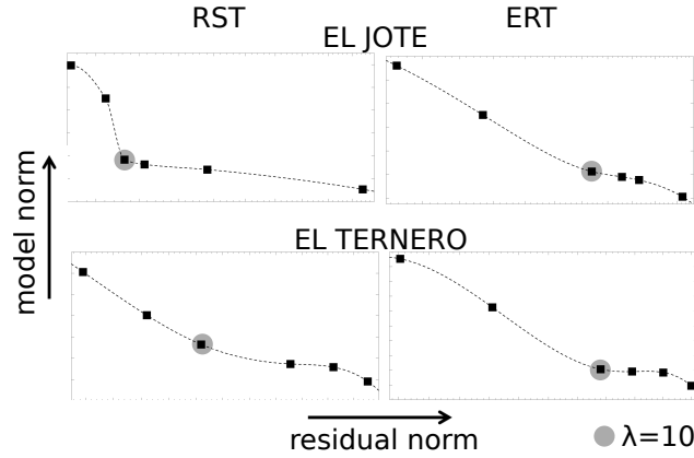
Figure 3. L-curve analysis for the regularization weights ( \lambda ) used in the inversion of ERT and RST data on both rock glaciers. In each plot, the values tested are \lambda = 1, 5, 10, 15, 50, 100 .
