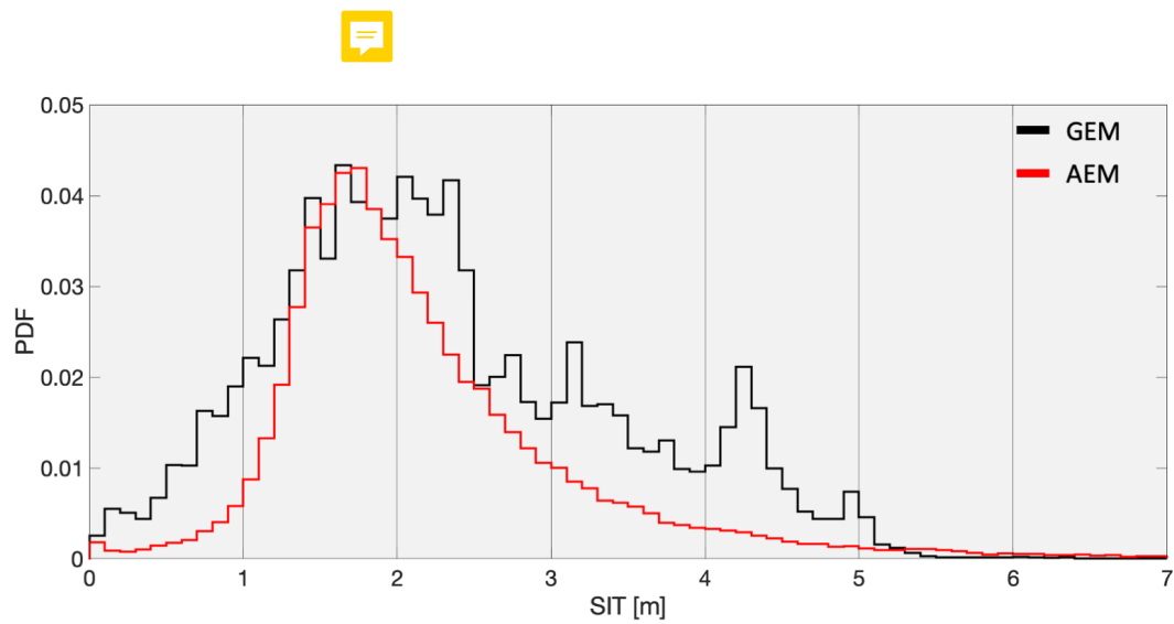
Figure S2. Comparison of MOSAiC floe sea ice thickness distribution gathered with the ground-based EM (GEM) between July 16 to July 27, 2020 (black) and airborne EM (AEM) derived sea ice thickness distribution (red) of the floe and wider area (radius about 5 km around the floe) from July 1 and July 7, 2020.
