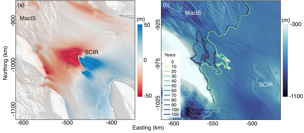
Figure 11. (a) The total change in ice thickness 150 years after removal of the SCIR. Red indicates thinner ice and blue indicates thicker ice without the ice rumpled. (b) Retreat of a section of the simulated MacIS grounding line ( \bar{B}_{inv} case) following removal of the SCIR plotted on the subglacial bed elevation (Fretwell et al., 2013).
