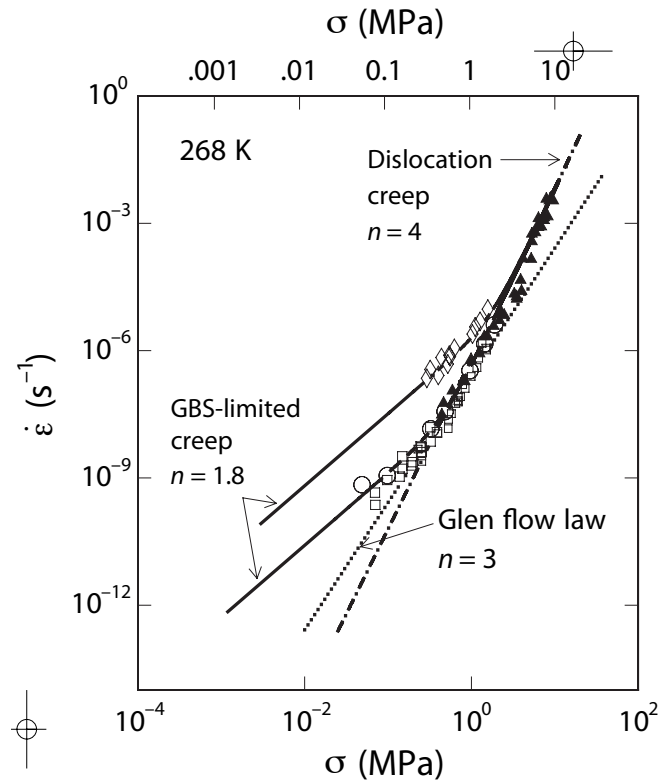
Figure 1. Strain-rate versus stress compiled from laboratory experiments on coarse-grained ice revealing the existence of the 720 dislocation creep regime ( n=4 ) and GBS-limited creep regime ( n=1.8 ) at high and low stress, respectively. The upper and lower solid lines show grain boundary sliding flow law calculated for grain sizes of 0.2 and 2 mm, respectively; dashed-dot line shows dislocation creep flow law; dotted line depicts the Glen Law. Data are from ambient pressure tests at 268 K: d = 0.2 mm (diamonds) (Goldsby & Kohlstedt, 2001); d \geq 1 mm (squares) (Steinemann, 1958); d \geq 1 mm (circles) (Mellor & Smith, 1966); d \geq 1 mm (triangles) (Barnes et al. 1971). Note that the Glen law fails to adequately describe the flow of ice over 725 a wide range of stresses. Figure adapted from Goldsby (2006).
