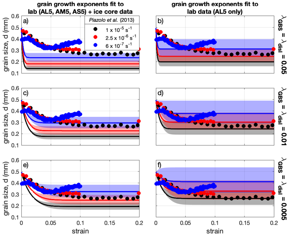
Figure 5. Comparison of wattmeter to experimental data on grain size evolution from Piazolo et al. (2013). Calculations are performed assuming a shear zone with an imposed strain rate corresponding to the laboratory experiments ( 1 \times 10^{-5} \text{ s}^{-1} black; 2.5 \times 10^{-6} \text{ s}^{-1} red; 6 \times 10^{-7} \text{ s}^{-1} blue). Initial grain size is set to 0.5 mm and grain size evolution is calculated as a function of time/strain using Eq. (13). Panels (a,c,e) show results using the grain growth parameters from the joint fit between the laboratory and ice core data (black line in Fig. 2); panels (b,d,f) show results using the grain growth parameters from Azuma et al. (2012) experiment AL5. Rows indicate calculations using different values for \lambda = \lambda_{GBS} = \lambda_{disl} ranging from (a,b) 0.05, (c,d) 0.01, and (e,f) 0.005.
