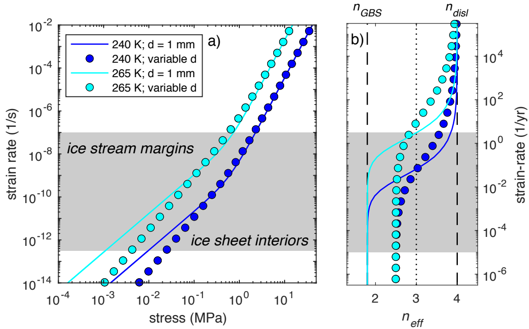
Figure 4. (a) Comparison of strain rate vs. stress predicted for a constant grain size of 1 mm (colored lines) to those predicted by the steady-state grain size calculated from the wattmeter (colored symbols). Dark blue and light blue colors correspond to temperatures of 240 K and 265 K, respectively. Wattmeter calculations correspond to those shown in Fig. 3 for a shear zone of fixed width. (b) Effective stress exponent as a function of strain-rate predicted from the model. The effective stress exponent is calculated from the slope of the strain-rate vs. stress curve shown in panel (a). For cases with a fixed grain size, the stress exponent transitions from the experimentally-derived value for GBS-limited creep (at low strain rate) to the value for dislocation creep (at high strain rate). The effective stress exponent in the GBS-limited creep regime calculated from the wattmeter is higher than the experimentally-determined value and remains closer to the Glen law value of \sim 3 for strain rates typical of natural systems.
