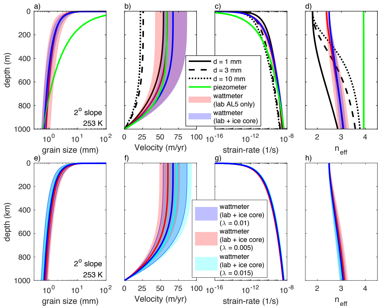
795 Figure 6. (a) Steady-state grain size, (b) velocity, (c) strain-rate, and (d) the effective stress exponent, n_{eff} calculated as a function of depth. The effective stress exponent is calculated from our model using the local gradients in stress and strain rate. Red and blue curves correspond to calculations using the grain growth parameters from Azuma et al. (2012) experiment AL5 and the joint fit of the experimental and ice core data, respectively; shading denotes error bounds based on uncertainty in fit of the grain growth data. Black curves show calculates constant grain sizes of 1 mm (solid), 3 mm (dashed), and 10 mm (dotted). Green curve shows calculations based on the piezometer of Jacka & Li (1994). Note that the effective stress exponents calculated using the wattmeter fall in a range similar to the Glen law ( n_{eff} = 2.5-3 ). (e-h) Same as panels a-d, but comparing cases using different values for \lambda = \lambda_{GBS} = \lambda_{disl} . 800
