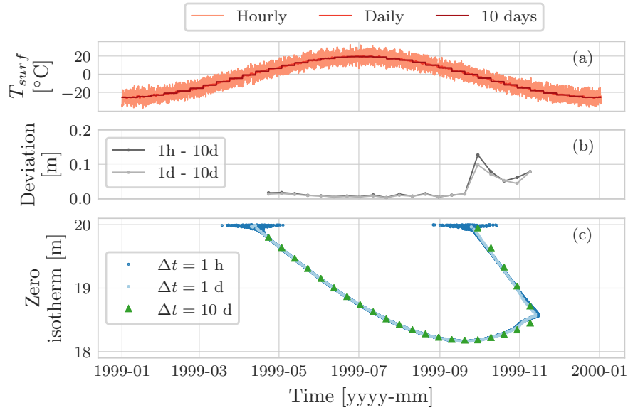
Figure 11. Comparison of the position of the zero-isotherm, panel (c), after 100 years of three simulations: using an hourly boundary condition with time step of \Delta t = 1 \text{ h} , using a daily boundary condition with a time step of \Delta t = 1 \text{ day} , and a 10-day boundary condition with a time step of \Delta t = 10 \text{ day} . Panel (a) shows the surface temperature for the hourly, the daily and the 10-days simulations. Panel (b) shows the deviation of the position of the zero-isotherm after 100 years between the hourly and the 10-days simulation, and between the daily and the 10-days simulation.
