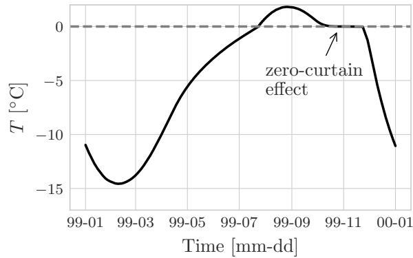
Figure G3. Hourly temperature at 1.5 m depth for the year 1999. Note the prolonged period of 43 days (11 October until 23 November) when temperature remained within \pm 0.1 ^{\circ}\text{C} . This is the so-called zero-curtain effect, and it is due to latent heat of fusion that is continually released during the freezing of soil moisture.
