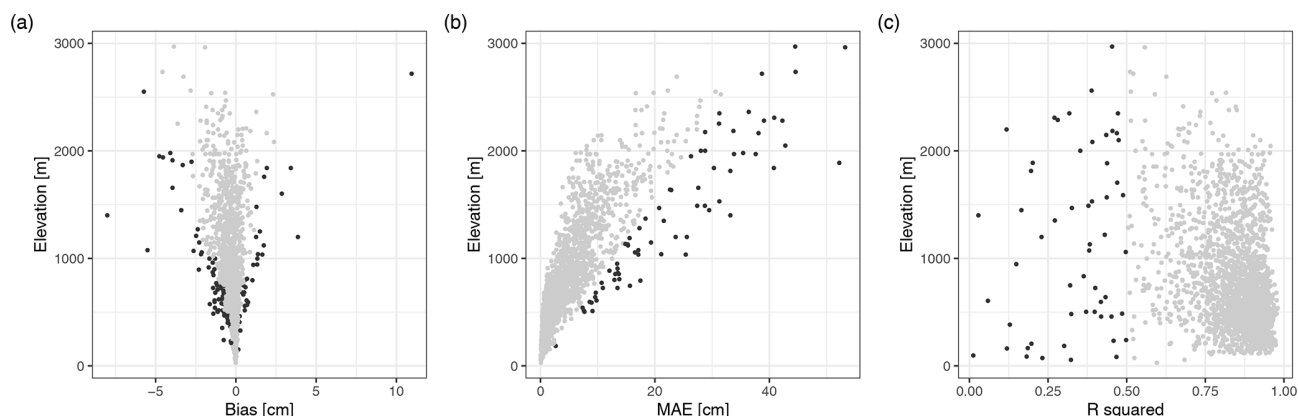
Figure A4. Metrics for spatial consistency: (a) bias, (b) mean absolute error (MAE), and (c) R^2 TS7 (squared correlation). Metrics were derived from statistical simulations of the monthly series from December to February using spatial neighbours. Black points indicate stations which were further analysed with manual checks.
