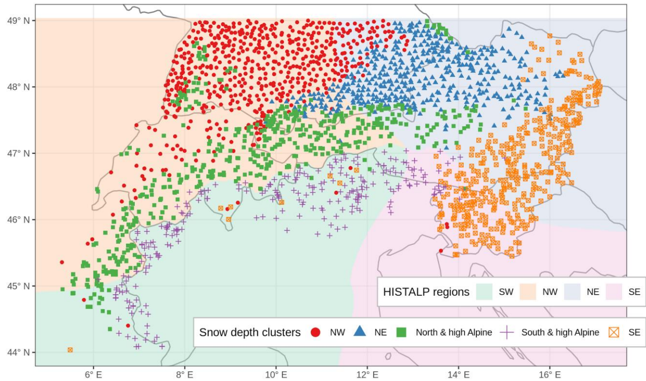
Figure 5: Clustering of stations based on daily snow depth data. Map of regions from applying a k-means clustering on the first five principal components. Underlaid are the HISTALP coarse resolution subregions (Auer et al., 2007), which were derived using a semi-automatic principal component analysis of climate variables (temperature, precipitation, air pressure, sunshine, and cloudiness).
