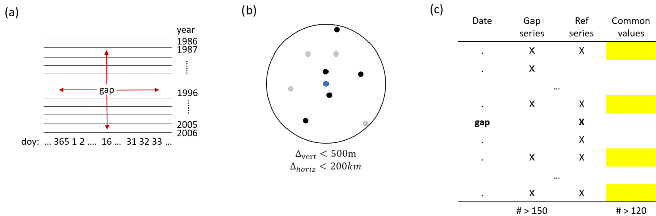
755 Figure A2: Visualization of some steps of gap filling algorithm. (a) shows how the window data in the gap series around the gap is determined (step 1.); day is day-of-the-year. (b) shows the selection of potential reference series by horizontal and vertical distance (step 2.). (c) shows how common dates for gap and reference series are identified (step 3.); the dates come from the window in (a).
