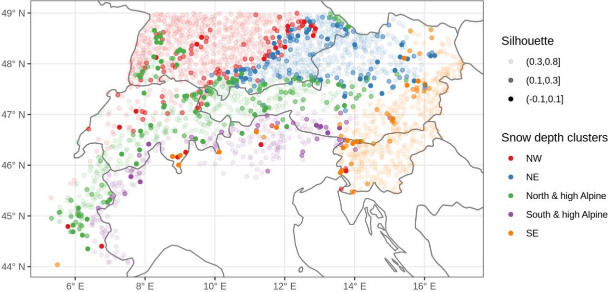
870 Figure B1: Silhouette values of the stations, which show consistency of clustering. The silhouette is a measure of how similar the station is to its own cluster compared to the other clusters (see methods for formula). High values indicate a good match, while low and negative values indicate a poor match.
