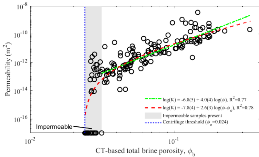
Figure 7. Relationship of simulated vertical permeability K and the total brine porosity \phi . Two log-log fits are drawn and specified in the legend, one for K(\phi) shown as corresponding to power laws of the form K = a(\phi)^b (green curve), one for K(\phi - \phi_c) and K = a(\phi - \phi_c)^b as red curve. The grey shading indicates the regime where permeable and impermeable samples are found. The numbers in brackets are the uncertainties in the last decimal of the log-log least square fit. The grey shading indicates the regime where permeable and impermeable samples are found.
