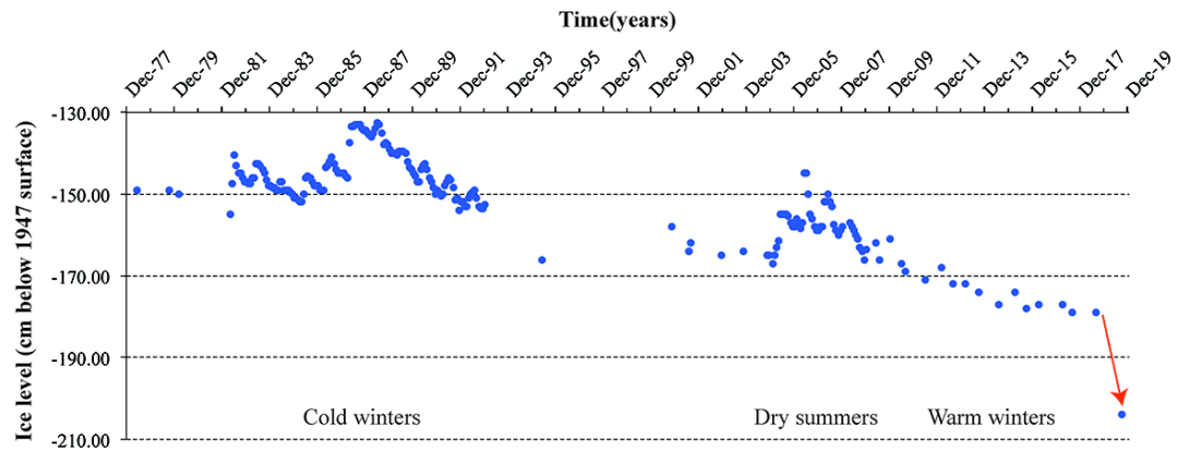
490 Figure 2: Upper surface ice level changes of the glacier in Scărișoara Ice cave, Romania, between 1975 and 2019. The red arrow points to the unprecedented annual melt in 2019.
