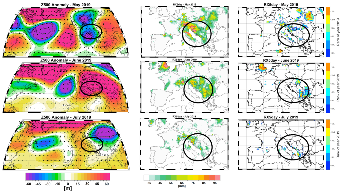
540 Figure 7. Left column: Geopotential height anomalies at 500mb level (Z500) [a) May 2019; d) June 2019 and g) July 2019]; Middle column - Highest 5-day precipitation amount (RX5day) [b) May 2019; e) June 2019 and h) July 2019] and right column – Top-six ranking of 2019 monthly RX5day [c) May 2019; f) June 2019 and i) July 2019]. A score of 1 represents the wettest month since 1950, a score of 2 represents the second wettest, and so on; all ranks greater than 6 are shown in white. Analyzed period: 1950–2015. For the Z500 the anomalies are computed relative to the period 545 1971 – 2000. Black ellipses indicate the study area.
