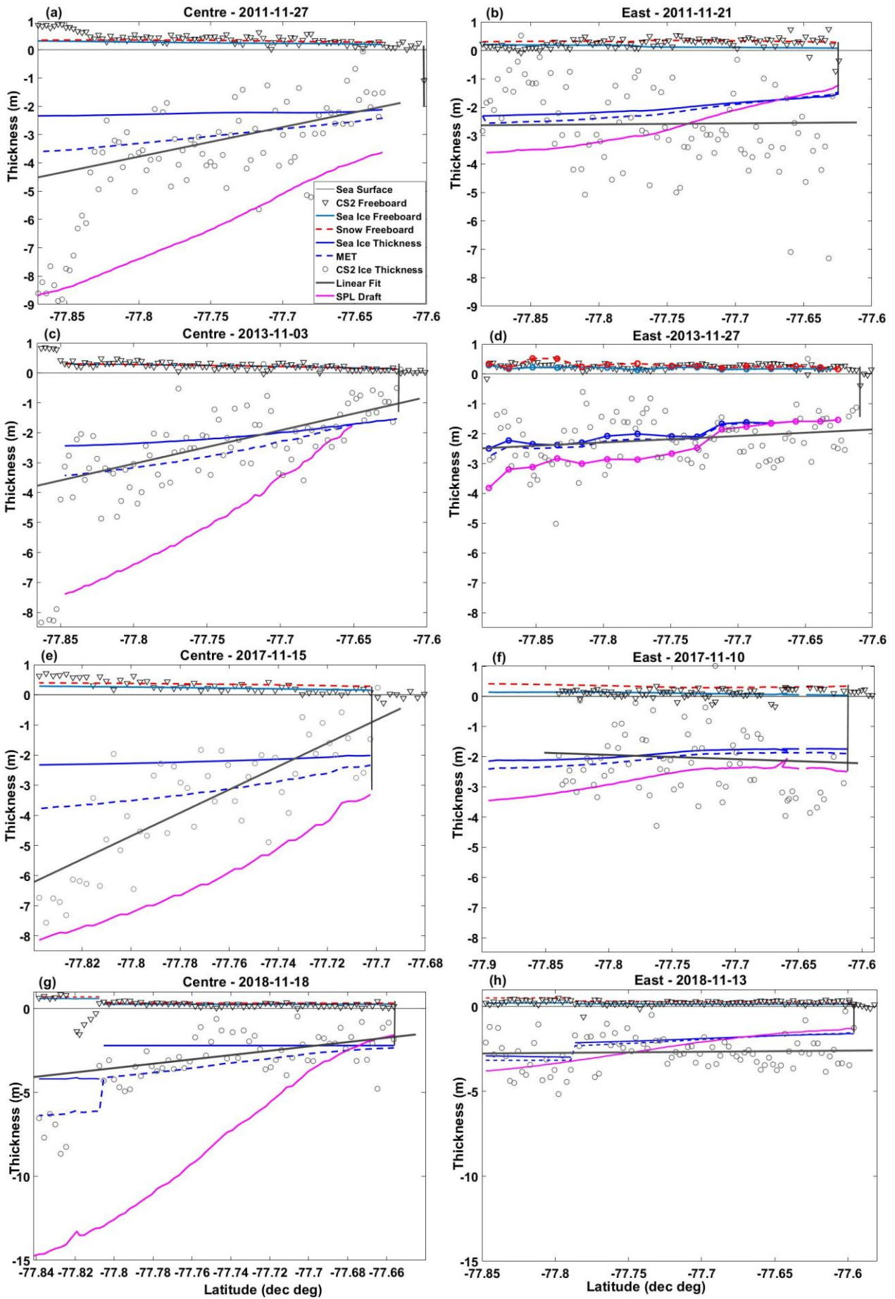
480 Figure 4: Comparison of along-track profiles of CS2 freeboard and CS2 ice thickness in the centre (a, c, e, and g) and east (b, d, f and h) for 2011, 2013, 2017 and 2018. The McMurdo Ice Shelf is located in the south (left) of all profiles. Linear fits applied to CS2 ice thickness (over first-year ice only) are shown with interpolated drill hole sea ice and SPL thicknesses, MET and sea ice and snow freeboard. A drill hole validation line was carried on along the eastern CS2 track on the 27 th November 2013 by Price et al. (2015) and drill hole measured snow and sea ice freeboard, sea ice and SPL thickness, and MET are included in (d) (circles).
