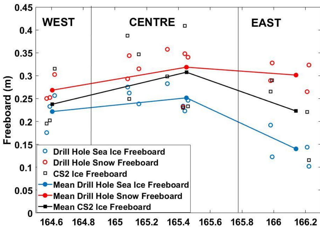
410 Figure 3: Comparison of all drill hole measured sea ice and snow freeboards with CS2 freeboard over first-year fast ice only for the 3 tracks in the west, 7 in the centre and 4 in the east (refer to Fig. 1 for locations and values given in Table 1). The mean regional values for the tracks in the west, centre and east are shown with a solid line to illustrate the mean freeboard distribution across McMurdo Sound. The longitudes are taken from where each CS2 track crossed latitude 77.7°S.
