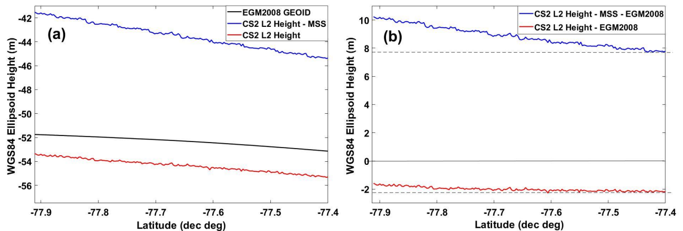
Figure A1: Comparison of CryoSat-2 heights from the Level 2 SIN-InSAR product and the effects of de-trending with the Earth Gravitational Model 2008 (EGM 2008) geoid (Pavlis et al., 2012) over 55 km of open ocean in McMurdo Sound on 17 March 2011. (a) Surface 1 : CS2 height with the MSS applied and all ocean corrections applied (red); Surface 2 : CS2 height with the MSS removed and all ocean corrections applied (blue); and Surface 5 : EGM 2008 surface (black). (b) CS2 height with the MSS removed and de-trended for the EGM 2008 geoid (blue), and Surface 6 : CS2 height with the MSS applied and all ocean corrections applied and then de-trended for the EGM 2008 geoid (red). All heights are given relative to the WGS84 ellipsoid. Dashed horizontal lines are included in b to highlight the different gradients in the profiles.
