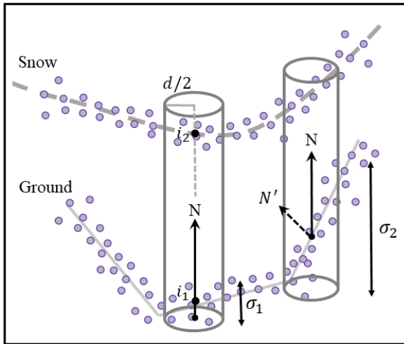
640 Figure B1: M3C2 method for computing snow depth. Vector N shows the normal on the reference surface (ground) and d is the projection scale. Surface roughness is the standard deviation of the point clouds within the cylinder ( \sigma ). Misorientation on rough surfaces ( N' ) is seen by high standard deviation ( \sigma_2 ) and is resolved by choosing the proper normal scale. Snow depth is the vertical distance between the average positions of ground and snow point clouds within the cylinder (distance between i_1 and i_2 ). Redrawn from Lague et al., 2013.
