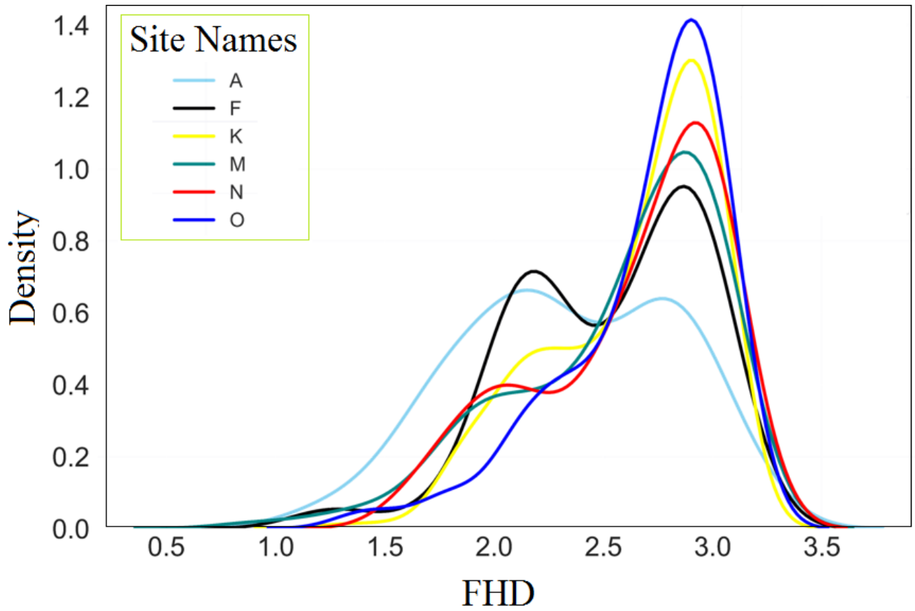
650 Figure B3: Foliage Height Diversity (FHD) distribution for each site.
