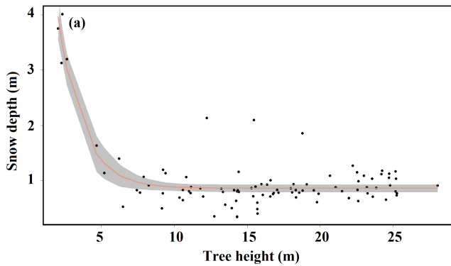
600 Figure 10: Tree height and snow depth within the 10 m transition zone in the south direction for (a) site A and (b) site K. The exponential and linear fit is shown with a red line along with 95 % confidence interval (grey).
