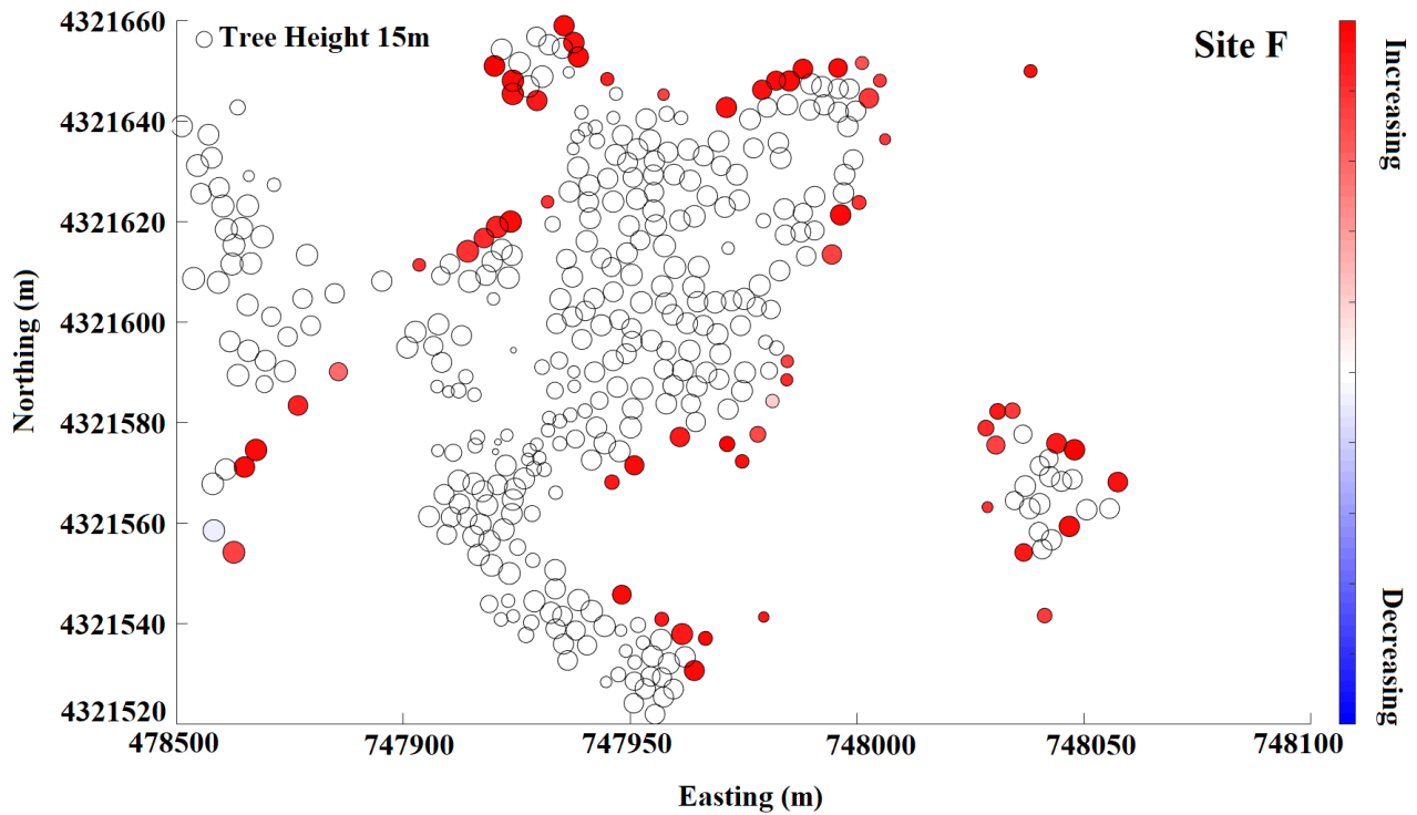
Figure B5: Snow depth change within a 10 m buffer from the edge of a tree at site F. Red color indicates snow depth increases moving from the tree edge toward the open and blue indicates snow depth decreases. Increasing and decreasing patterns are shown for individual trees at each site with adequate snow coverage.
