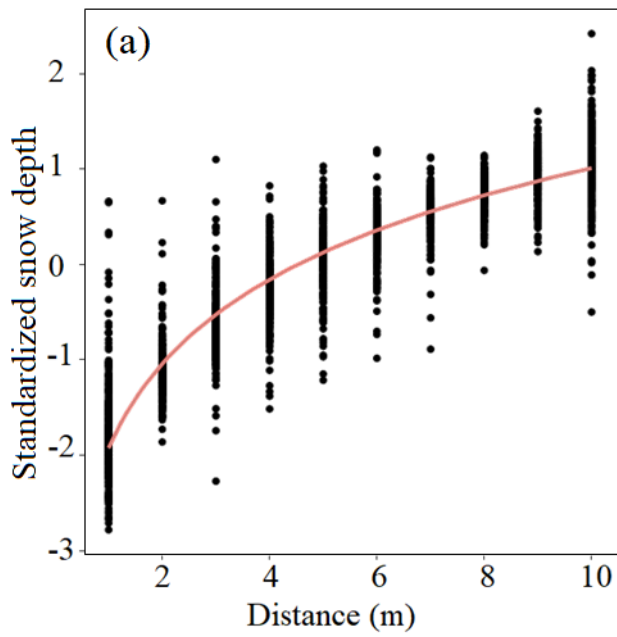
595 Figure 9: Increasing (a) and decreasing (b) snow depth trends and regression within a 10 m distance from the tree edges for all sites together. The confidence interval depicted in this figure is 95 %.
