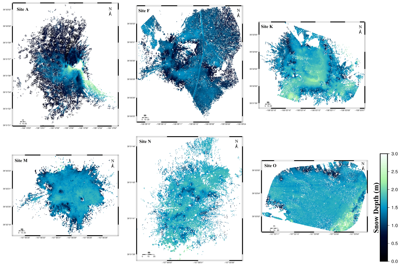
585 Figure 5: Snow depths at each site from TLS data.
