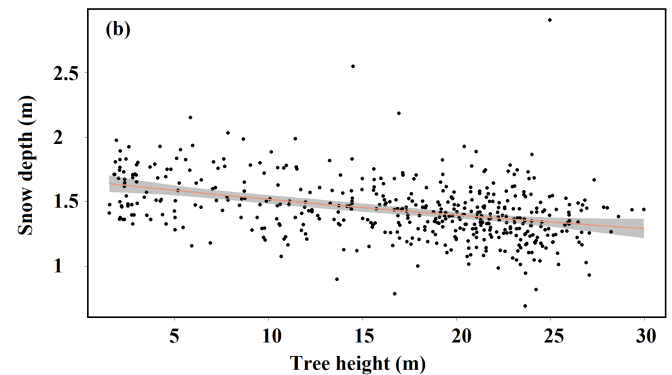
600 Figure 10: Tree height and snow depth within the 10 m transition zone in the south direction for (a) site A and (b) site K. The exponential and linear fit is shown with a red line along with 95 % confidence interval (grey).
