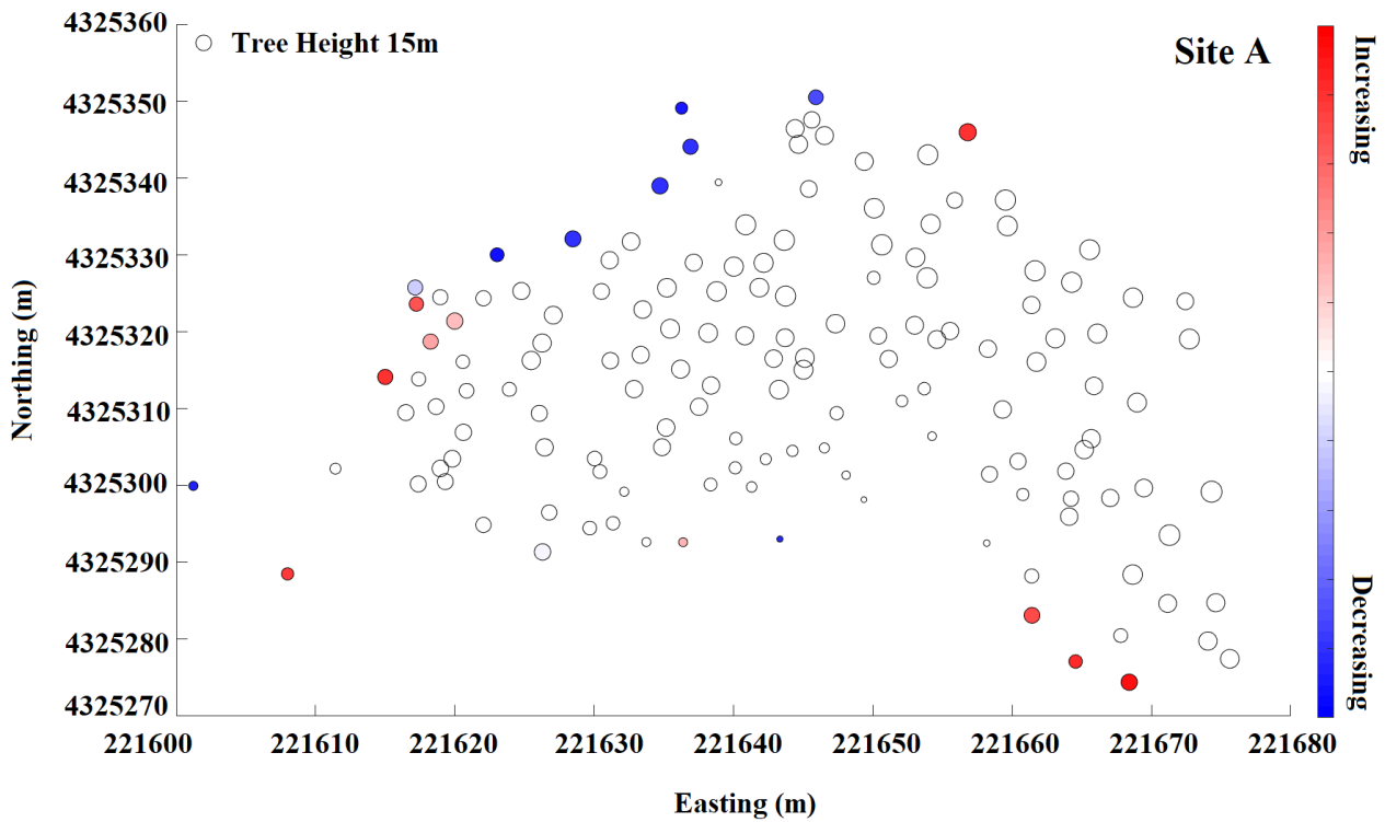
655 Figure B4: Snow depth change within a 10 m buffer from the edge of a tree at site A. Red color indicates snow depth increases moving from the tree edge toward the open and blue indicates snow depth decreases. Increasing and decreasing patterns are shown for individual trees at each site with adequate snow coverage.
