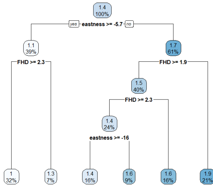
590 Figure 7: Decision tree at site O. Snow depth (m) are represented along with percent of the individual trees used for analysis.
