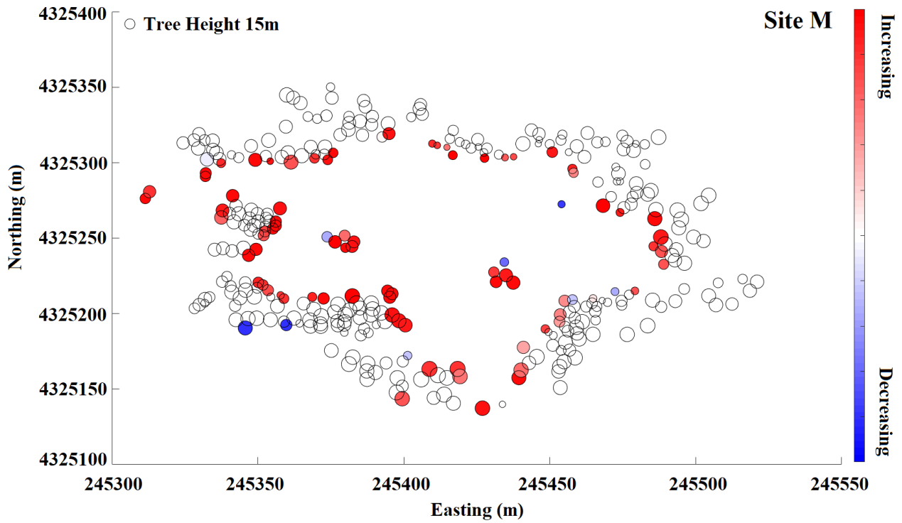
665 Figure B7: Snow depth change within a 10 m buffer from the edge of a tree at site M. Red color indicates snow depth increases moving from the tree edge toward the open and blue indicates snow depth decreases. Increasing and decreasing patterns are shown for individual trees at each site with adequate snow coverage.
