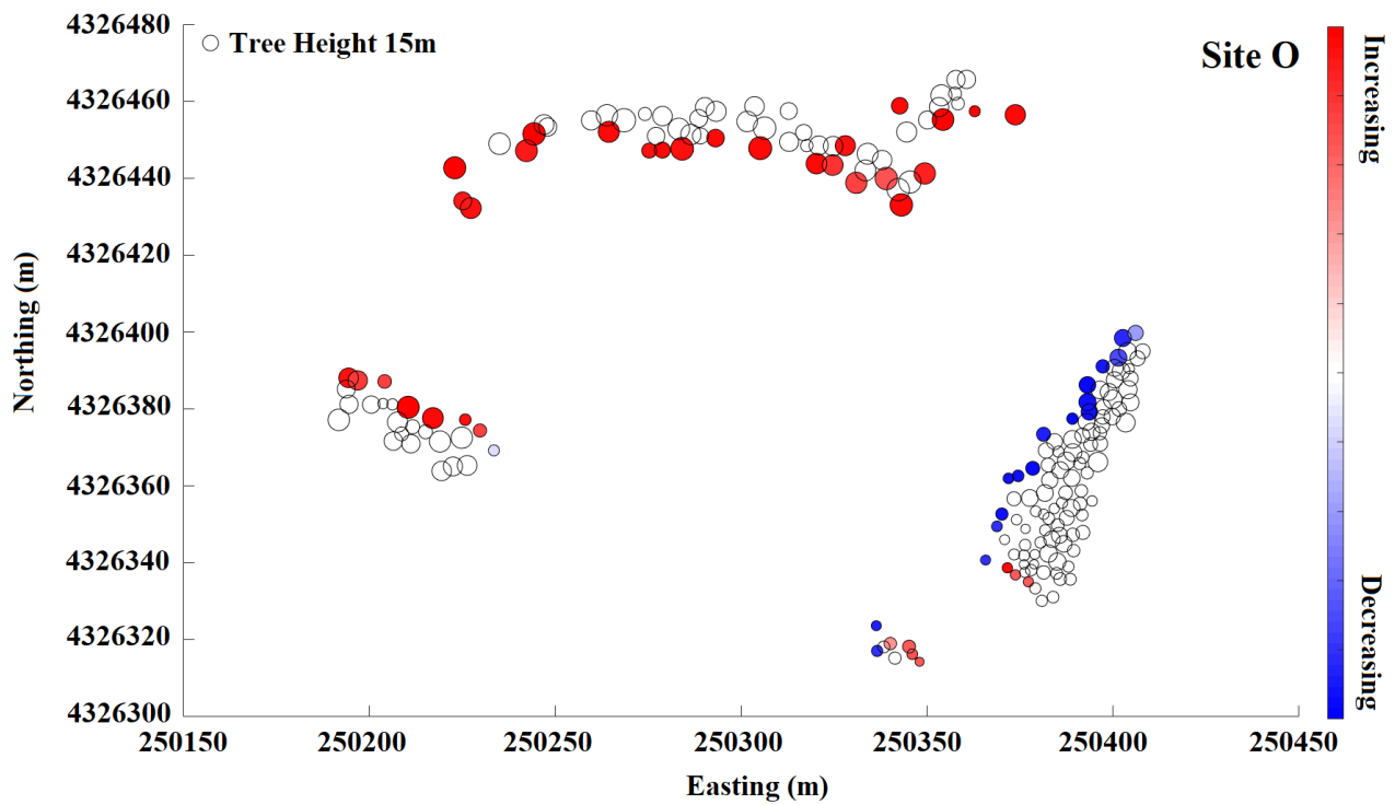
675 Figure B9: Snow depth change within a 10 m buffer from the edge of a tree at site O. Red color indicates snow depth increases moving from the tree edge toward the open and blue indicates snow depth decreases. Increasing and decreasing patterns are shown for individual trees at each site with adequate snow coverage.
