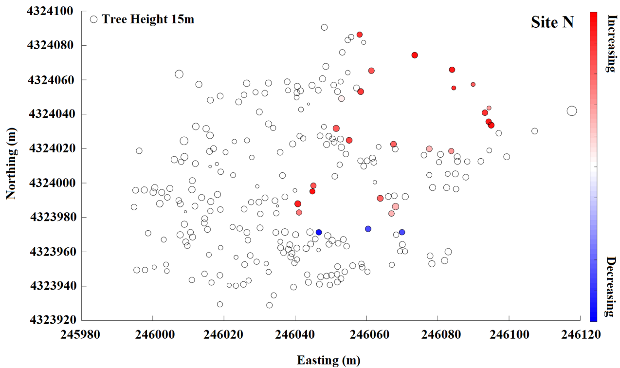
670 Figure B8: Snow depth change within a 10 m buffer from the edge of a tree at site N. Red color indicates snow depth increases moving from the tree edge toward the open and blue indicates snow depth decreases. Increasing and decreasing patterns are shown for individual trees at each site with adequate snow coverage.
