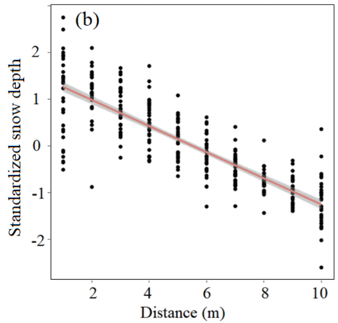
595 Figure 9: Increasing (a) and decreasing (b) snow depth trends and regression within a 10 m distance from the tree edges for all sites together. The confidence interval depicted in this figure is 95 %.
