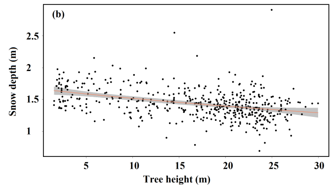
590 Figure 10: Tree height and snow depth within the 10 m transition zone in the south direction for (a) site A and (b) site K. The exponential and linear fit is shown with a red line along with 95 % confidence interval (grey).
