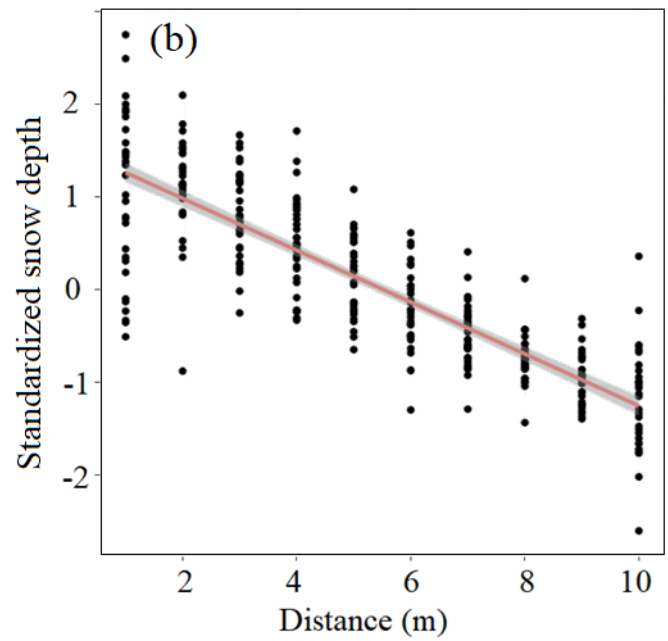
Figure 9: Increasing (a) and decreasing (b) snow depth trends and regression within a 10 m distance from the tree edges for all sites together. The confidence interval depicted in this figure is 95 %.
