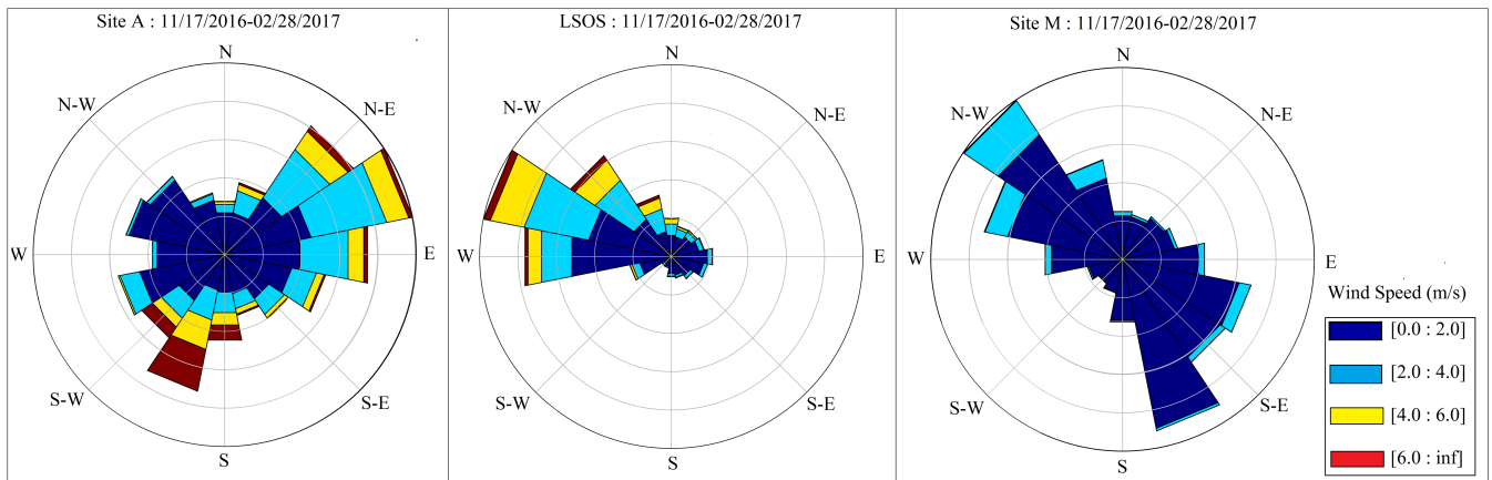
565 Figure 2: Rose diagrams of meteorological stations A, LSOS, and M.
