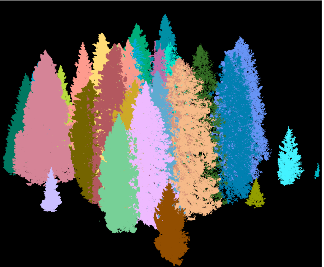
Figure B2: As an example, segmentation results for one las tile at site F.
