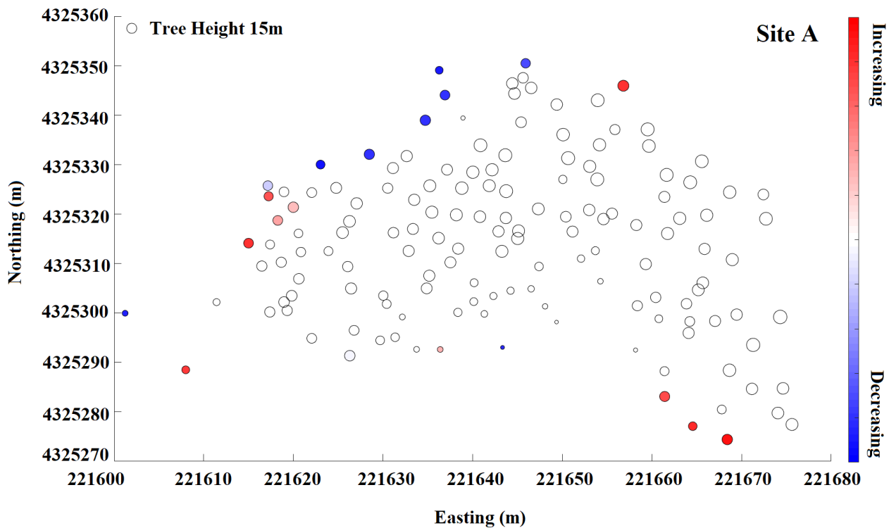
645 Figure B4: Snow depth change within a 10 m buffer from the edge of a tree at site A. Red color indicates snow depth increases moving from the tree edge toward the open and blue indicates snow depth decreases. Increasing and decreasing patterns are shown for individual trees at each site with adequate snow coverage.
