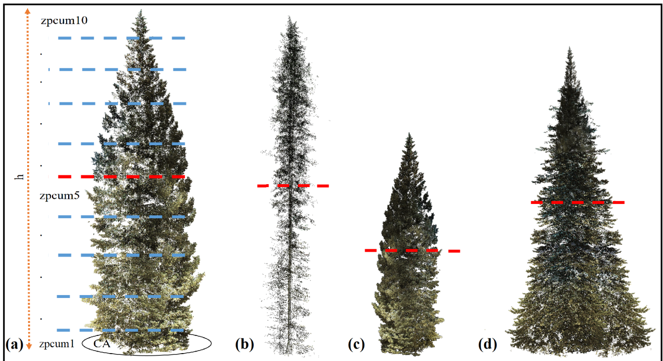
570 Figure 4: Graphical examples of trees with different structures and the metrics of foliage height diversity (FHD), crown volume and the cumulative percentage of vegetation returns (zpcum). Crown volume is estimated using crown area (CA) x height (h). Zpcum is based on 10 layers (zpcum1–zpcum10) (see example in (a)). Red dashed lines are examples of the cumulative layer with > 50 % of vegetation returns. The foliar complexity (FHD) of (a) and (c) are similar but the crown volumes and cumulative percentage of vegetation returns are different; whereas the FHD of (b) is the lowest.
