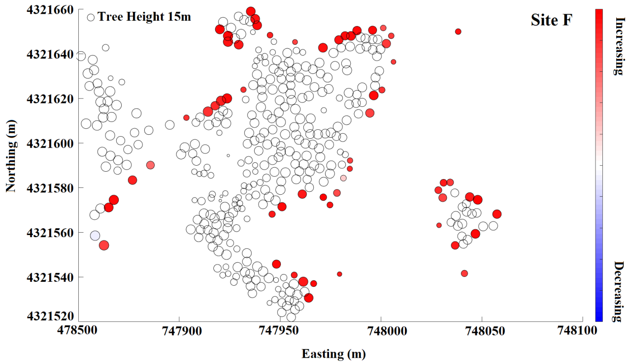
650 Figure B5: Snow depth change within a 10 m buffer from the edge of a tree at site F. Red color indicates snow depth increases moving from the tree edge toward the open and blue indicates snow depth decreases. Increasing and decreasing patterns are shown for individual trees at each site with adequate snow coverage.
