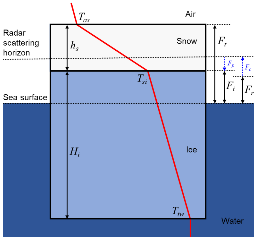
725 Figure 1. Schematic diagram of a typical snow–ice system during the winter. Snow depth ( h_s ), ice thickness ( H_i ), total freeboard ( F_t ), radar freeboard ( F_r ), and ice freeboard ( F_i ) are indicated. Correction terms regarding the wave propagation speed change in snow layer ( F_c ) and the displacement of the scattering horizon from the ice surface ( F_p ) are indicated by blue arrows. The red line denotes a typical temperature profile with air–snow interface temperature ( T_{as} ), snow–ice interface temperature ( T_{si} ), and ice–water interface temperature ( T_{iw} ).
