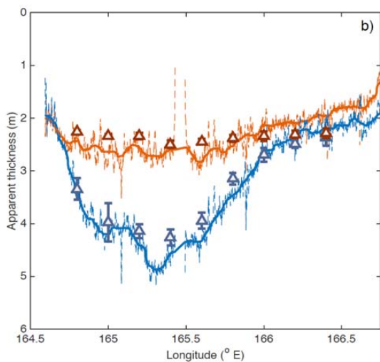
Figure 6: Apparent AEM thicknesses h_{a,Q} (orange lines) and h_{a,I} (blue lines) along E-W profiles at (a) 77°50'S and (b) 77°46' S in Nov 2011, approximately 3 km and 11 km from front of McMurdo Ice Shelf, respectively. Dotted lines are raw data, while solid lines are filtered with a 300 point median filter. Triangles show mean and standard deviation of drill-hole measurements at calibration points: Consolidated ice (snow plus ice; orange), and consolidated ice + ( \alpha = 0.4 ) SIPL thickness (blue; Eq. 5c).
