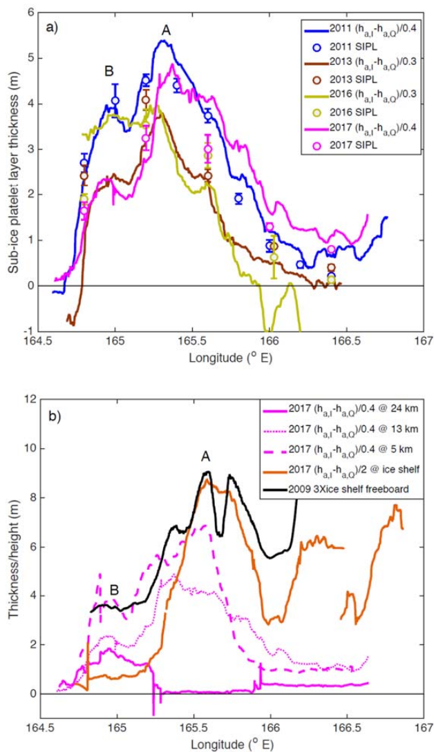
455 Figure 10: (a) SIPL thickness along 77°46'S in 2011, 2013, 2016 and 2017, approximately 11 km from McMurdo Ice Shelf front. Recurring local maxima or shoulders in thickness are identified at A and B. (b) SIPL thickness profiles in November 2017 at different distances from McMurdo Ice Shelf front (pink lines), at approximately 24 km (solid), 13 km (dotted) and 5 km (dashed). Figure also shows uncalibrated, scaled SIPL thickness beneath ice shelf in 2017 (brown), and scaled ice shelf freeboard in 2009 (black; from Rack et al 2013), at 77°55' S. The ice shelf data are smoothed by a moving average filter of window size 50. Local thickness maxima are identified at A and B.
