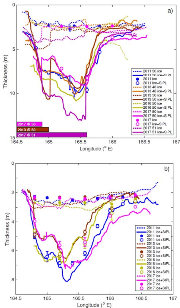
445 Figure 9: Interannual variability of AEM derived and drill-hole consolidated ice h_i (stippled lines and filled symbols) and total thickness h_i+h_{sipl} (solid lines and open symbols) along E-W transects at similar latitude (median filtered). (a) Transects at approximately 77°48'S to 77°51'S in Nov 2011, 2013, 2016, and 2017, approximately 3 to 5 km from McMurdo Ice Shelf front. Horizontal bars indicate very thick MY ice present in the West along part of the profiles in 2013 and 2017. (b) Transect at approximately 77°46'S in Nov 2011, 2013, 2016 and 2017, approximately 11 km from McMurdo Ice Shelf front. Note different y-axis scales, i.e. thicker SIPL farther south.
