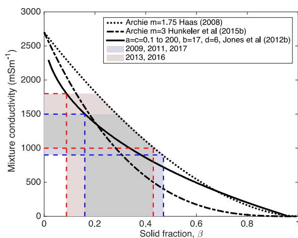
415 Figure 8: Conductivity versus solid fraction for porous media according to theories by Archie (1942) with different cementation factors m = 1.75 and 3 , and Jones et al. (2012b; black curves). Colored areas show range of SIPL conductivities derived from comparison of drill-hole and EM SIPL thicknesses (Fig. 5b, Table 1), and resulting solid fractions according to the different theories.
