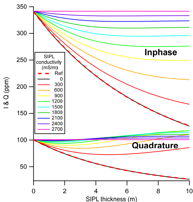
Figure 3: Inphase I and Quadrature Q responses to a 0 to 10 m thick SIPL under 2 m thick consolidated ice for SIPL conductivities of 0 to 2700 mS/m computed with three-layer EM forward model (see Fig. 2). Ref shows negative exponential curves for consolidated ice with zero conductivity used for computation of I and Q apparent thicknesses using Eq. 2b.
