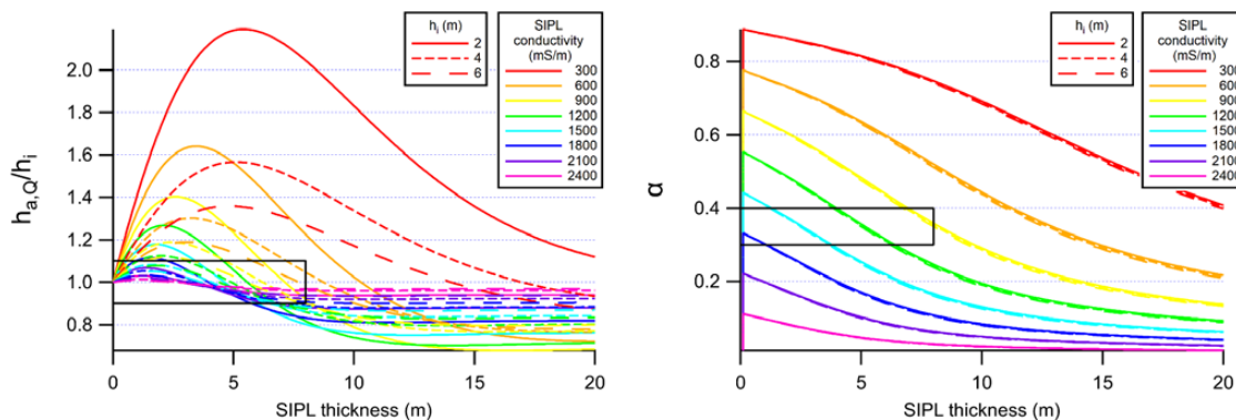
Figure 5: Ratio of h_{a,0}/h_i (left; see Eq. 5a) and \alpha = (h_{a,0} - h_i)/h_{sipl} (right; see Eq. 5c) versus SIPL thickness, at different consolidated ice thicknesses h_i between 2 and 6 m, and different SIPL conductivities between 300 and 2400 mS/m. Curves follow from curves in Figures 3 and 4. Black boxes show the range of h_{a,0}/h_i and \alpha values resulting from the calibration (Section 3.2).
