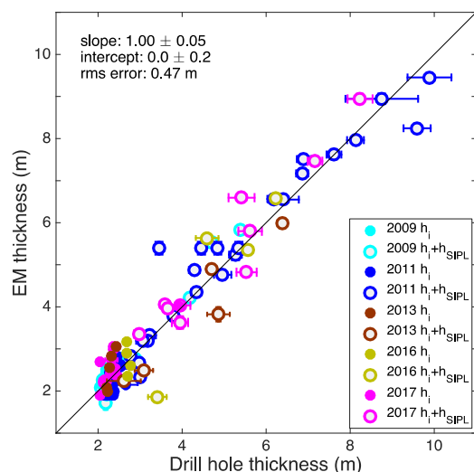
380 Figure 7: Scatter plot of EM derived versus drill-hole consolidated ice thickness ( h_i ; filled symbols) and total thickness ( h_i+h_{sipl} ; open symbols), with symbol color denoting year of measurement. Total thickness ( h_i+h_{sipl} ) was calculated with \alpha = 0.4 (best fit value 385 0.40 \pm 0.07 , N=46 ) for 2009, 2011, 2017 and \alpha = 0.3 for 2013 and 2016 (best fit value 0.30 \pm 0.15 , N=9 ), see Table 1. Error bars show ice thickness variability at each calibration location (5 drill holes) or within the approximate EM footprint (the latter are too small to be visible at the scale of the graph). The black line is 1:1. N = 9 for 2009, N = 26 for 2011, N = 5 for 2013, N = 4 for 2016, N = 11 for 2017, thus total N = 55 .
