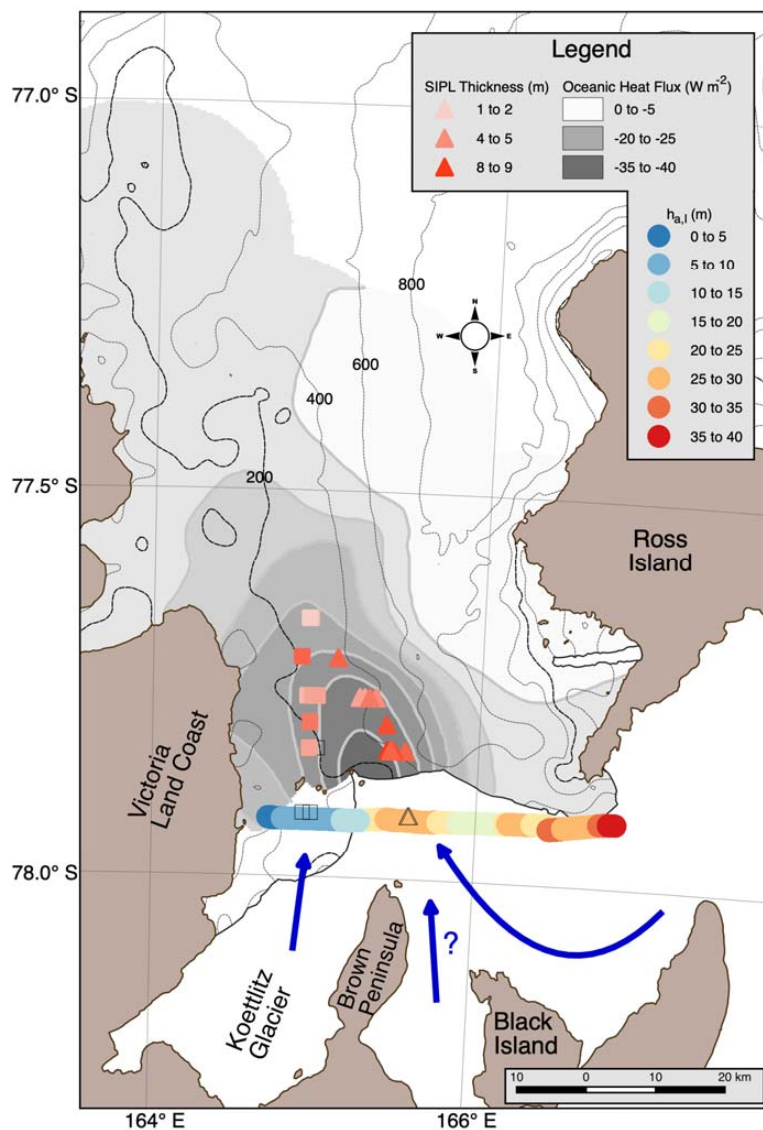
490 Figure 11: (a) Bathymetric map of McMurdo Sound showing the location of local maxima in SIPL thickness, with peak A as triangles, and B as squares for all years 2009, 2011, 2013, 2016 and 2017. The magnitude of the local maxima are colored proportionally to the thickness of the peak, with darker orange for thicker average SIPL. Open symbols denote peaks whose absolute thicknesses were uncertain. Colored horizontal line shows ice shelf h_{a,l} profile flown in 2017 with locations of corresponding A and B peaks identified. 495 Contours in grey are proportional to negative ocean heat flux from Langhorne et al. (2015). Blue arrows indicate possible paths of surface ISW (based on Robinson et al, 2014).
