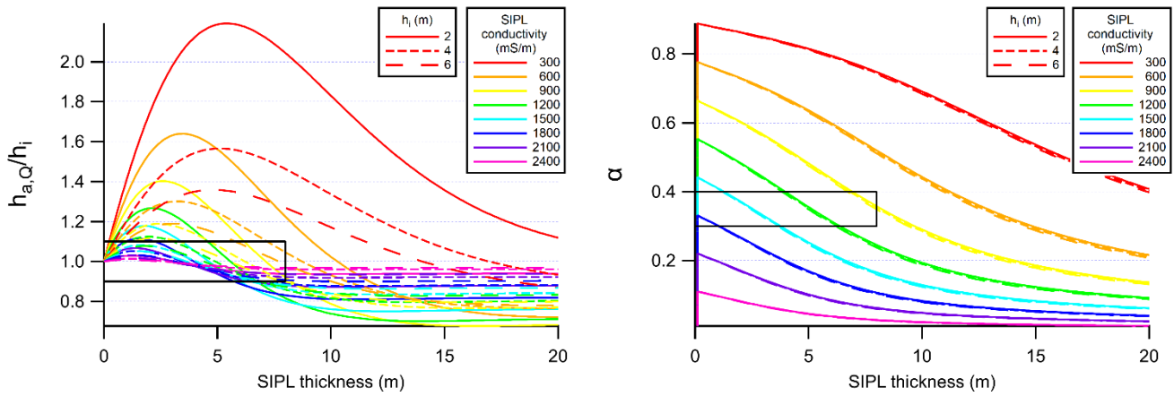
315 Figure 5: Ratio of h_{a,Q}/h_i (left; see Eq. 5a) and \alpha = (h_{a,I} - h_i)/h_{sipl} (right; see Eq. 5c) versus SIPL thickness, at different consolidated ice thicknesses h_i between 2 and 6 m, and different SIPL conductivities between 300 and 2400 mS/m. Curves follow from curves in Figures 3 and 4. Black boxes show the range of h_{a,Q}/h_i and \alpha values resulting from the calibration (Section 3.2).
