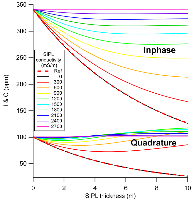
250 Figure 3: Inphase I and Quadrature Q responses to a 0 to 10 m thick SIPL under 2 m thick consolidated ice for SIPL conductivities of 0 to 2700 mS/m computed with three-layer EM forward model (see Fig. 2). Ref shows negative exponential curves for consolidated ice with zero conductivity used for computation of I and Q apparent thicknesses using Eq. 2b.
