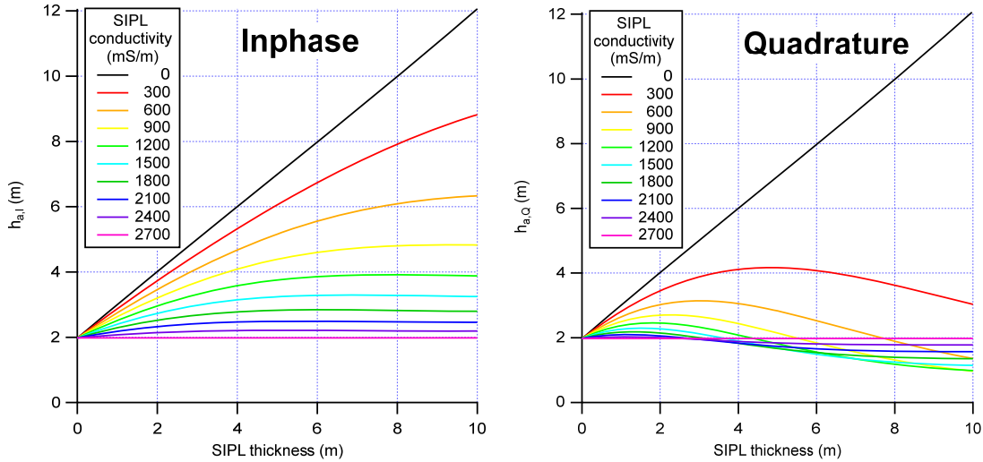
275 Figure 4: Apparent thicknesses resulting from applying simple negative-exponential equations like in Eq. 3a&b to the I and Q curves in Figure 3.
