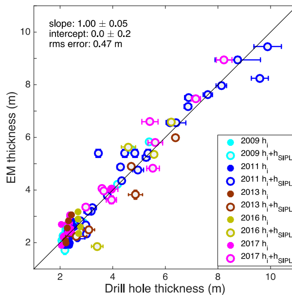
395 Figure 7: Scatter plot of EM derived versus drill-hole consolidated ice thickness ( h_i ; filled symbols) and total thickness ( h_i+h_{sipl} ; open symbols), with symbol color denoting year of measurement. Total thickness ( h_i+h_{sipl} ) was calculated with \alpha = 0.4 (best fit value 0.40 \pm 0.07 , N=46 ) for 2009, 2011, 2017 and \alpha = 0.3 for 2013 and 2016 (best fit value 0.30 \pm 0.15 , N=9 ), see Table 1. Error bars show ice thickness variability at each calibration location (5 drill holes) or within the approximate EM footprint (the latter are too small to be visible at the scale of the graph). The black line is 1:1. N = 9 for 2009, N = 26 for 2011, N = 5 for 2013, N = 4 for 2016, N = 11 for 2017, thus total N = 55 .
