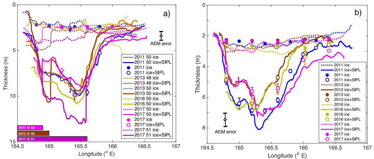
460 Figure 9: Interannual variability of AEM derived and drill-hole consolidated ice h_i (stippled lines and filled symbols) and total thickness h_i+h_{sipl} (solid lines and open symbols) along E-W transects at similar latitude (median filtered). (a) Transects at approximately 77^{\circ}48'S to 77^{\circ}51'S in Nov 2011, 2013, 2016, and 2017, approximately 3 to 5 km from McMurdo Ice Shelf front. Horizontal bars indicate very thick MY ice present in the West along part of the profiles in 2013 and 2017. (b) Transect at approximately 77^{\circ}46'S in Nov 2011, 2013, 2016 and 2017, approximately 11 km from McMurdo Ice Shelf front. Note different y-axis scales, i.e. thicker SIPL farther south. The data reduction model uncertainty in AEM total thicknesses (snow+ice+SIPL) is shown. 465
