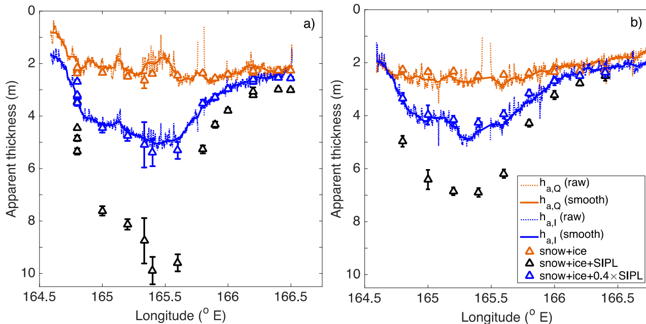
370 Figure 6: Apparent AEM thicknesses h_{a,Q} (orange lines) and h_{a,I} (blue lines) along E-W profiles at (a) 77°50'S and (b) 77°46' S in Nov 2011, approximately 3 km and 11 km from front of McMurdo Ice Shelf, respectively. Dotted lines are raw data, while solid lines are filtered with a 300 point median filter. Triangles show mean and standard deviation of drill-hole measurements at calibration points: Consolidated ice (snow plus ice; orange), consolidated ice + SIPL thickness (black) , and consolidated ice + ( \alpha = 0.4 ) SIPL thickness (blue; Eq. 5c).
