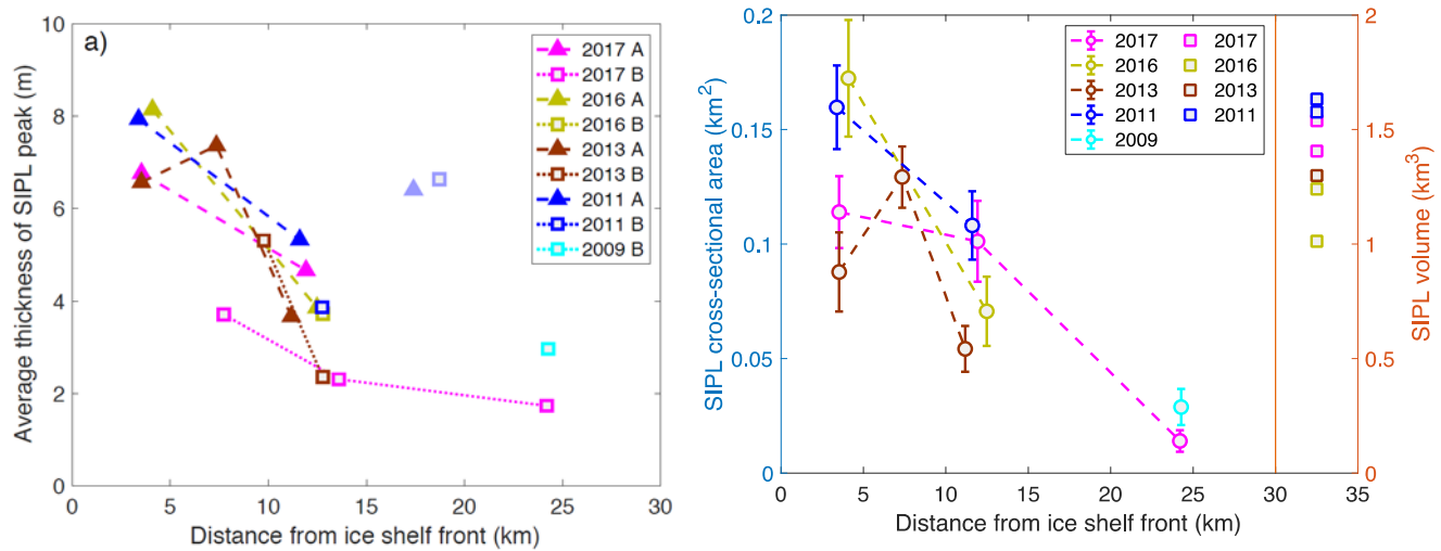
525 Figure 12: (a) SIPL thickness of peaks A and B (averaged over 0.1° of longitude) versus distance from ice shelf front for all years 2009, 2011, 2013, 2016 and 2017 (cf. Fig. 11). (b) East-west cross-sectional area through the SIPL region (defined as greater than 1 m thickness). Simultaneous SIPL volumes over a 675 km 2 area in the central McMurdo Sound from Brett et al. (2020) are shown on right (squares). Error bars assume a ± 0.5 m data reduction model uncertainty in EM SIPL measurements (Section 3.2).
