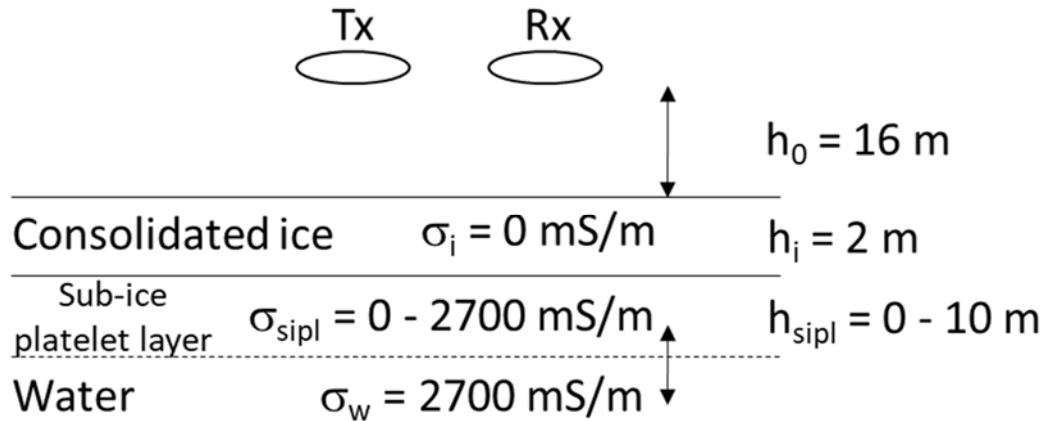
235 Figure 2: Schematic of the four-layer forward model to compute EM responses over sea ice underlain by a SIPL with variable thickness and conductivity. Tx and Rx illustrate transmitting and receiving coils, respectively. Instrument height h_0 = 16 m, snow + ice thickness h_i = 2 m, and water conductivity of 2700 mS/m are based on typical conditions during our surveys in McMurdo Sound.
