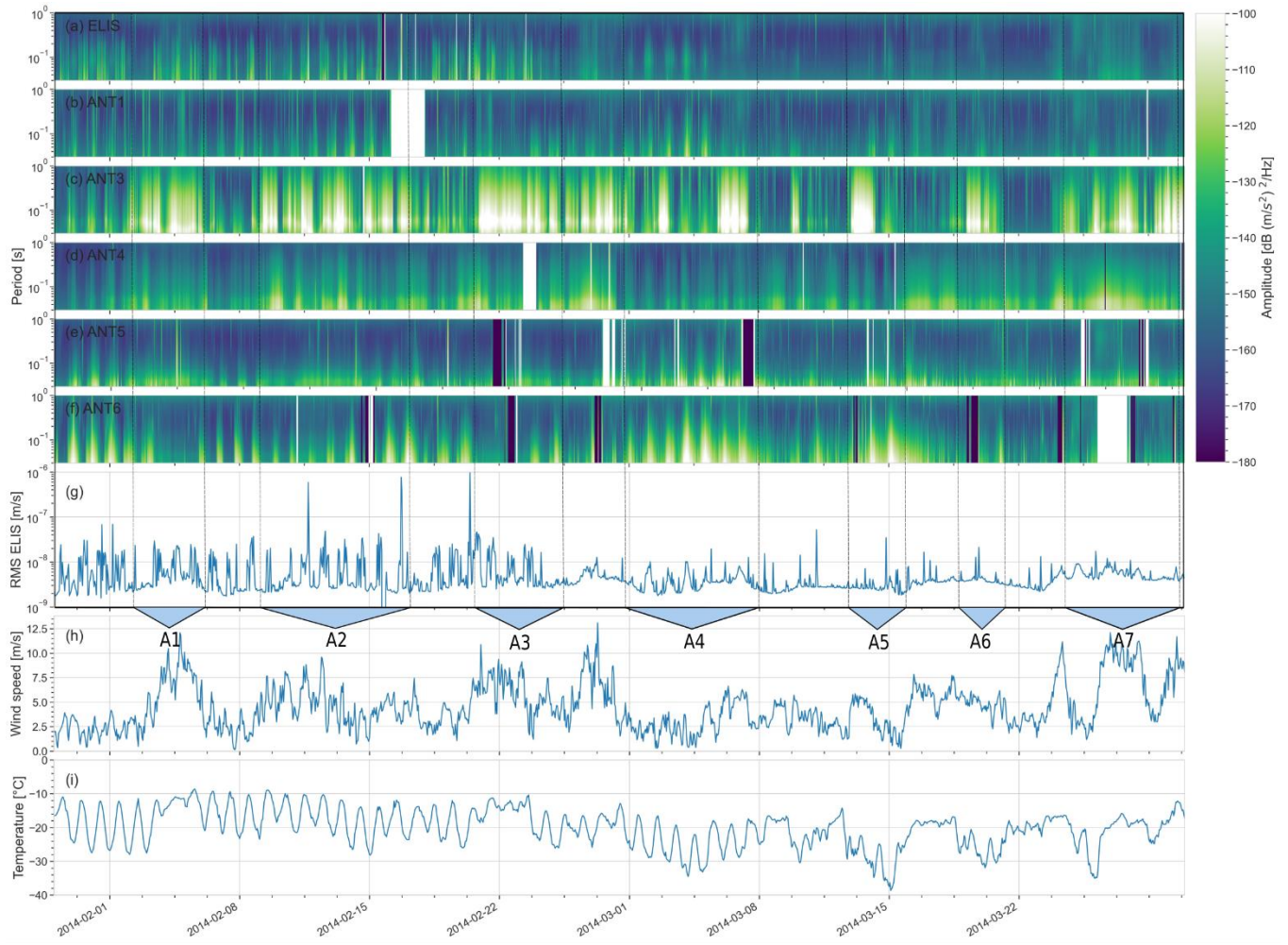
Figure 6: Belgian Antarctica Network Spectrograms (1 – 50 Hz) without wind noise for the 29/01/2014 – 30/03/2014 period with their associated the RMS for ELIS and the average wind speed [m/s] and temperature [°C] for the same period from the AWS station at ELIS. A1 – A7 represent periods of increased amplitude.
