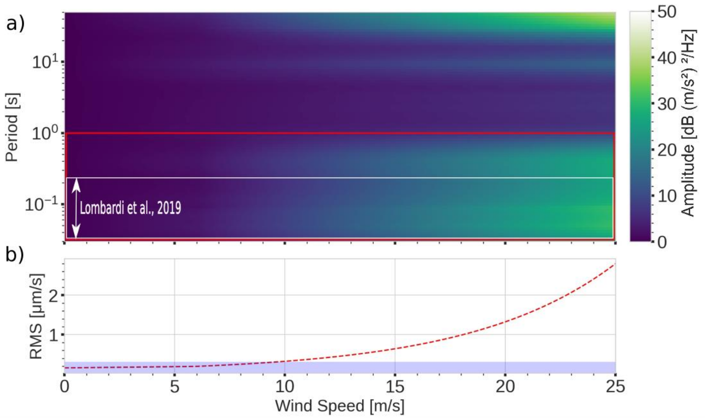
Figure 4: a) Relative Synthetic Spectrogram frequency and wind-speed dependent noise model representing wind-induced noise increase; in white is the frequency range of the thermally-induced icequakes observed by Lombardi et al., 2019. b) The 1 – 50 Hz RMS ground speed at ELIS HHZ extracted from the red rectangle on subplot a) and in light blue the amplitude range of these icequakes.
