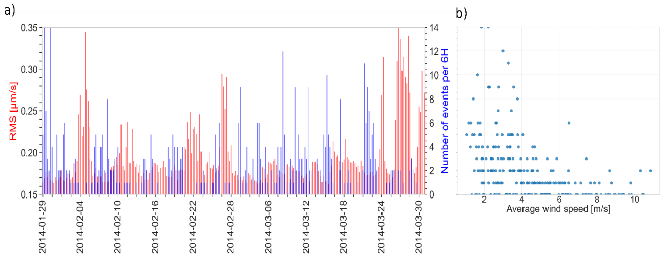
Figure 5: a) RMS per 6h calculated from the average wind speed and the noise model seen at ELIS vs the cumulative number of events detected icequake rate per 6h (seismic rate) by Camelbeeck et al. (2019). b) Icequake rate per 6h vs Average wind speed [m/s]
