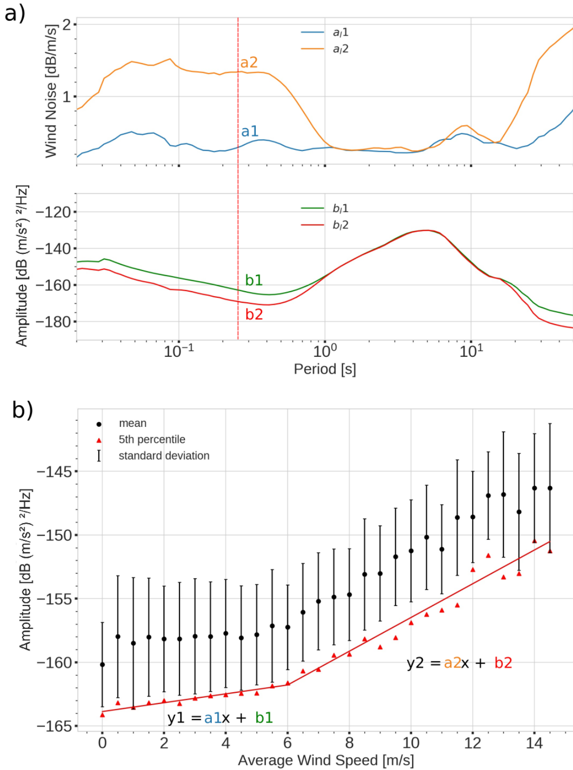
Figure 3: a): Wind Induced Noise Model describing the parameters of 2 linear functions for every period of ELIS HHZ in 2017: y = ax + b . The first subplot represents the “a” parameter in the linear regression y = ax + b and the second one shows the “b” parameter. Those 2 different linear relation parameters are until 6 m/s ( a_1/b_1 ) and after 6 m/s ( a_2/b_2 ). b): Behaviour of the 5 th percentile (red) and mean (black) noise amplitude for the 0.26 s period at ELIS HHZ for vs the average wind speed of 2017. [m/s] for the 0.26 s period (red dotted line on figure 3 a). There are 2 different red linear behaviours/functions: before 6 m/s ( y_1 ) and after 6 m/s respectively y_1 and y_2 : the parameters used are shown on the graph a) by the red line and their parameters.).
