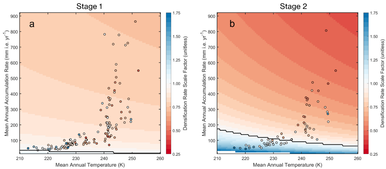
Figure 2. The dry-snow densification calibration coefficients for (a) stage 1, R_0 , and (b) stage 2, R_1 (Sect. 2.1.3; Eqns. 11–12, 15) over a range of mean annual temperatures and snow accumulation rates provide the background color contours. The coefficients derived for each of the calibration sites are plotted as closed circles, colored by their scale factor (i.e., calibration coefficients). The background color contours are derived directly from the calibrated R_0 , R_1 equations. The circles each represent the calibration coefficient derived directly from the depth-density profile at each calibration site. The black contour separates the region of enhanced densification (blue) from the region of reduced densification (red).
