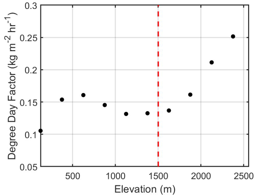
975 Figure 8. Mean degree-day factors over the Greenland Ice Sheet binned at 250 m elevation intervals for a temperature threshold, T_0 , of 270.25 K. We assume that degree-day factors above the vertical dashed red line at 1500 m are non-physical (i.e., too large). For all elevations greater than 1500 m, we apply a maximum degree-day factor equal to the mean within the 1250-1500 m elevation bin ( 0.13 \text{ kg m}^{-2} \text{ hr}^{-1} \text{ K}^{-1} ).
