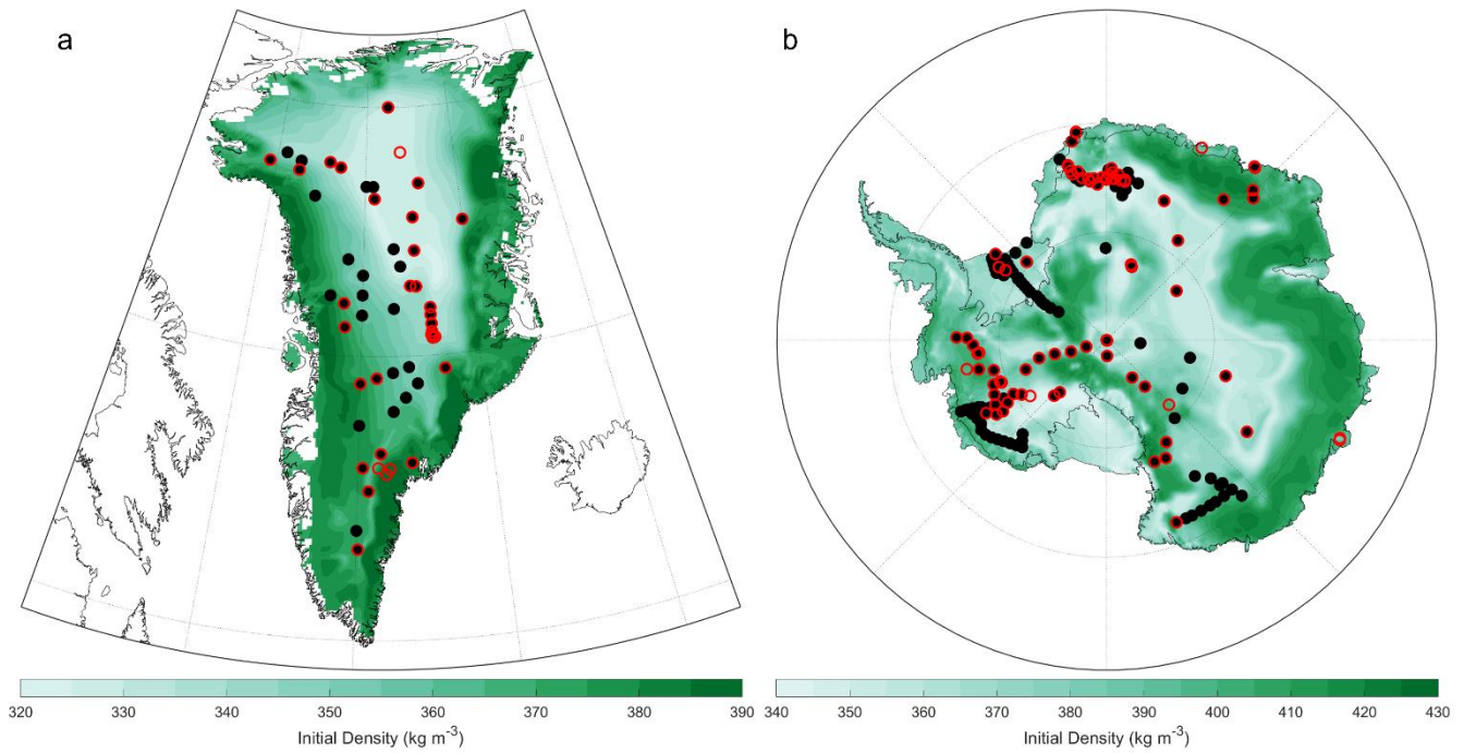
930 Figure 1. Modeled time-invariant initial density for the (a) Greenland and (b) Antarctic Ice Sheets. These results are based on MERRA-2 mean surface climate conditions. The solid black circles indicate locations that were used to train and test the initial density model as well as used in stage 1 calibration (Section 2.1.5), and the red open circles indicate sites used in stage 2 calibration. Note the differences in color scale for Greenland and Antarctica.
