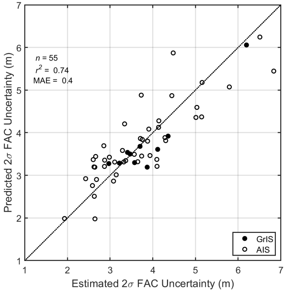
1010 Figure 12. Comparisons of the estimated 2-sigma uncertainty in FAC for both GrIS (solid circles) and AIS (open circles) and the model prediction of the 2-sigma uncertainty derived from Eqn. 20, which only applies to sites with a liquid-to-solid ratio (LSR) between 0 and 1 (Sect. 2.5.1). The uncertainty for those sites that fall outside of those LSR bounds were defined as their standard deviation through time (Eqn. 21). Performance statistics provided apply to the entire population (i.e., GrIS and AIS combined).
