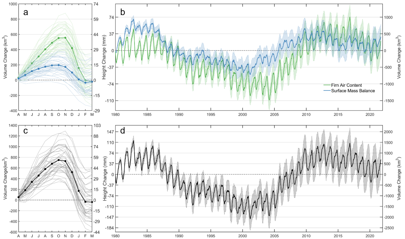
1045 Figure 18. Height and volume change of the Antarctic Ice Sheet (grounded and floating ice). (a) Seasonal changes separated 1050 into surface mass balance (SMB; blue) and firm air content (FAC; green) components. The thin lines represent each year, and the thick, dotted line represents the mean over the RCI (1980–2019). (b) A forty-year time series of volume and height change due to SMB and FAC. (c,d) The FAC and SMB combined height and volume change. The shaded regions represent the cumulative 2-sigma uncertainty in the volume changes, which accounts for spatial and temporal correlation in the time series. Note the differences in scale.
