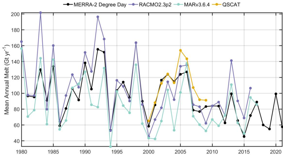
1095 Figure 25. Comparison of annual melt from the MERRA-2 degree day model (Sect. 2.2.1) and Trusel et al. (2013b) QSCAT-derived surface meltwater fluxes used to calibrate the degree day model, as well as two regional climate models, RACMO2.3p2 (Van Wessem et al., 2018) and MARv3.6.4 (Agosta et al., 2019).
