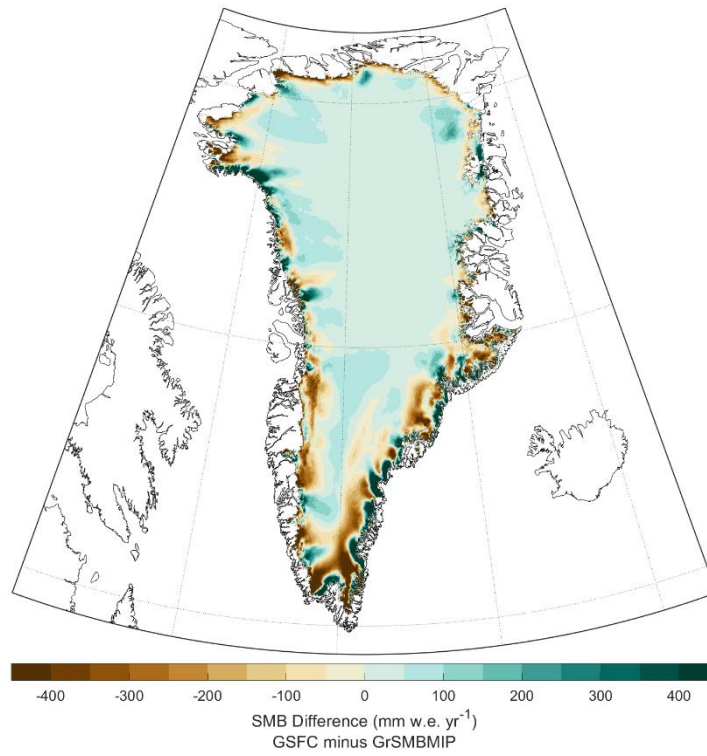
1070 Figure 21. The difference in mean annual SMB between GSFC and the GrSMBMIP ensemble mean.
