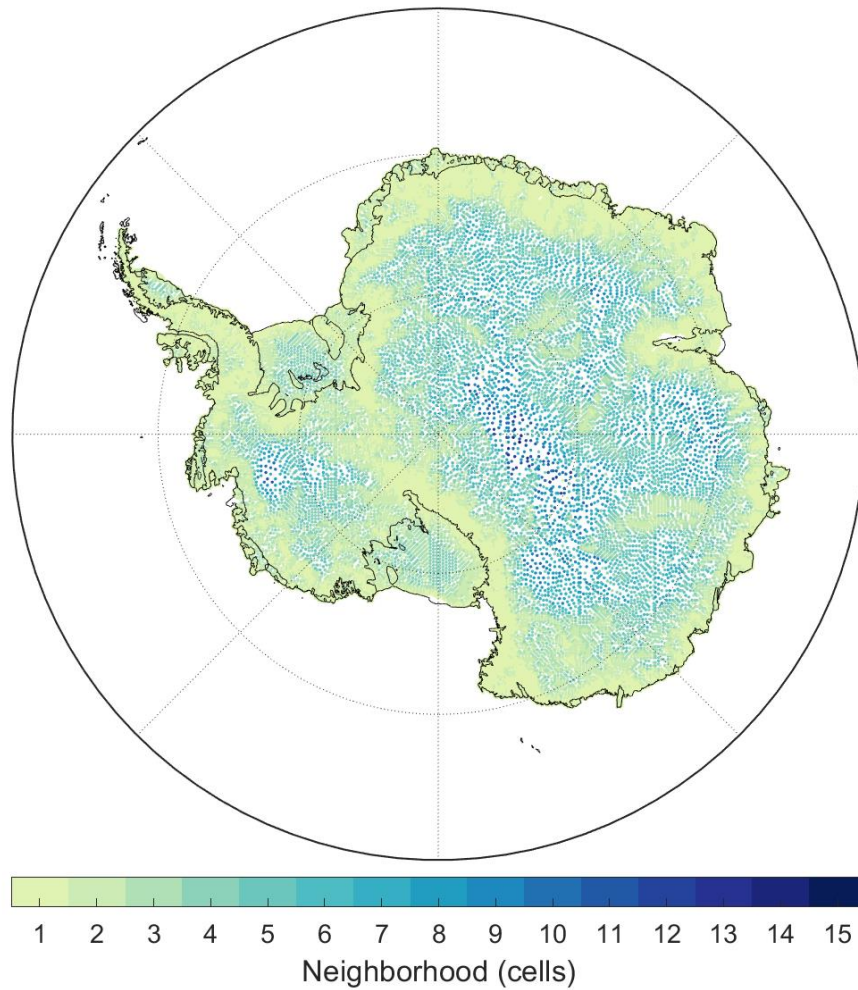
945 Figure 3. The Antarctic GSFC-FDM simulation locations colored by the representative size of their neighborhood. Darker colors (larger neighborhoods) with more white space (redundant simulations) indicate that the gradients in mean annual climate variables do not vary significantly over short length scales. Paler colors suggest stronger gradients with fewer redundant simulations.
