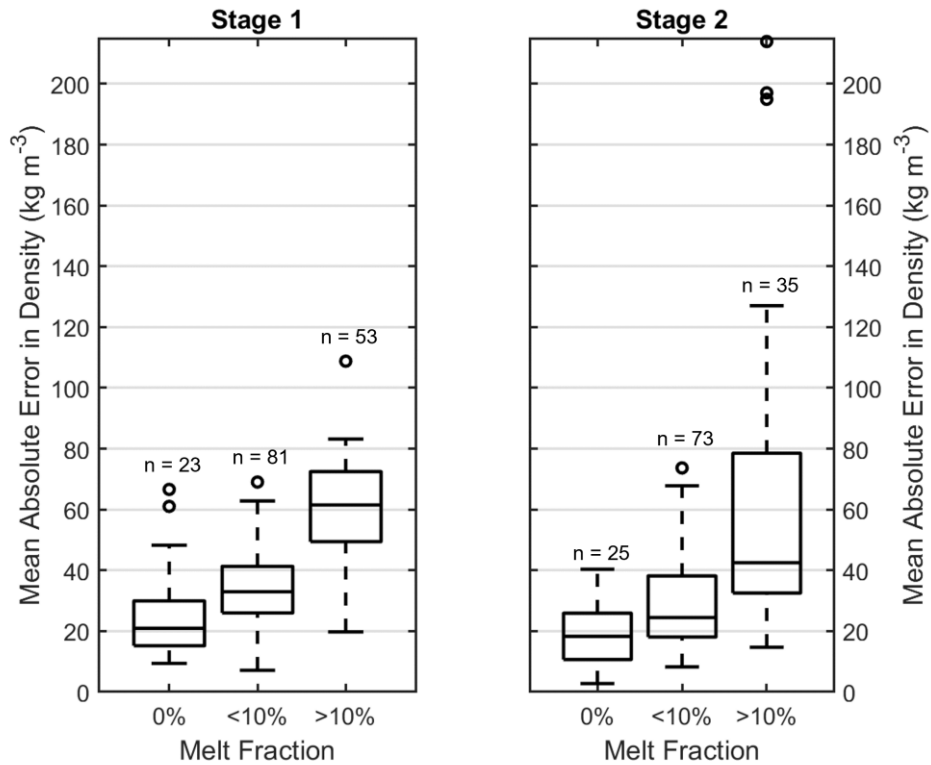
995 Figure 11. Boxplot of the mean absolute errors in density for stages (a) 1 and (b) 2 of densification in relation to the total melt experienced. The number of observations that make up each distribution is listed above each bar. The black rectangle represents the interquartile range of the mean absolute error while the horizontal line within represents the median. The whiskers show the maximum and minimum with outliers posted as open circles. Melt fraction is defined as the ratio of mean annual melt to mean annual snow accumulation expressed as a percentage.
