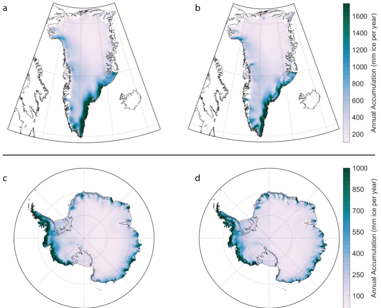
960 Figure 5. Mean annual net accumulation (snowfall-minus-sublimation) for the Greenland (upper) and Antarctic (lower) ice sheets from MERRA-2 (a,c) and M2R12K (b,d) over their contemporaneous time span (2000–2014). Note the differences in color scale for Greenland and Antarctica.
