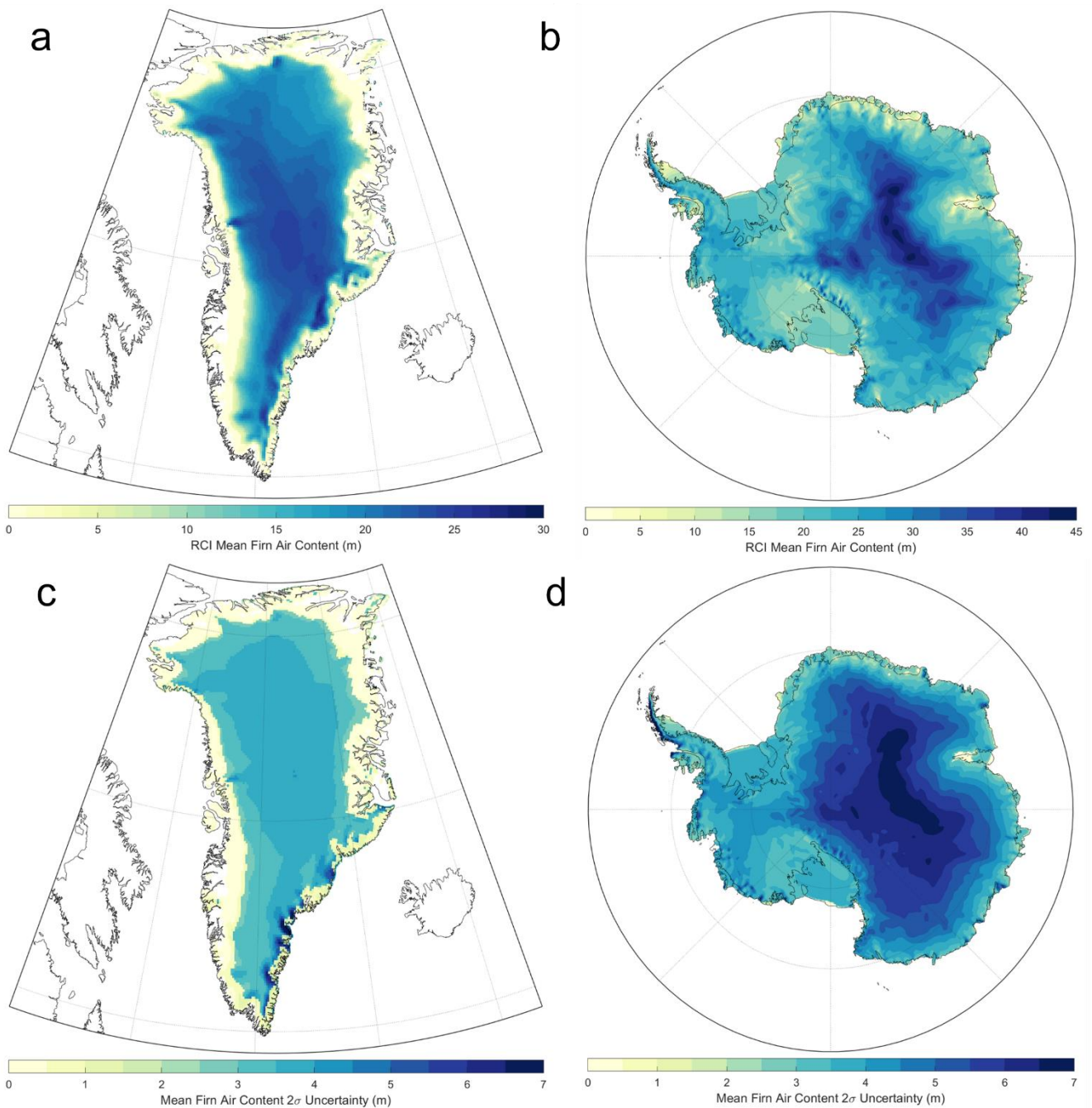
Figure 13. The mean firn air content (FAC) for the (a) Greenland Ice Sheet and (b) the Antarctic Ice Sheet over their 1015 respective reference climate intervals and (c,d) the respective 2-sigma uncertainty. Note the differences in color scale for Greenland and Antarctica and their uncertainties.
