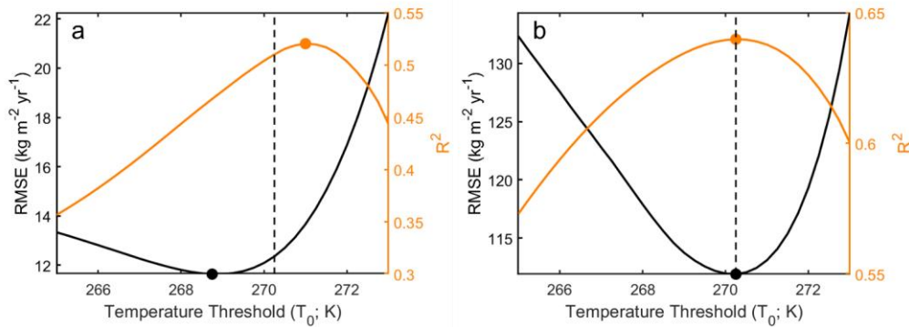
Figure 777. Degree-day model evaluation for (a) Antarctica and (b) Greenland for different temperature thresholds, T_0 . The orange and black lines represent the median-mean r^2 and RMSE of every grid cell for a given temperature threshold. The orange and black dots indicate the threshold that maximize r^2 and minimize RMSE , respectively. The dashed line represents the threshold selected for each ice sheet as it maximizes the distance between the two curve and yields the best model according to these evaluators. Note the differences in vertical scales.
