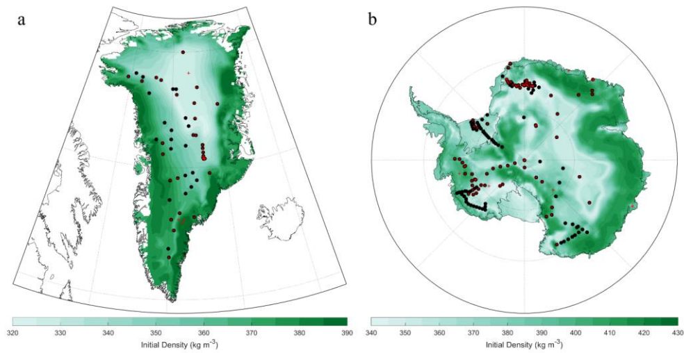
1665 Figure 1. Modeled time-invariant initial density for the (a) Greenland and (b) Antarctic Ice Sheets. These results are based on MERRA-2 mean surface climate conditions and Equation 21. The open circles are calibration site locations. The solid circles indicate locations that were used in stage 1 calibration to train and test the initial density model (Section 2.1.5), and the red + indicates sites used in stage 2 calibration. Note the differences in color scale for Greenland and Antarctica.
