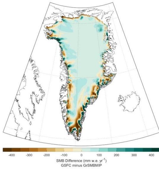
Figure 2124. The difference in mean annual SMB between GSFC and the GrSMBMIP ensemble mean.
