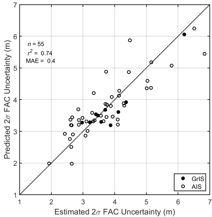
Figure 1242. Comparisons of the estimated 2-sigma uncertainty in FAC for both GrIS (solid circles) and AIS (open circles) and the model prediction of the 2-sigma uncertainty derived from Eqn. 20. Performance statistics provided apply to the entire population (i.e., GrIS and AIS combined).
