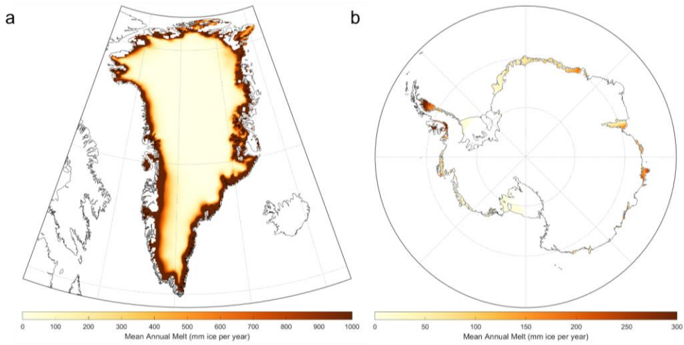
Figure 109.—Figure 9. Mean annual meltwater fluxes for the (a) Greenland and (b) Antarctic Ice Sheets based on a degree-day approach. Note the differences in color scale for Greenland and Antarctica.
