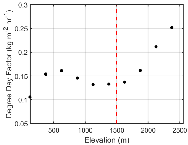
Figure 88. Mean degree-day factors over the Greenland Ice Sheet binned at 250 m elevation intervals for a temperature threshold, T_0 , of 270.25 K. We assume that degree-day factors above the vertical dashed red line at 1500 m are non-physical (i.e., too large). For all elevations greater than 1500 m, we apply a maximum degree-day factor equal to the mean within the 1250-1500 m elevation bin ( 0.13 \text{ kg m}^{-2} \text{ hr}^{-1} \text{ K}^{-1} ).
