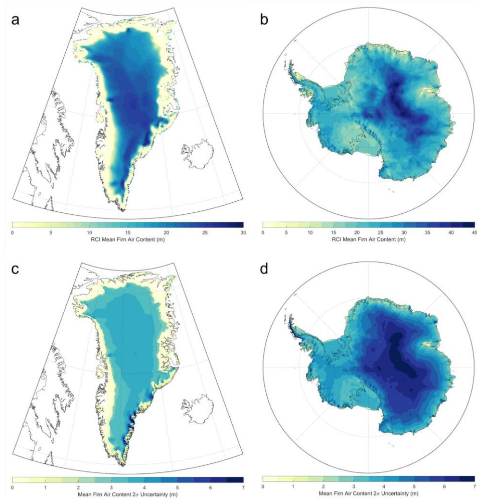
Figure 13.14.0. The mean firn air content (FAC) for the (a) Greenland Ice Sheet and (b) the Antarctic Ice Sheet over their respective reference climate intervals and (c,d) the respective 2-sigma uncertainty. Note the differences in color scale for Greenland and Antarctica and their uncertainties. Note the differences in scale.
