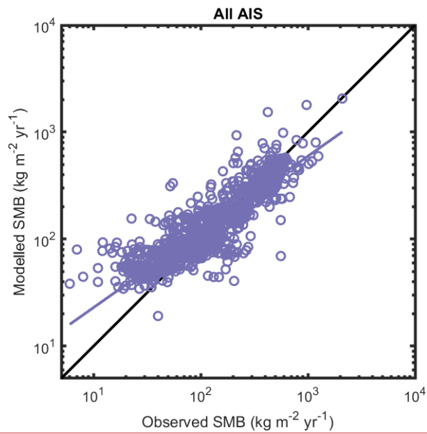
1835 Figure 2323. Comparison of N = 1201 observations of SMB with GSFC modelled SMB over the AIS. Note the logarithmic scale.
