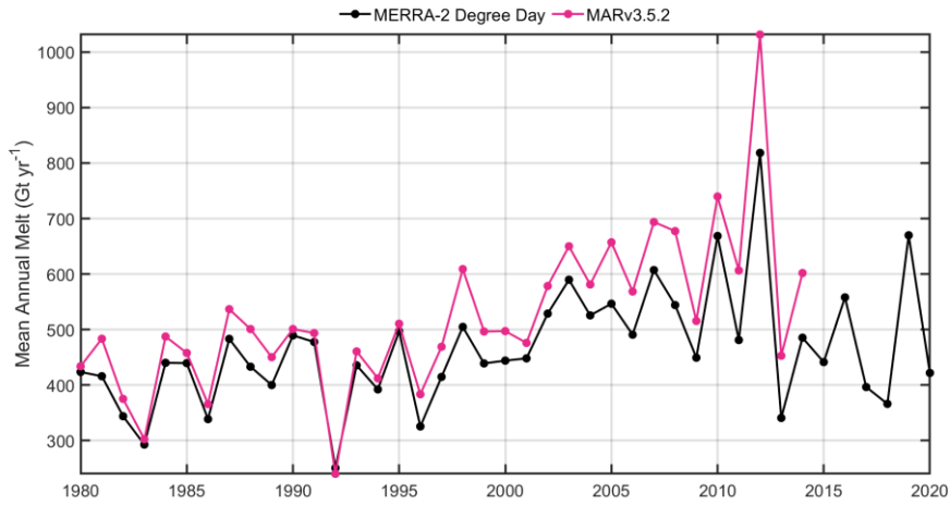
Figure 2222. Comparison of annual melt from the MERRA-2 degree-day model (Sect. 2.2.1) and MARv3.5.2, the model used to train the degree-day model (Fettweis et al., 2017).
