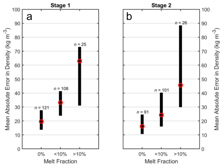
1740 Figure 11 . Range of mean absolute errors in density for stages (a) 1 and (b) 2 of densification in relation to the total melt experienced. The number of observations that make up each distribution is listed above each bar. The black bar represents the interquartile range of the mean absolute error while the red circle represents the median. Melt fraction is defined as the ratio of mean annual melt to mean annual snow accumulation expressed as a percentage.
