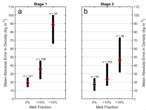
Figure 98. Range of mean-absolute errors in density for stages (a) 1 and (b) 2 of densification in relation to the total melt experienced. The number of observations that make up each distribution is listed above each bar. The black bar represents the interquartile range of the mean-absolute error while the red circle represents the median. Melt fraction is defined as the ratio of mean annual melt to mean annual snow accumulation expressed as a percentage.
