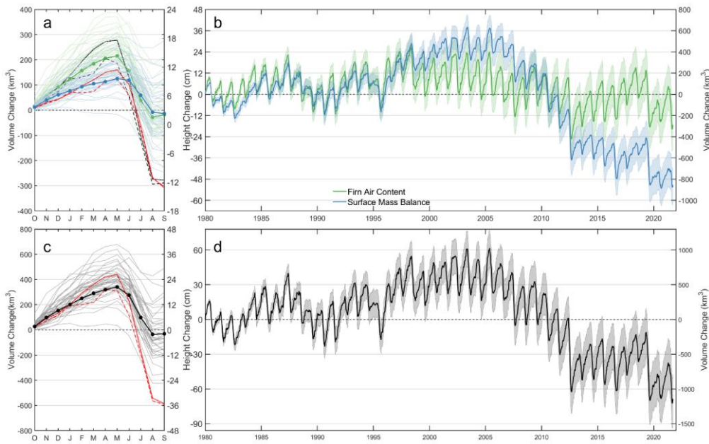
Figure 161613. Height and volume change of the Greenland Ice Sheet. (a) Seasonal changes separated into surface mass balance (SMB; blue) and firn air content (FAC; green) components. The thin lines represent each year, and the thick, dotted line represents the mean over the RCI (1980–1996). The solid and dashed lines represent the 2012 and 2019 mass balance years, respectively, where the black lines represent FAC and the red lines represent SMB. (b) A forty-year time series of volume and height change due to SMB and FAC. (c,d) The FAC and SMB combined height and volume change. The shaded regions represent the cumulative 2-sigma uncertainty in the volume changes, which accounts for spatial and temporal correlation in the time series. Note the differences in scale.
