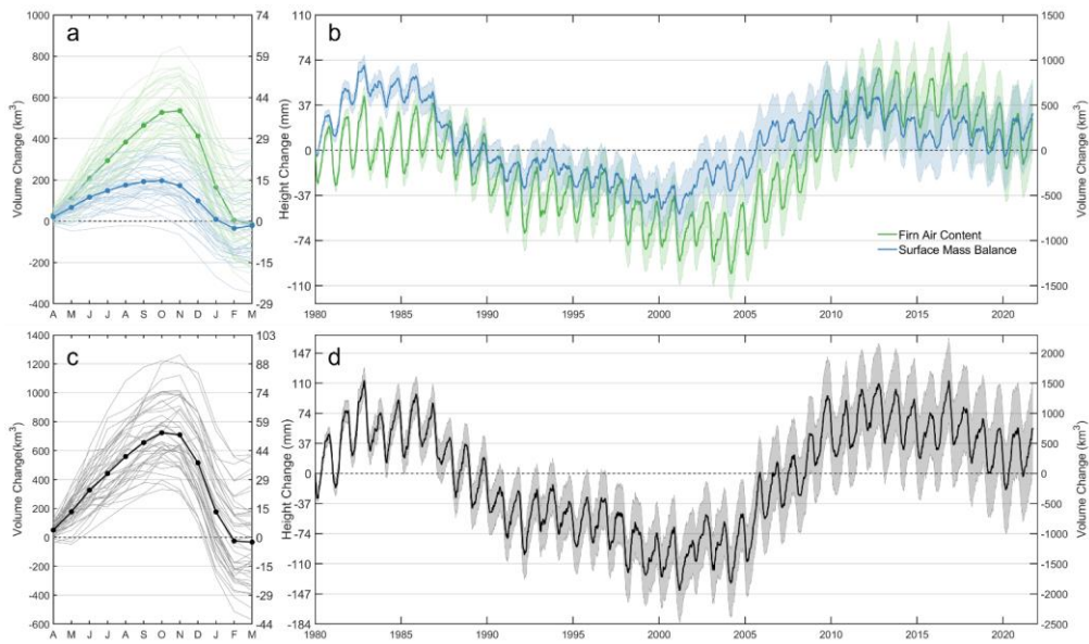
Figure 181814. Height and volume change of the Antarctic Ice Sheet (grounded and floating ice). (a) Seasonal changes separated into surface mass balance (SMB; blue) and firm air content (FAC; green) components. The thin lines represent each year, and the thick, dotted line represents the mean over the RCI (1980–2019). (b) A forty-year time series of volume and height change due to SMB and FAC. (c,d) The FAC and SMB combined height and volume change. The shaded regions represent the cumulative 2-sigma uncertainty in the volume changes, which accounts for spatial and temporal correlation in the time series. Note the differences in scale.
