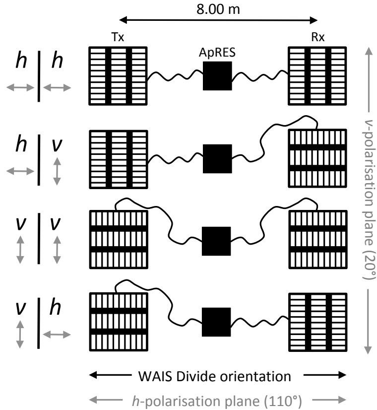
Figure 1. Four orthogonal combinations of antenna orientations as used for the polarimetry experiments in this study . Antennas (Tx = transmitting, Rx = receiving) were positioned 8.00 m apart and rotated 90° in a vertical (v) or horizontal (h) orientation. The orientation nomenclature (Tx | Rx) is with respect to the electric field of the antenna (grey arrows). The antenna-axis-h-polarisation plane (110°) was oriented approximately parallel with the WAIS Divide orientation.
