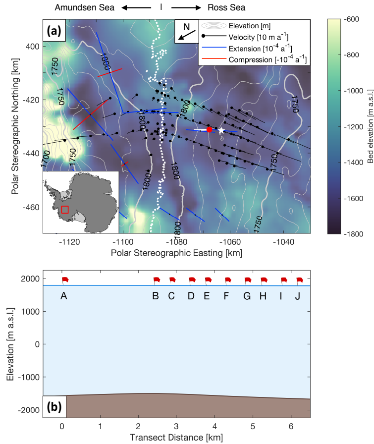
Figure 2. (a) Map of local surface (white contours, REMA, Howat et al., 2019) (m a.s.l. with white contours at 10 m intervals, REMA, Howat et al., 2019) and bed topography (background colour, MEaSUREs BedMachine Antarctica, Morlighem et al., 2020) in the WAIS Divide area, as well as GPS-measured surface velocities (black lines, Conway and Rasmussen, 2009) and strain configurations (blue and red arrows, Matsuoka et al., 2012). Strain rates below 2.5 \times 10^{-5} \text{ a}^{-1} are not shown. The locations of the ApRES polarimetry transect (solid white line) and the results presented from Site I (red dot) in this study are shown relative to \sim 5 \text{ km} NE of the WAIS Divide Deep-Ice Core site (WDC, white star). The WAIS Divide is delineated as a thick dotted white line, with ice flowing northwards towards the Amundsen Sea and southwards towards the Ross Sea. Location of (a) is shown as a red box in the map inset. (b) Surface and basal topography along the ApRES polarimetry transect showing the relative locations of the 10 ApRES measurement sites. Site A is closest to the WAIS Divide, and Site J is closest to the WDC core site. The results shown in Figures 4-6 depict the fabric profile of Site I, which has an estimated ice thickness of 3426 m from BedMachine.
