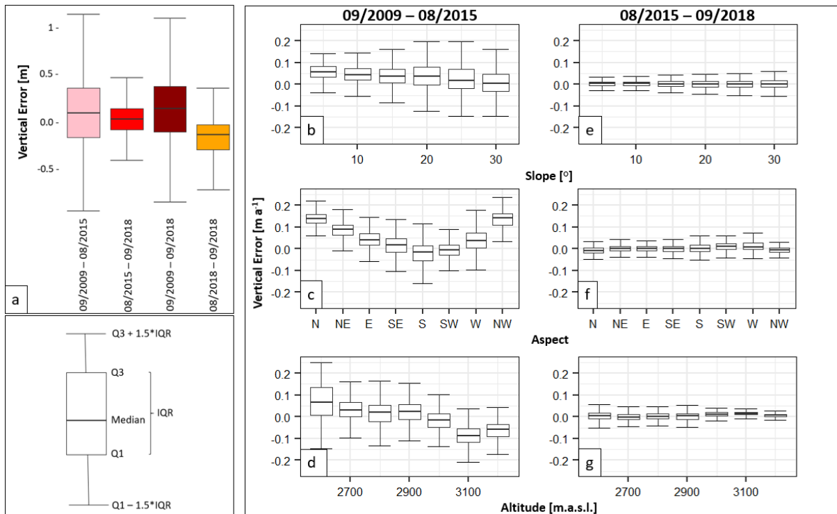
305 Figure 6: Overall vertical error of the DSM differences (a); Annual vertical error for the periods 09/2009-08/2015 (b-d) and 08/2015-09/2018 (e-g) in relation to slope (b,e), aspect (c,f) and altitude (d,g).
