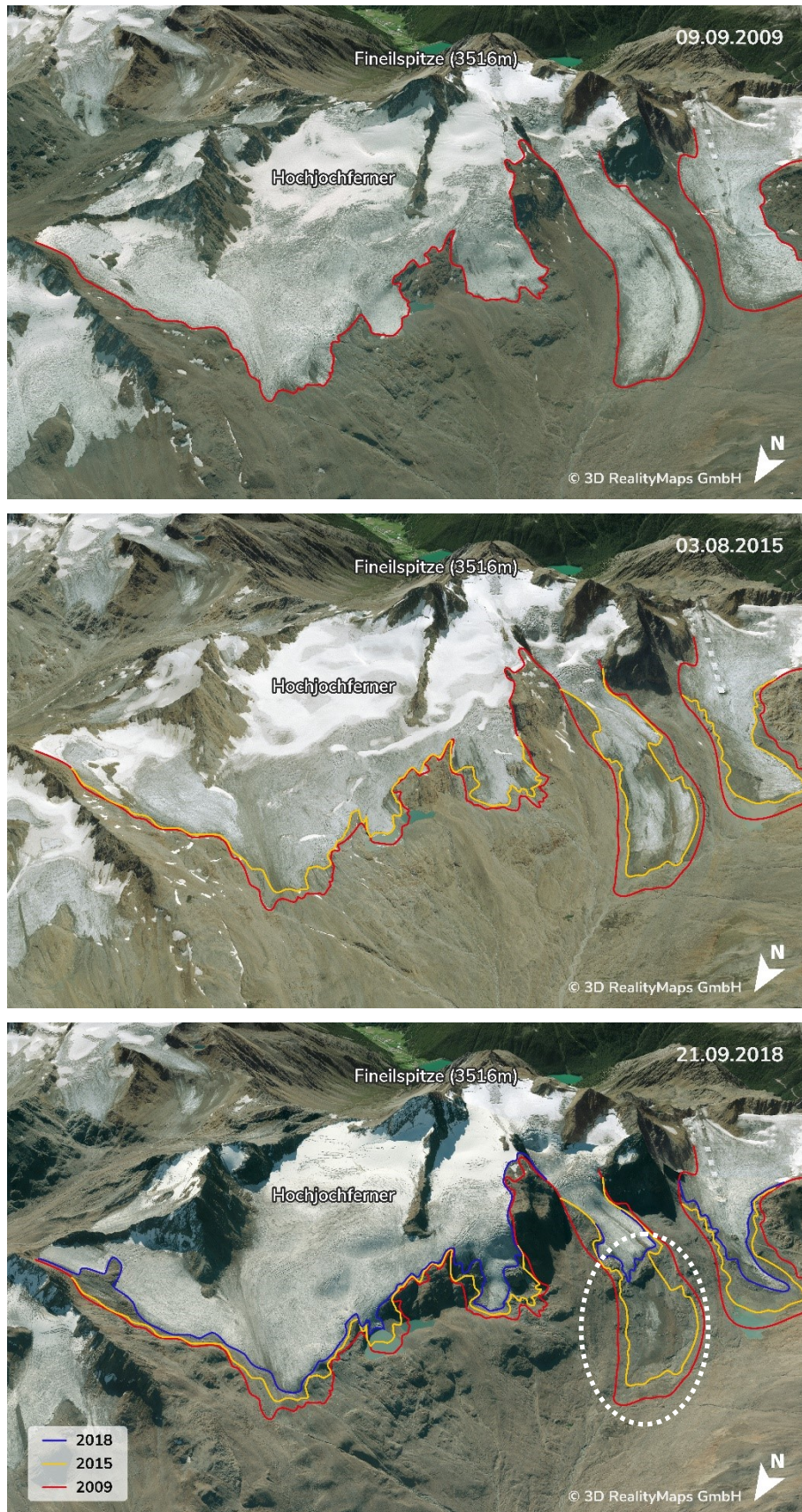
290 Figure 5: 3D visualization of the length change for the Hochjochferner in 2009 (top), 2015 (middle), and 2018 (bottom); Lines indicate glacier extent for the respective years. The second glacier tongue from the right (white dotted circle) lost 826 m in 9 years.
