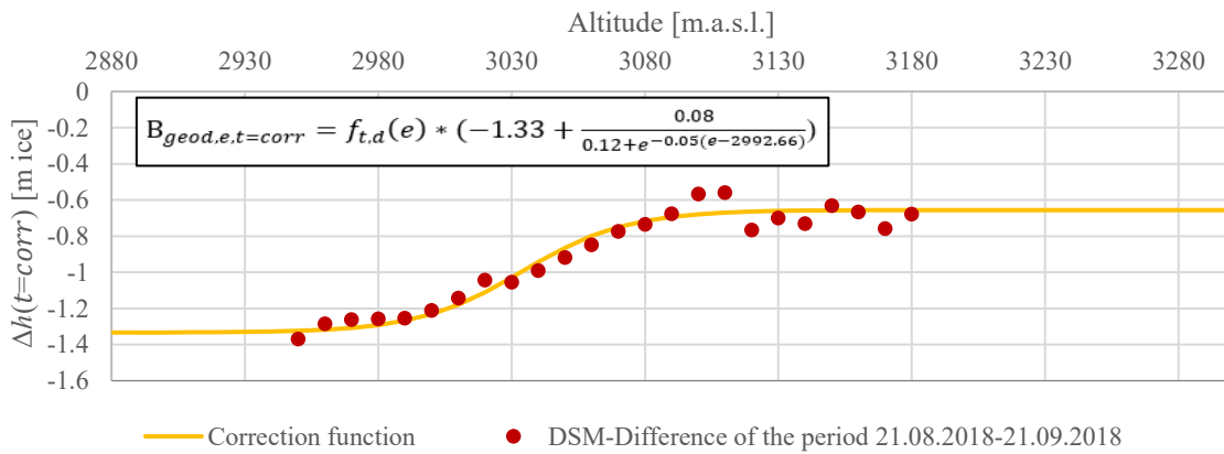
Figure 3: Surface changes in 10 m altitude bins for the correction period (21.08.2018 to 21.09.2018, red dots); Regression curve (yellow), representing height changes related to the altitude; SD of the regression is 0.07 m ice.
