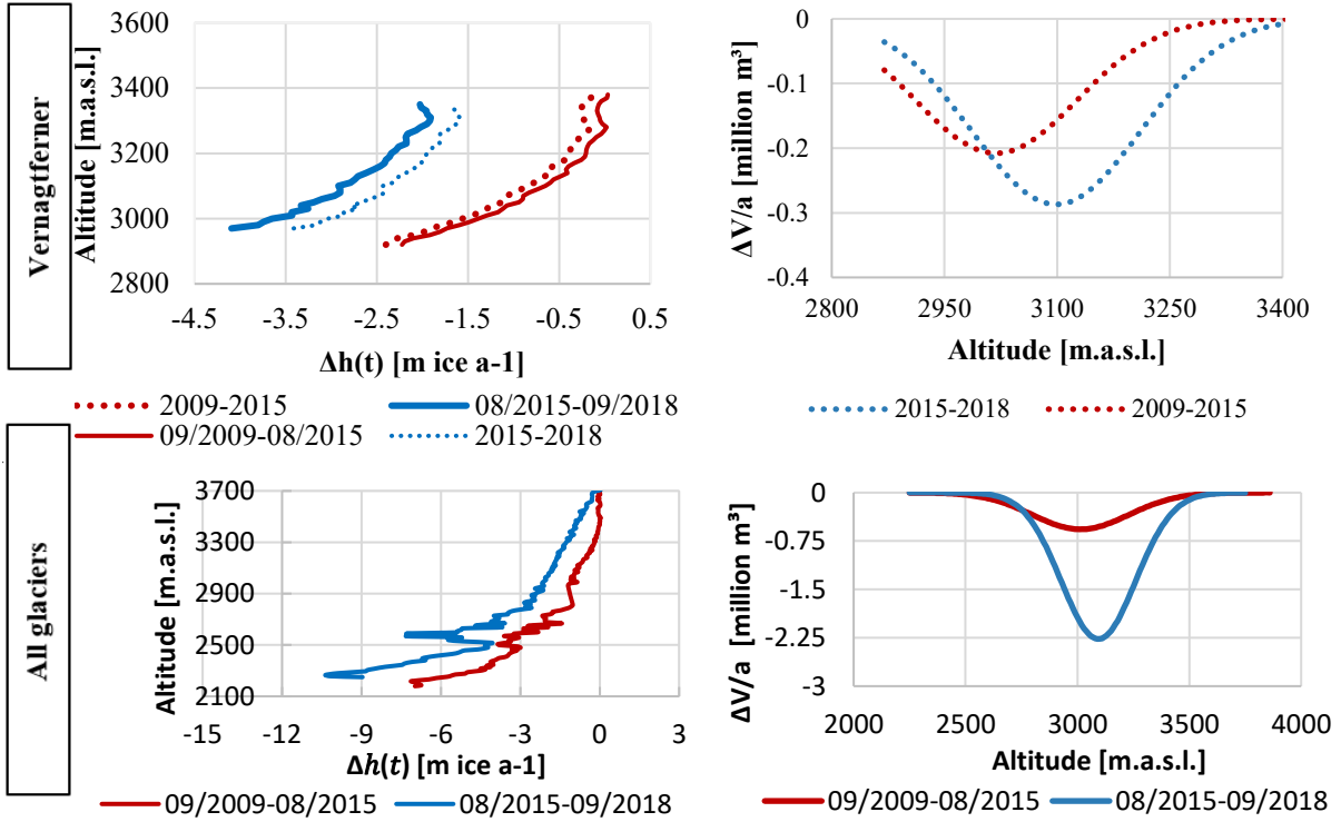
Figure 7: Top left: Annual height changes \Delta h(t) per altitude for the Vernagtferner, Bottom left: Surface height 325 changes of all glaciers; Right: annual volume changes for the Vernagtferner (top) and all glaciers (bottom); Dotted lines represent the surface or volume changes after the correction of the acquisition dates.
