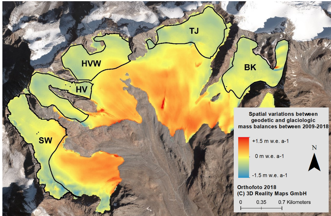
Figure 10: Top: Variation Raster 2009–2018: Spatial variations of the annual geodetic (corrected) and glaciological mass balance data; Blue areas with negative variations represent areas where B_{\text{geod},t} < B_{\text{glac},t} . In red areas, the opposite relation is present (see Eq. 7). For regions that appear yellow, both methods present similar mass balances; Black outlines represent the different accumulation areas of the Vernagtferner.
