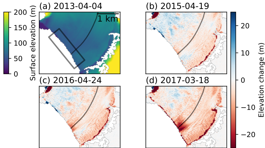
Figure 4. Elevation distribution in September 2014–April 2013 (a) and elevation change from April 2015 to March 2017 (b–d), using ArcticDEM. Colors in (b–d) show the total elevation change relative to September 2014–April 2013 (negative, red, means lowering). The manually traced location of the moraine (Fig. 1a) is indicated by a transparent black line in all panels, and the location of cropped ortho-images in Fig. 3 is shown by a black rectangle in (a).
