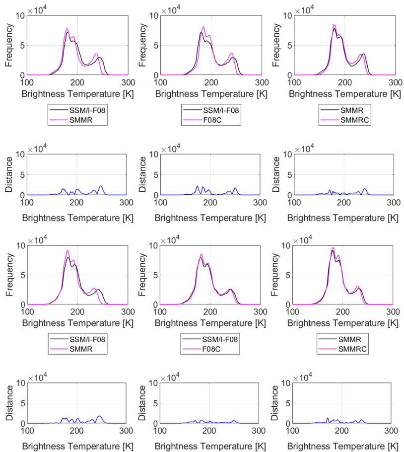
Figure 4: Brightness temperature histograms Histograms of T_b before and after the application of the intercalibration relations, Greenland. Relations are applied for both evening (a) and morning (b) passes, reporting the histograms of the data and the distance (absolute value of the difference as in Equation. (8)) between the histograms for original data. The first column represents the uncorrected data, the second the results applying the correction to SMMR data and the third the results applying the correction to the SSM/I data.
