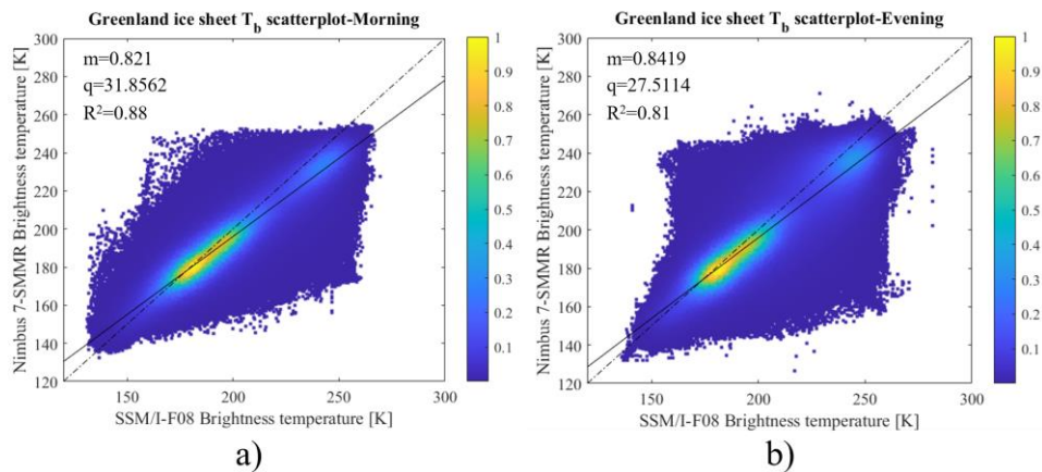
820 Figure 3 Density scatter plots of SMMR and SSM/I-F08 T_b brightness temperature data sensed during the overlap period (09/07/1987-20/08/1987) of the two sensors over the Greenland ice sheet for a) morning and b) evening passes. Solid black lines show the linear fitting and dashed black lines the 1:1 line. The colour palette indicates points density relative frequency.
