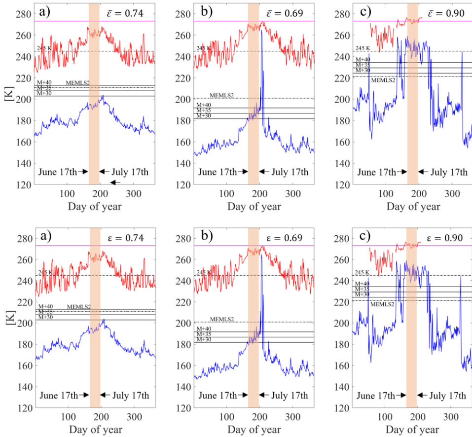
840 Figure 5: Timeseries of enhanced resolution T_b brightness-temperature 37 GHz H-pol (blue) and air temperature (red) at Summit (a), Humboldt (b) and Swiss Camp (c) stations, year 2005. Threshold values obtained with the different detection algorithms are also reported as horizontal black lines (solid M+\Delta T , dashed 245K and dash-dot MEMLS) while the 0^\circ\text{C} threshold is reported as magenta solid line. The 30 days window between 17 June and 17 July is shown in the shaded orange area, reporting the values of average estimated emissivity ( \epsilon ).
