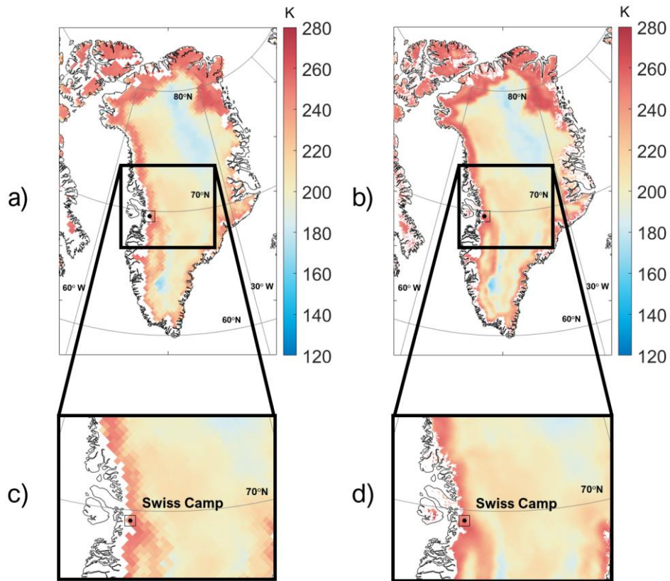
Figure 1: Maps of PMW passive-microwave T_b brightness temperature at 37 GHz, horizontal polarization, acquired over Greenland on 16 July 2001 in the case of the a) coarse ( 25 km ) and b) enhanced ( 3.125 km ) resolution products. Panels c) and d) refer to the area highlighted in the square in panels a) and b).
