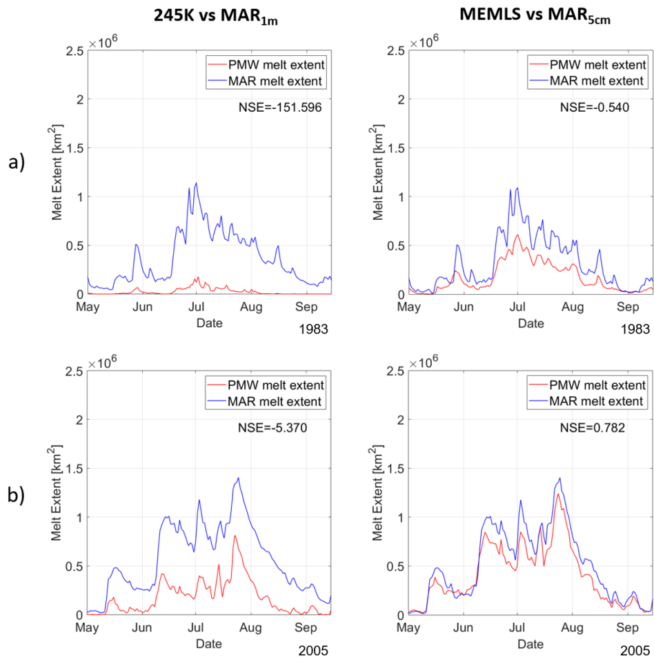
Figure 8: Melt extent estimation from PMW 37GHz H-pol T_b brightness temperature (red) and the regional climate model MAR (blue). Timeseries were obtained using the 245K algorithm and LWC average in the first 1 m of snowpack (left) and the MEMLS algorithm and LWC average in the first 5 cm of snowpack (right), for the years (a) 1983 and (b) 2005.
