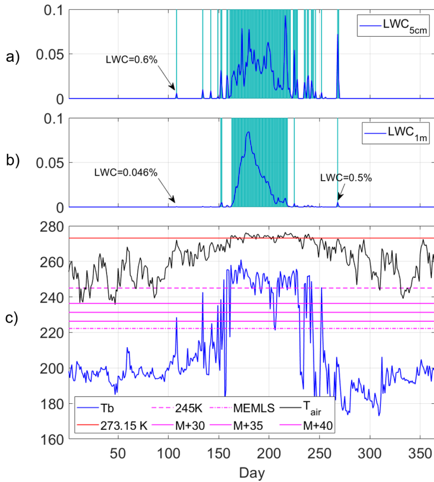
860 Figure 7: LWC from MAR averaged in the first 5 cm (a) and first 1 m (b) of the snowpack, (c) time series of 37 GHz horizontal polarization T_b (brightness temperature (3.125 km, blue), surface air temperature from AWS (black) and 245 K (dashed purple line), M+ \Delta T (solid purple lines) and MEMLS (dash-dotted purple line) thresholds for Swiss Camp site in 2001. Melting days according to MAR are marked as vertical light blue lines in panels (a) and (b).
