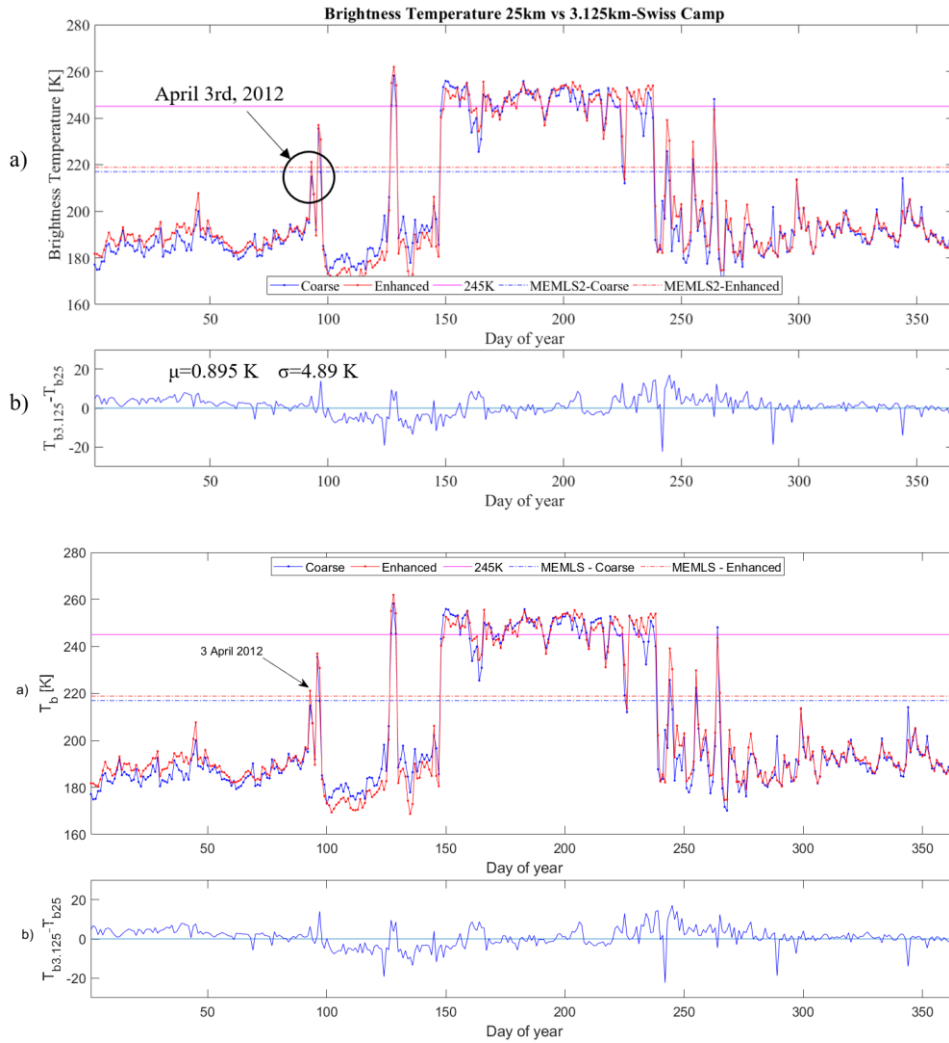
Figure 2 a) Time series of T_b brightness temperatures at 37 GHz, horizontal polarization, for the year 2012 of the pixel containing Swiss Camp site ( 69^{\circ}34'06'' N, 49^{\circ}18'57'' W,) in the case of the coarse (blue) and enhanced (red) products. Threshold values,
