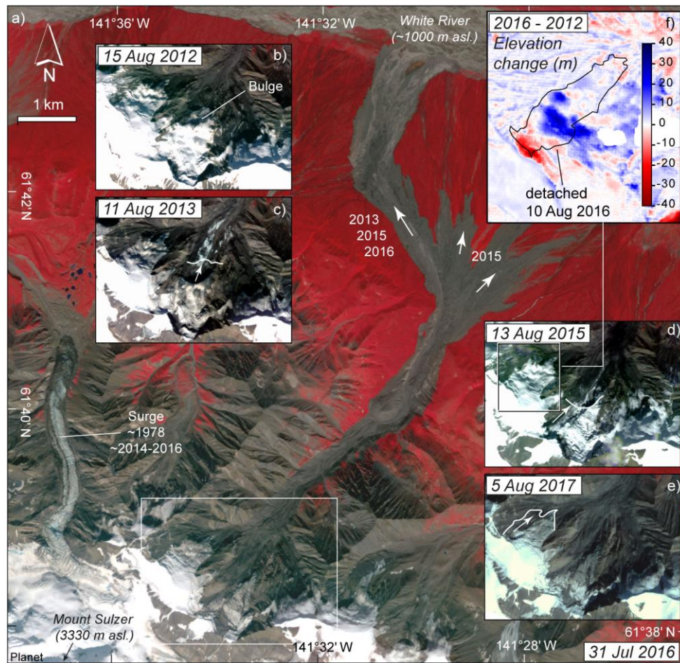
630 Figure 14: a) Overview of the three detachments and ice-rock avalanches from Flat Creek Glacier, Alaska, since 2012. 632 b) On the 15 Aug 2012 inset, a bulge is visible on the lower part of the glacier. c) On the 11 Aug 2013 inset, the glacier 634 part that detached on 5 Aug 2013 is indicated together with the front position before the event (white line). d) On the 636 13 Aug 2015 inset, the detachment of 31 Jul 2015 and the front position before it are indicated. e) On the 5 Aug 2017 inset, the area of the 10 Aug 2016 detachment is shown. All images © Planet (Dove and RapidEye satellites). (For more images and front positions see Jacquemart et al. (2020)). f) DEM difference between 13 Mar 2016 (Arctic DEM) and summer 2012 (Alaska IFSAR) showing surge-like mass redistribution (see also Supplement).
