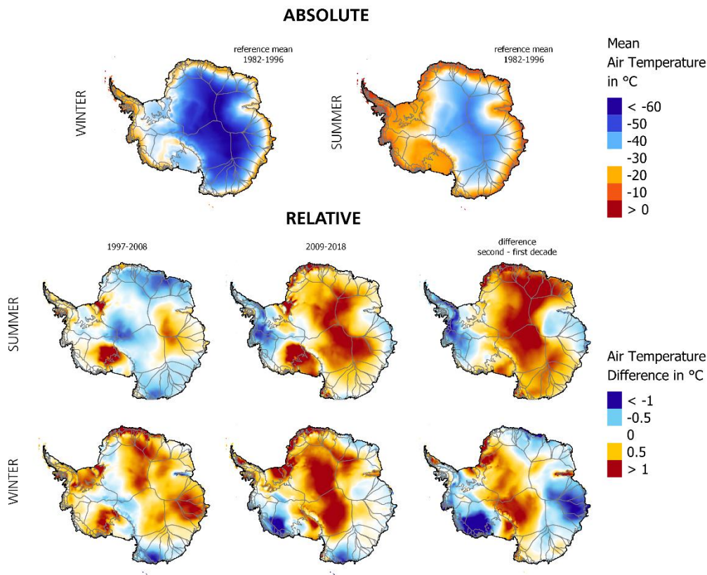
Figure 3 Absolute air temperature (1982-1996) and relative changes compared to the reference mean. Additionally, the difference between the first and second decade is illustrated.
