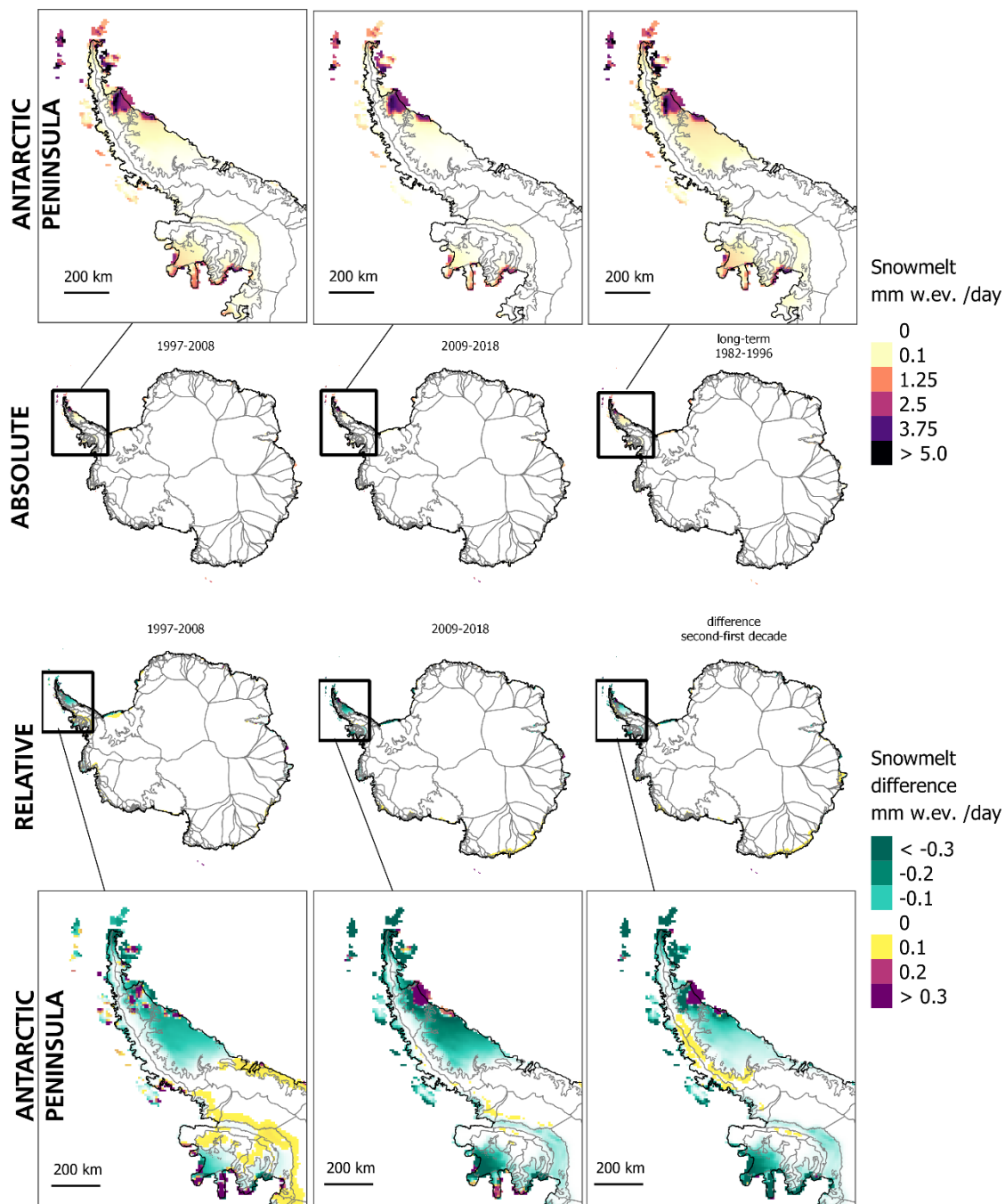
Figure 6 Mean snowmelt over Antarctica with enlarged views of the Antarctic Peninsula. Snowmelt is given in mm water equivalent per day.
