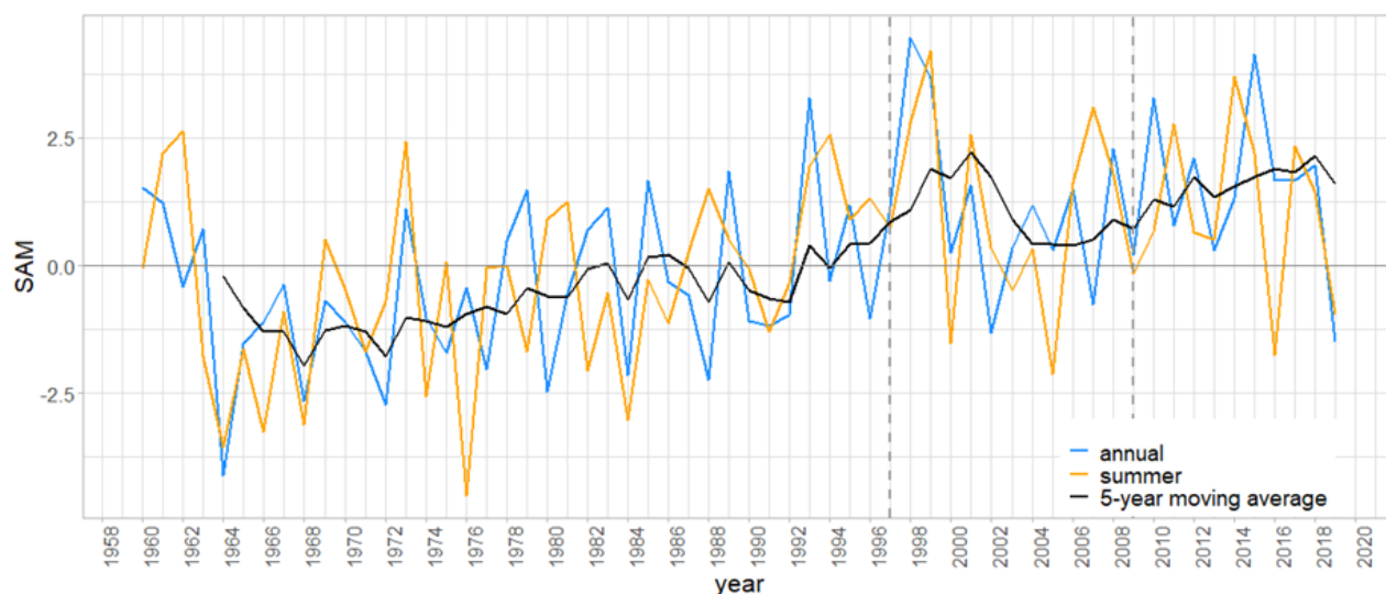
Figure 8 Southern Annular Mode (SAM) since 1960. Values are given for the annual SAM (blue), SAM during summer (orange) and a 5-year moving average for the annual SAM (black). The dashed grey lines indicate the investigated periods
