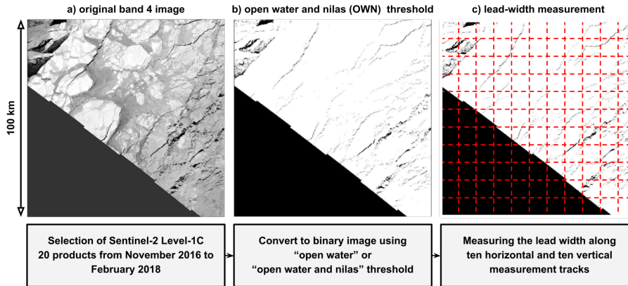
Figure 4. a) Exemplary original Sentinel-2 Level-1C band 4 image (sensing date: 16/03/2017). b) Binary image after the application of the open water and nilas (OWN) threshold, where leads are indicated with black pixels and no leads with white ones. c) Applied measurement grid with ten horizontal and vertical measurement tracks. The swath of the Sentinel-2 satellite does not cover the whole image area defined by the ESA data-processing grid. Thus, only the area covered by the satellite swath is considered for the lead-width measurement.
