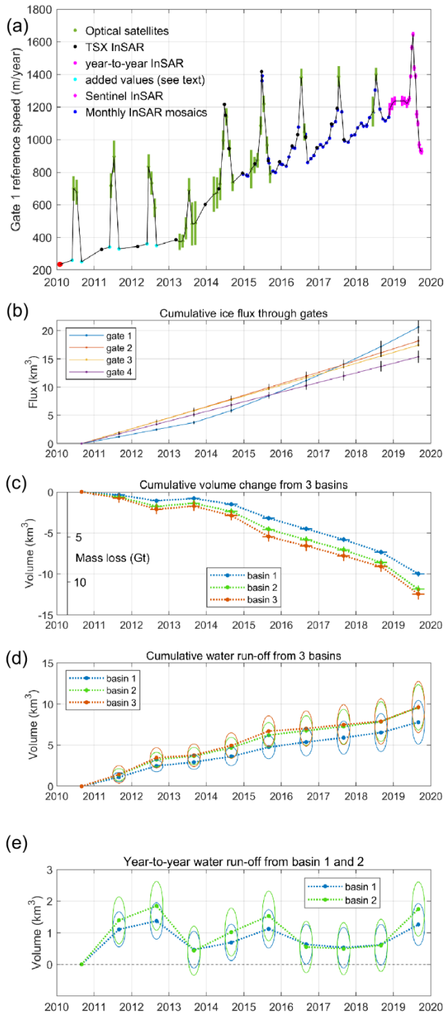
450 Figure 2: A: Temporal variation in surface speed at the reference point on gate 1. B: Cumulative year-to-year ice flux through the 4 gates. C: Cumulative volume of ice and mass lost by the three basins over the nine years. D: Cumulative water run-off from the three basins. The ellipses around each point are an indication of (vertically) the potentially uncertainty in the result and (horizontally) the time period of the CryoSat data used in estimating the volume change. E: Year-to-year variation in water run-off from basins 1 and 2. 455
