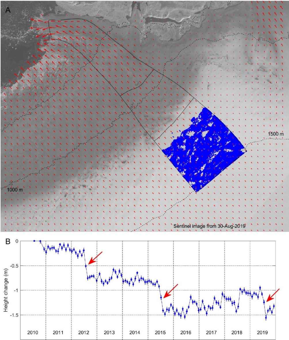
Figure 3. A: Part of the 30-Aug. 2019 Sentinel SAR image showing the positions (blue dots) of the 44,756 CryoSat POCA height estimates which were used in deriving the average 30-day temporal height change plot shown in B. The short vertical lines at each point are \pm 2 times the standard error of the mean of the height change estimates for each point and are an indication of the random error in the results. The three red arrows highlight the anomalous average summer height loss in 2012, 2015 and 2019 that has been ascribed to firn compaction due to warm temperatures at these elevations in these years.
